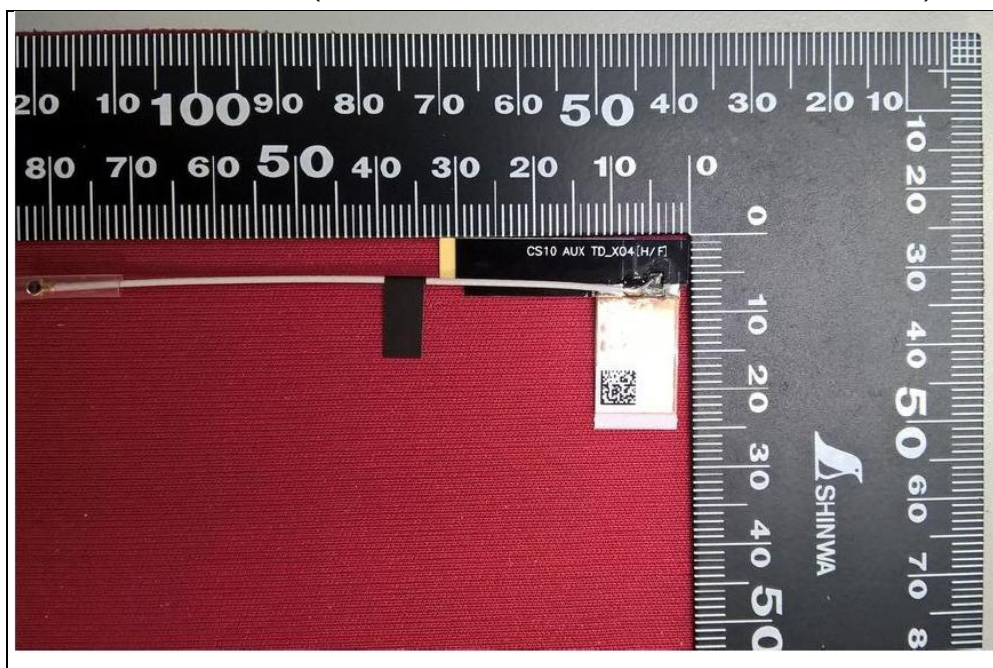
Antenna Set No.: 4 (Brand: TONGDA; Model: T-543-3010450-2 < Aux >)
