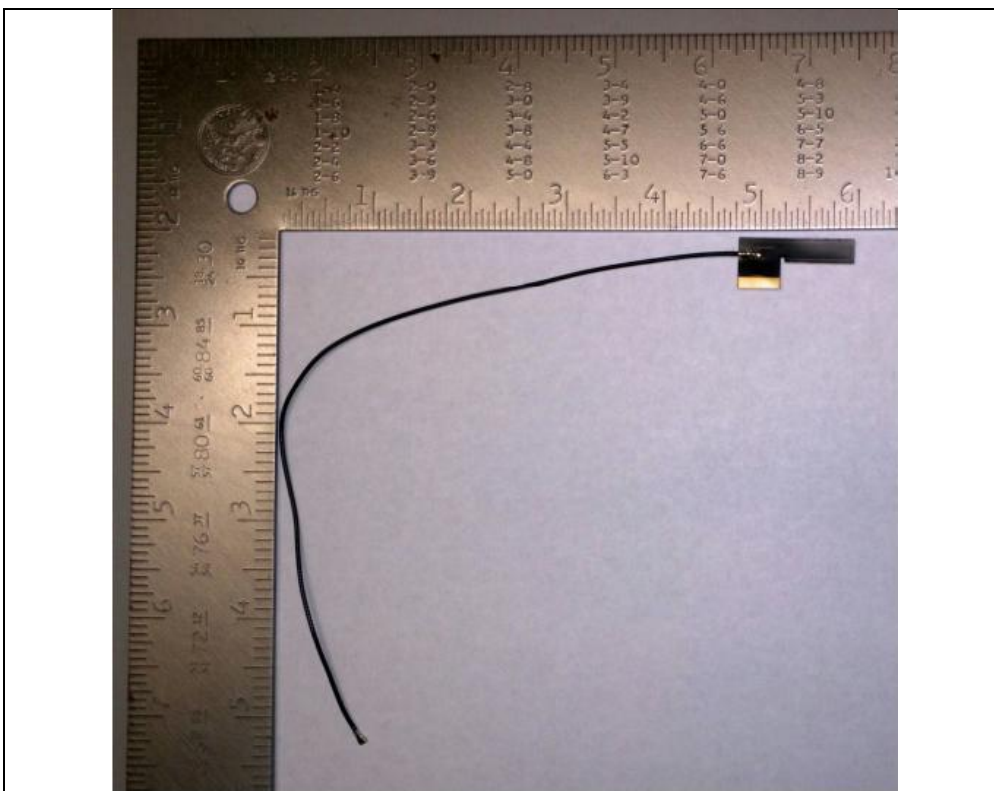
Antenna Set No.: 3 (Brand: Amphenol; Model: 867-00014 < Main >)
