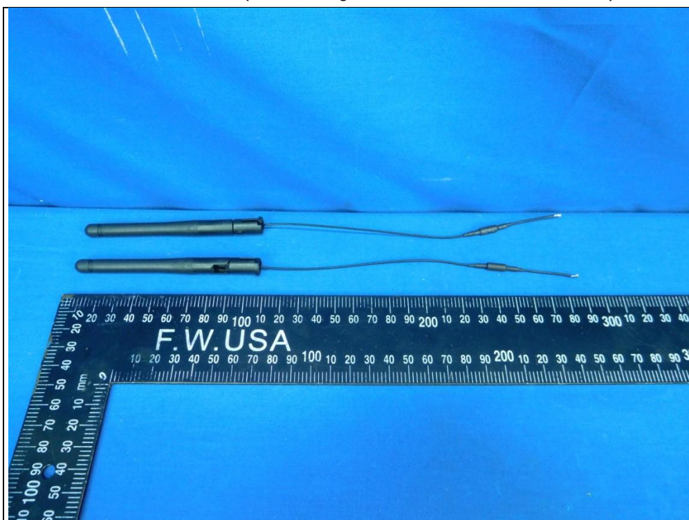
Antenna Set No.: 7 (Brand: Taoglas; Model: GW20.54.0180A.km)
