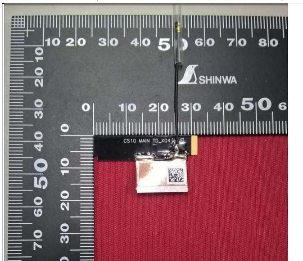
Antenna Set No.: 4 (Brand: TONGDA; Model: T-543-3010450-1 < Main >)
