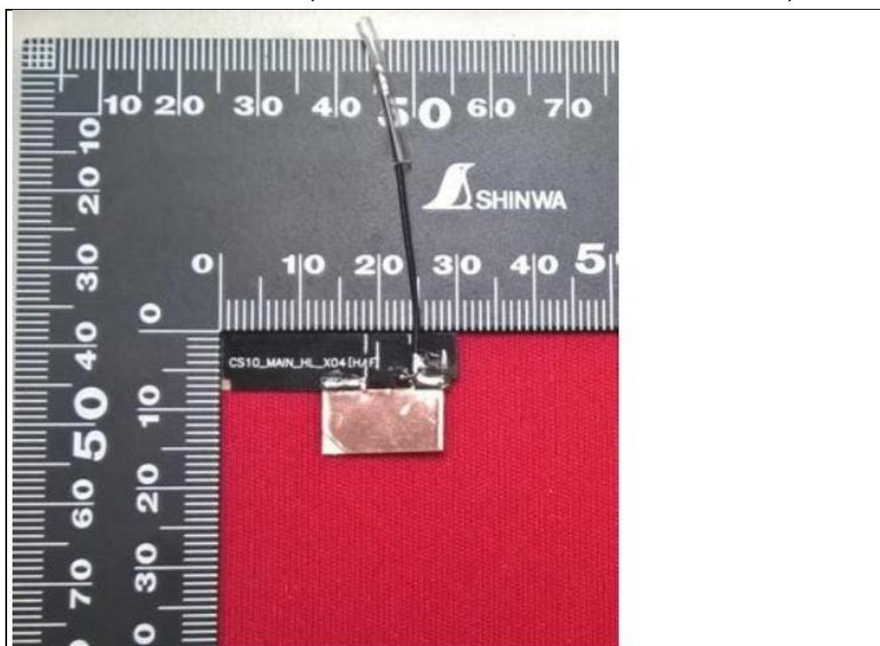
Antenna Set No.: 5 (Brand: HONGLIN; Model: 260-26079 < Main >)
