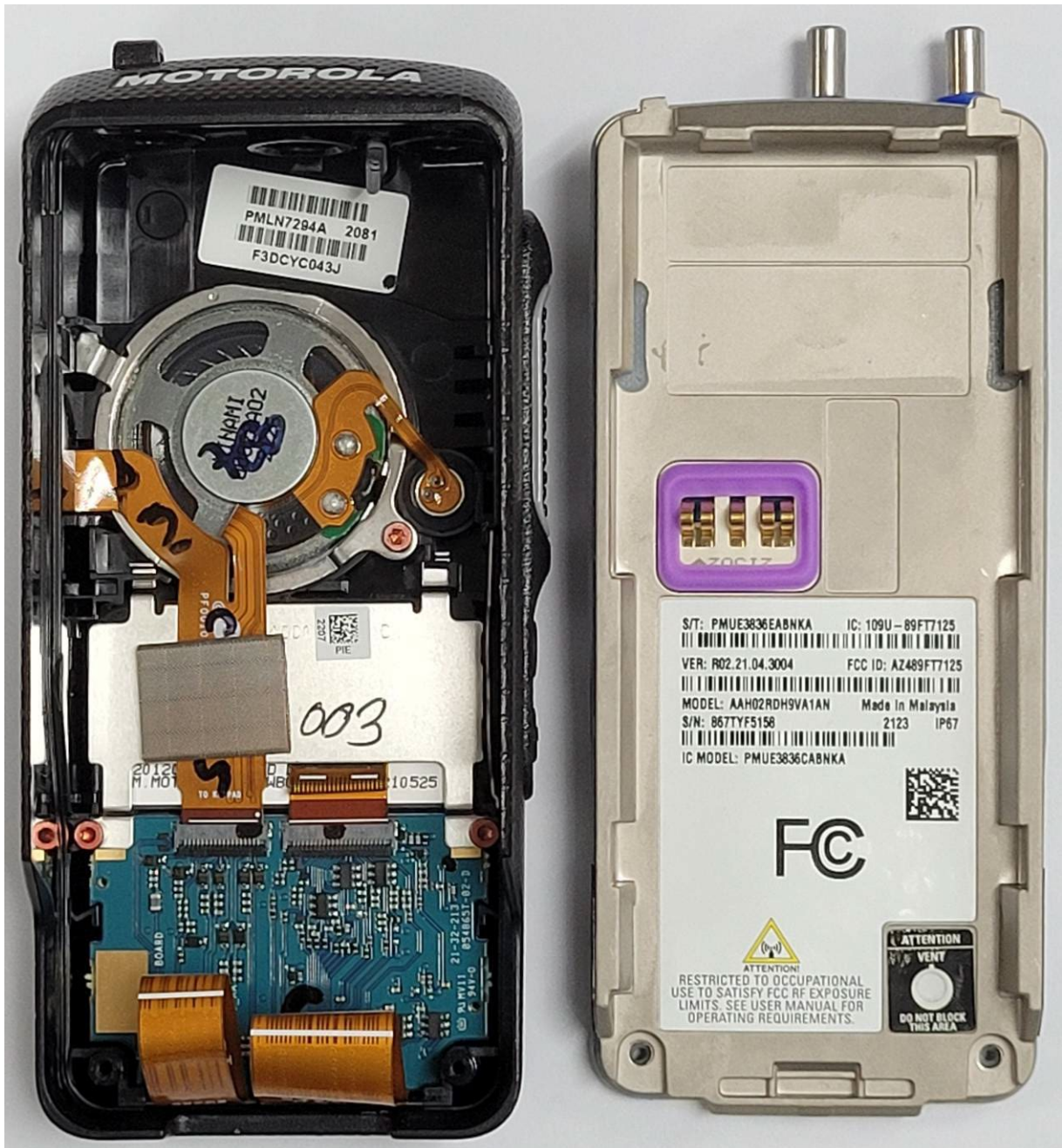
Chassis and Housing (back side) Non-TIA4950
