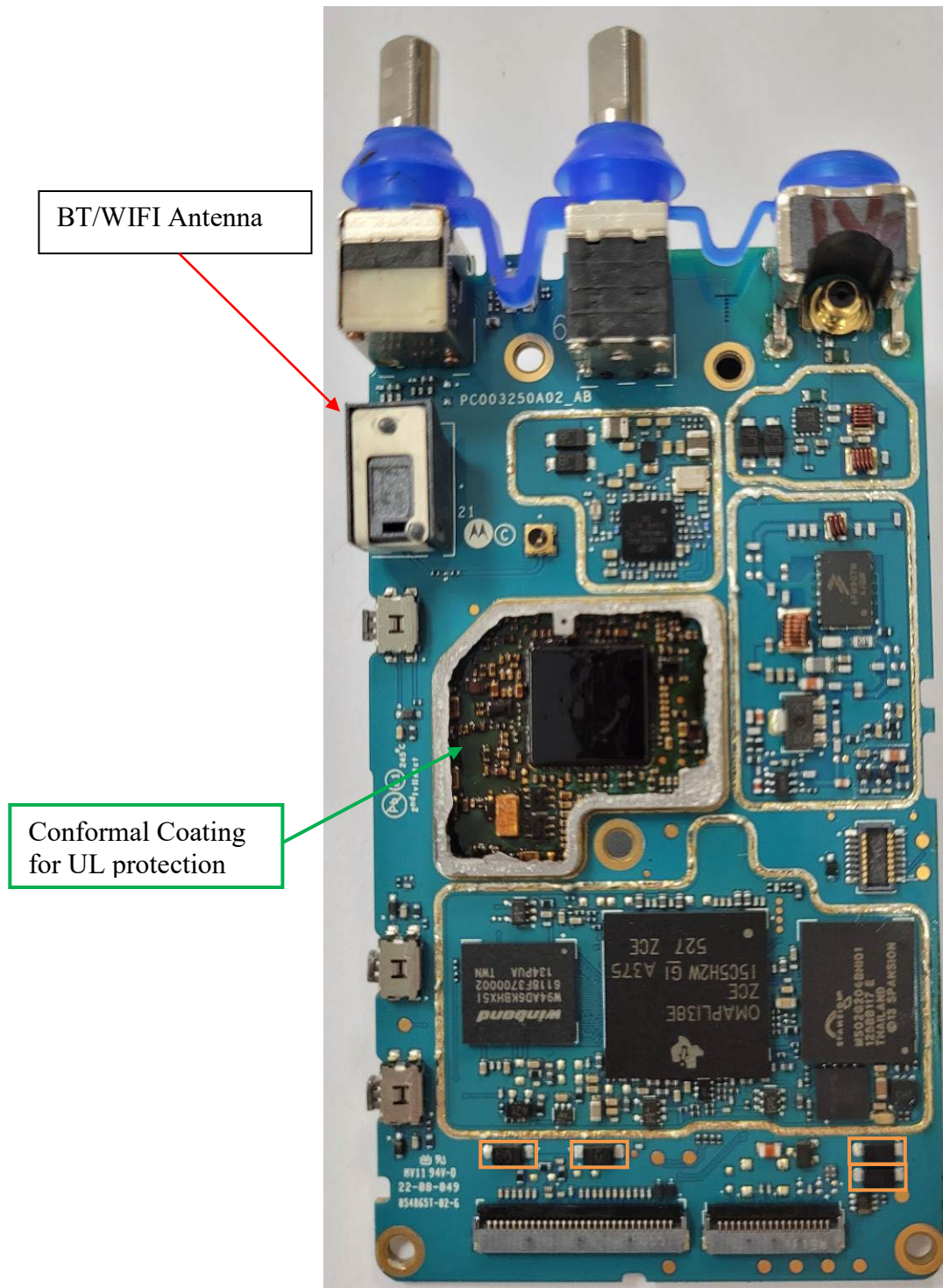
RF board without Shields (Top) TIA4950
