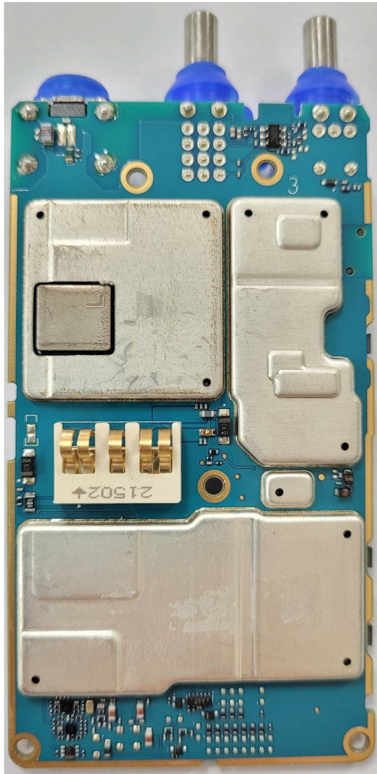
RF board with Shields (Bottom) TIA4950
