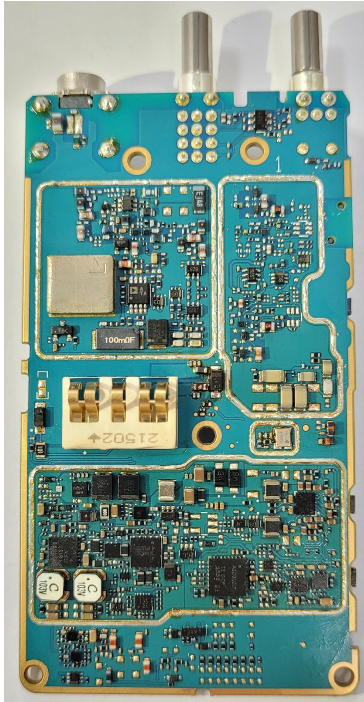
RF board without Shields (Bottom) Non-TIA4950
