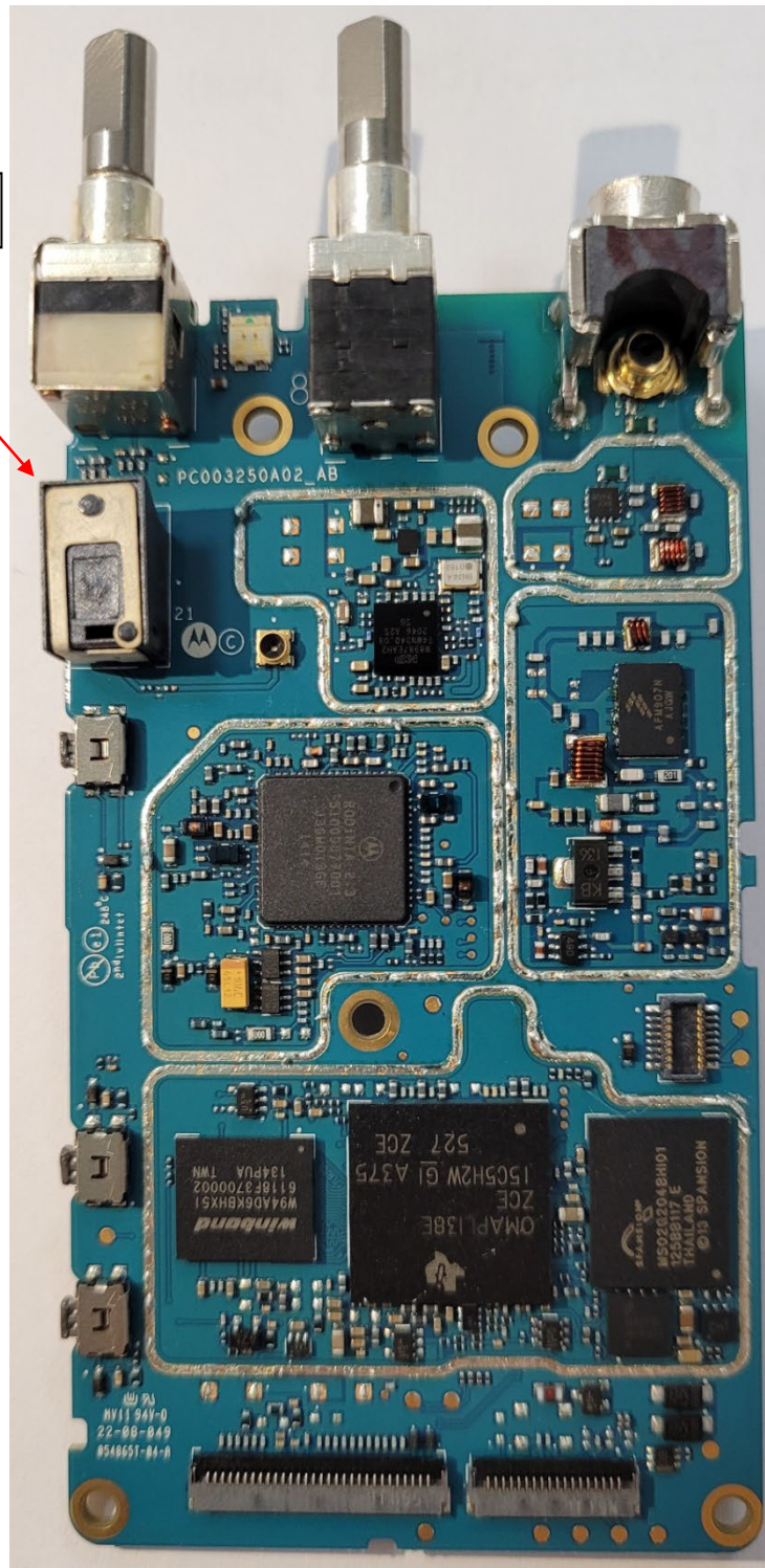
RF board without Shields (Top) Non-TIA4950
