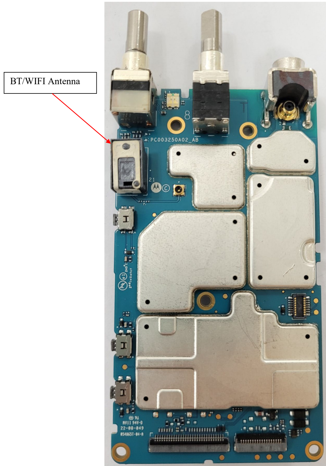
RF board with Shields (Top) Non-TIA4950
