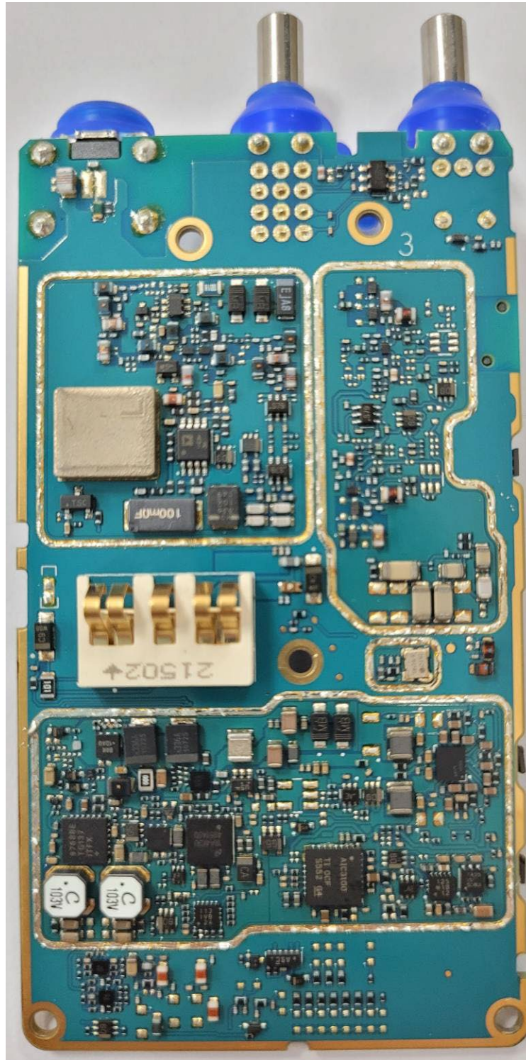
RF board without Shields (Bottom) TIA4950
