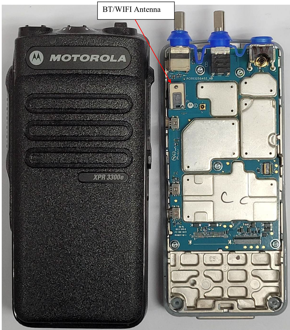
RF board with chassis and housing for Non Keypad model (front side) Non-TIA4950
