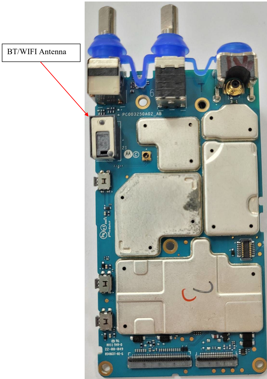
RF board with Shields (Top) TIA4950
