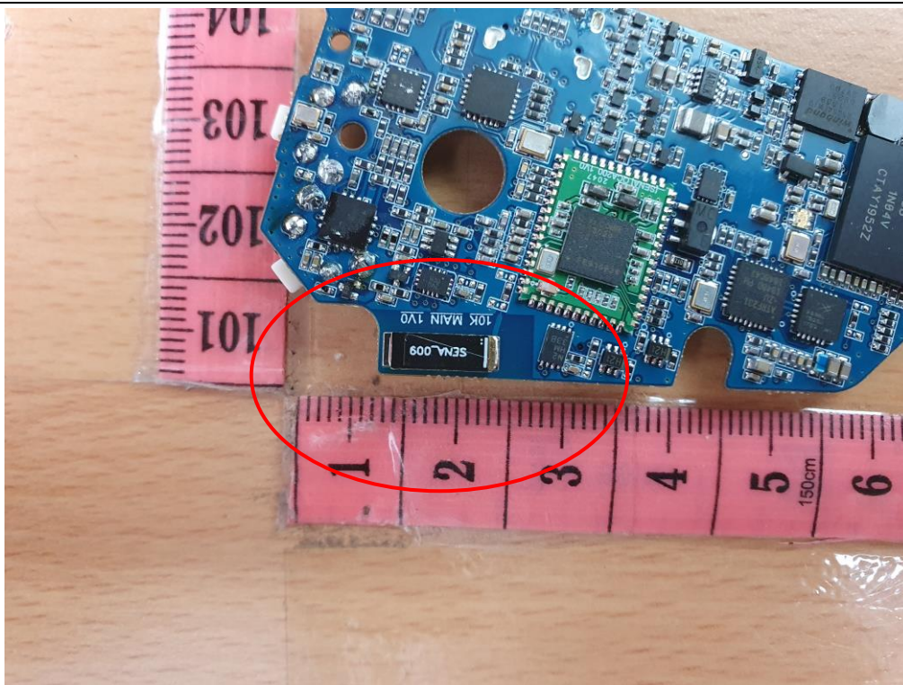
MESH Antenna
