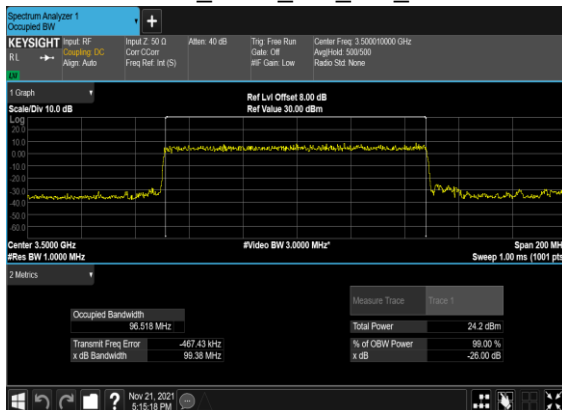
B5_N77(100M)_DFT-s-OFDM_PI_2- BPSK_Outer_Full_Mid_CH
