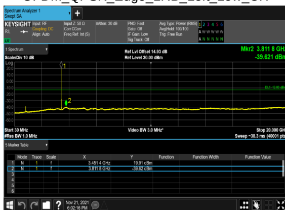
B5_N77(20M)_DFT-s- OFDM_QPSK_Edge_1RB_Left_Low_CH
