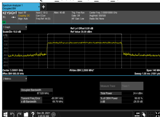
B5_N77(70M)_CP-OFDM_64 QAM_Outer_Full_Mid_CH
