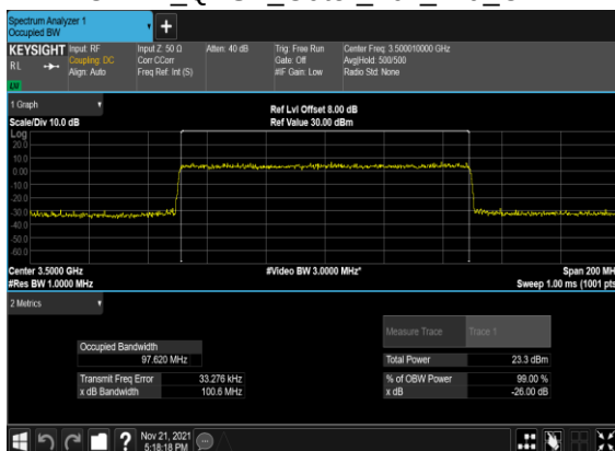
B5_N77(100M)_CP- OFDM_QPSK_Outer_Full_Mid_CH
