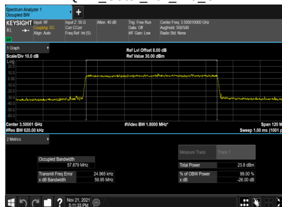
B5_N77(60M)_CP-OFDM_16 QAM_Outer_Full_Mid_CH
