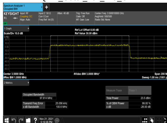
B5_N77(100M)_CP-OFDM_16 QAM_Outer_Full_Mid_CH
