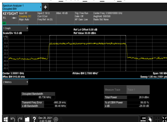
B5_N77(90M)_DFT-s-OFDM_PI_2- BPSK_Outer_Full_Mid_CH
