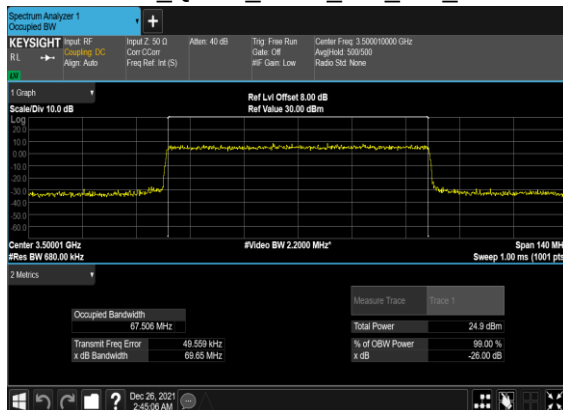
B5_N77(70M)_CP- OFDM_QPSK_Outer_Full_Mid_CH
