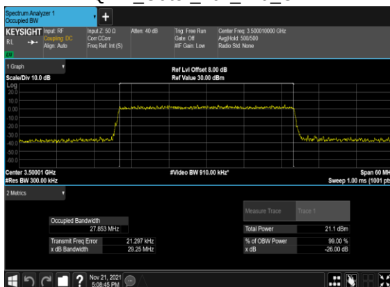
B5_N77(30M)_CP-OFDM_256 QAM_Outer_Full_Mid_CH
