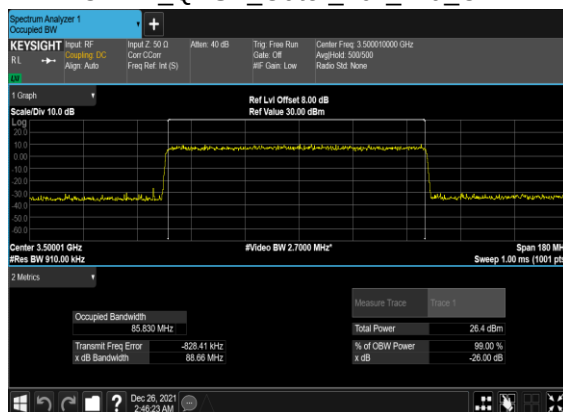
B5_N77(90M)_DFT-s- OFDM_QPSK_Outer_Full_Mid_CH
