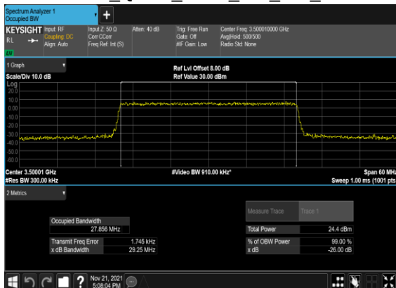
B5_N77(30M)_CP- OFDM_QPSK_Outer_Full_Mid_CH
