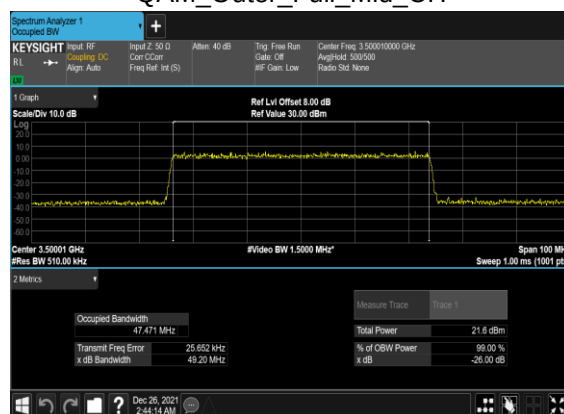
B5_N77(50M)_CP-OFDM_256 QAM_Outer_Full_Mid_CH
