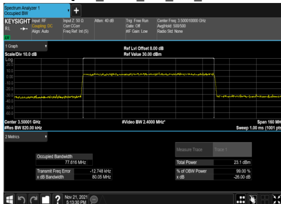
B5_N77(80M)_CP-OFDM_64 QAM_Outer_Full_Mid_CH
