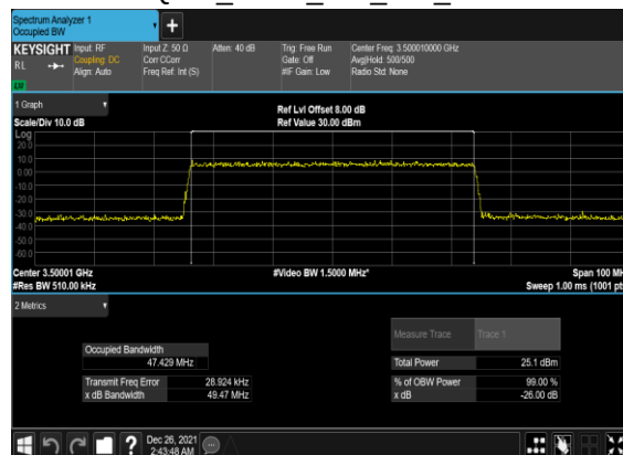
B5_N77(50M)_CP-OFDM_16 QAM_Outer_Full_Mid_CH
