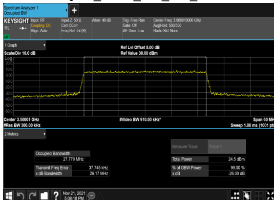
B5_N77(30M)_CP-OFDM_16 QAM_Outer_Full_Mid_CH
