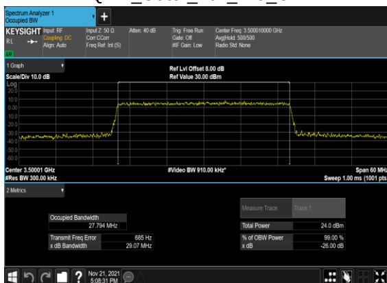
B5_N77(30M)_CP-OFDM_64 QAM_Outer_Full_Mid_CH
