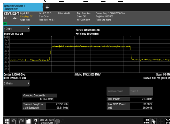
B5_N77(70M)_CP-OFDM_256 QAM_Outer_Full_Mid_CH
