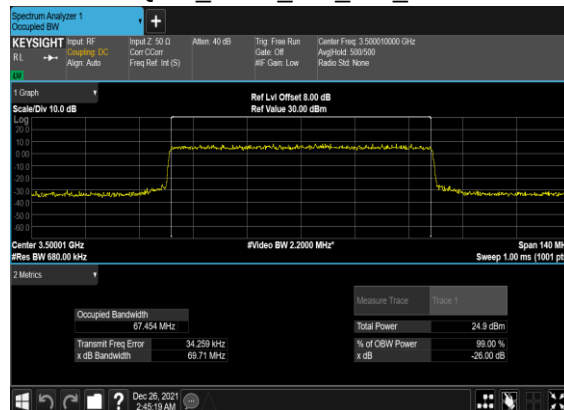
B5_N77(70M)_CP-OFDM_16 QAM_Outer_Full_Mid_CH
