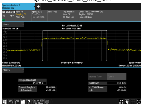
B5_N77(50M)_CP-OFDM_64 QAM_Outer_Full_Mid_CH
