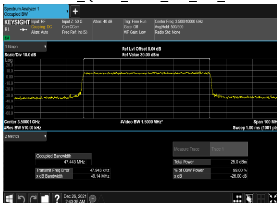
B5_N77(50M)_CP- OFDM_QPSK_Outer_Full_Mid_CH
