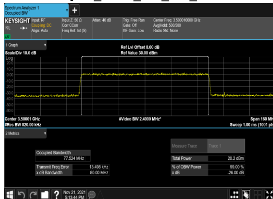
B5_N77(80M)_CP-OFDM_256 QAM_Outer_Full_Mid_CH
