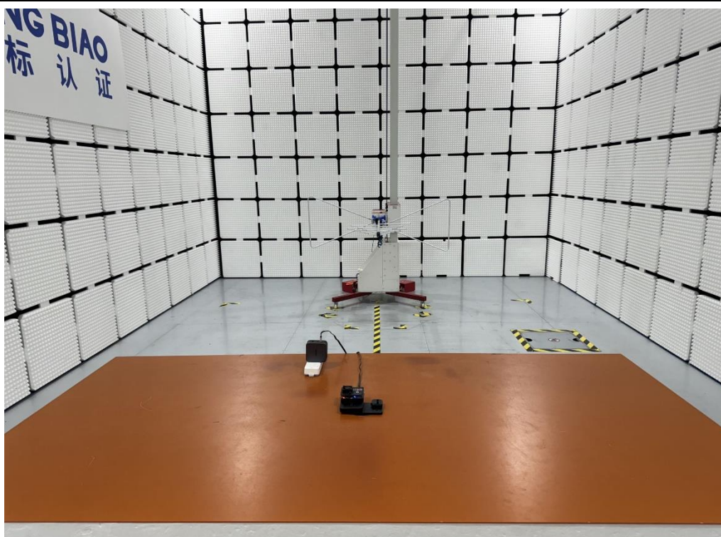
Radiated Emission Above 30MHz
