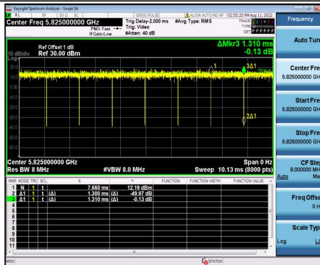
Keysight Spectrum Analyzer - Sweep SA Center Freq 5.825000000 GHz Trig Delay 2.000 ms #Avg Type: RMS Frequency
