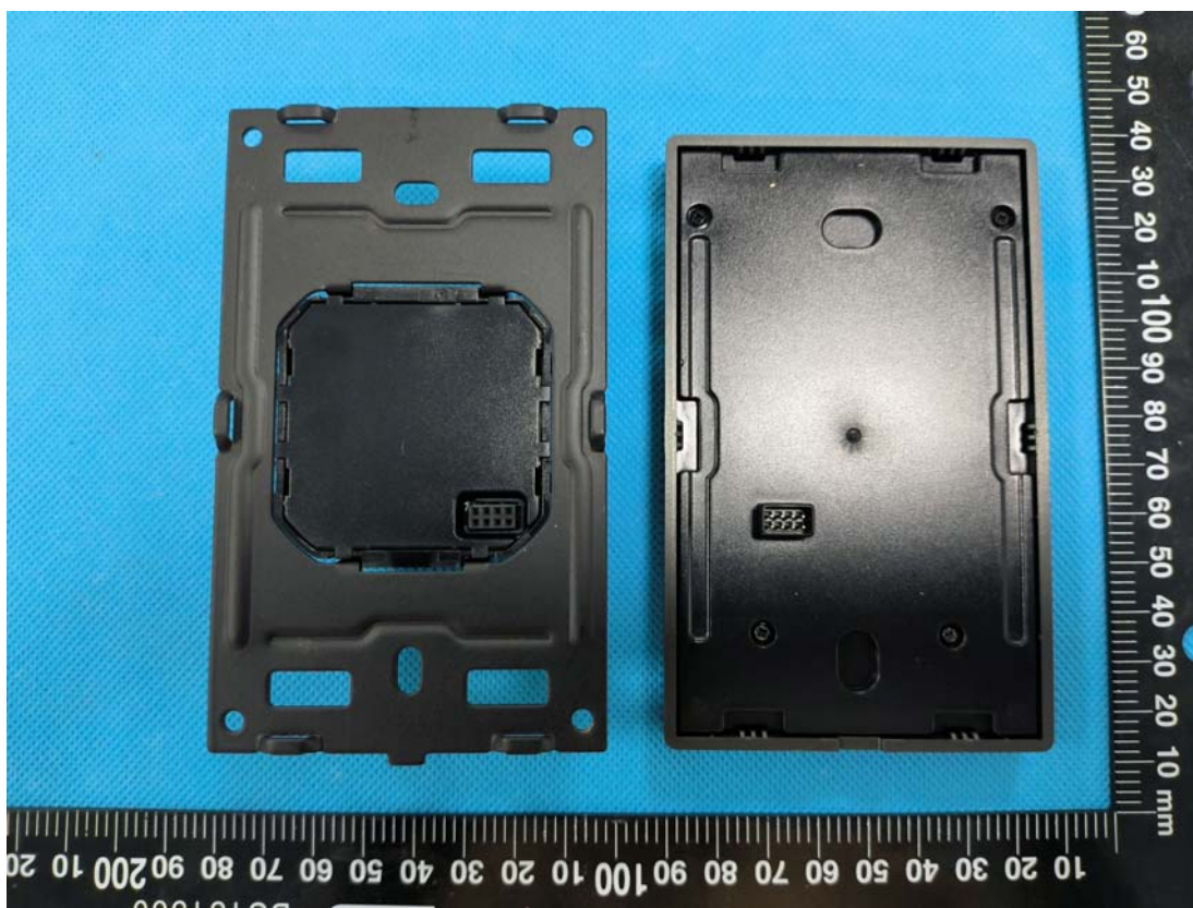
Model: M5-3C-120 With Relay 2#
