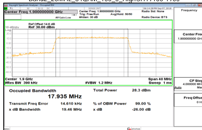
Band2_20MHz_64QAM_100_0_HighCH19100-1900
