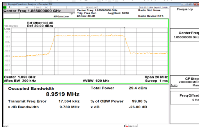
Band2_10MHz_16QAM_50_0_LowCH18650-1855
