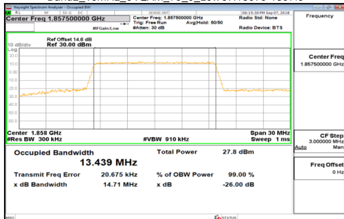
Band2_15MHz_64QAM_75_0_LowCH18675-1857.5
