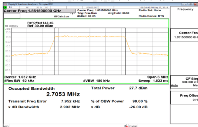
Band2_3MHz_64QAM_15_0_LowCH18615-1851.5
