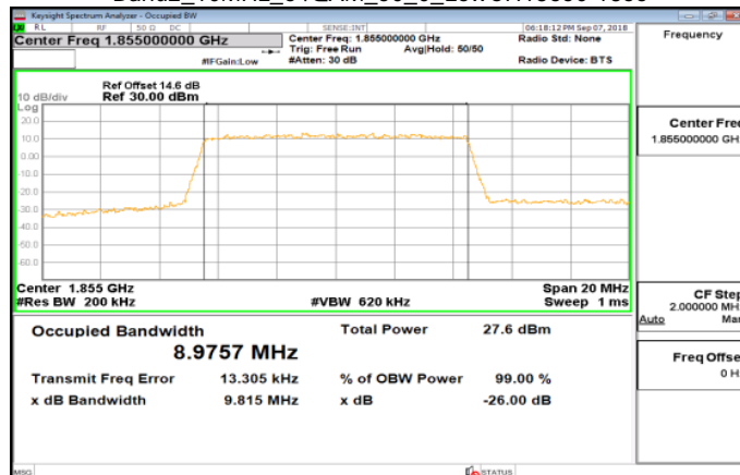
Band2_10MHz_64QAM_50_0_LowCH18650-1855
