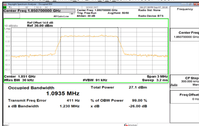
Band2_1_4MHz_64QAM_6_0_LowCH18607-1850.7
