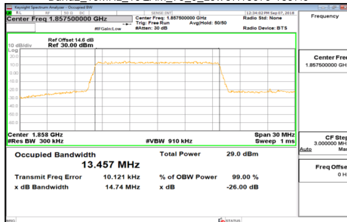
Band2_15MHz_16QAM_75_0_LowCH18675-1857.5
