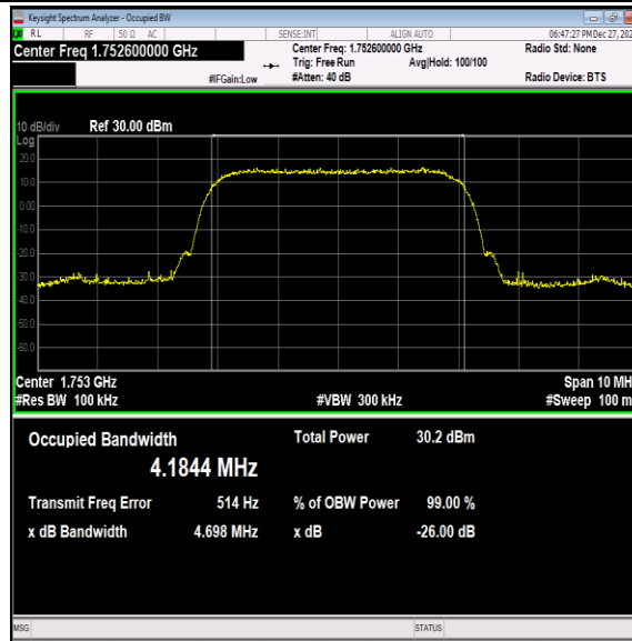
Band4-1513-2-PASS
