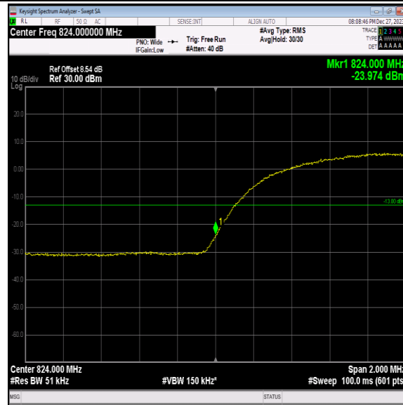
Band5-4132-1-PASS
