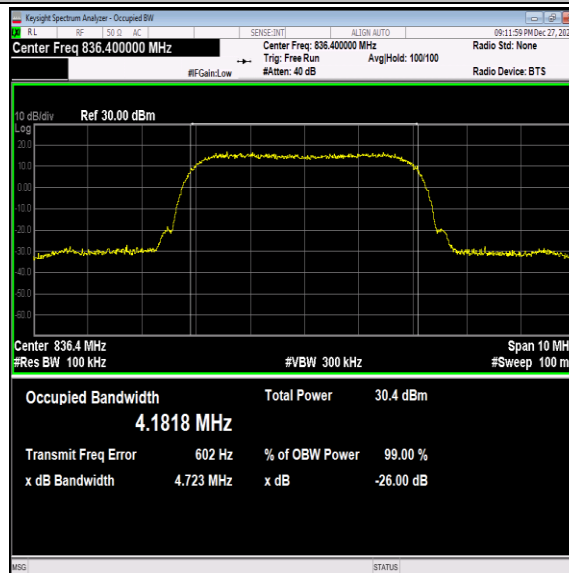
Band5-4182-1-PASS
