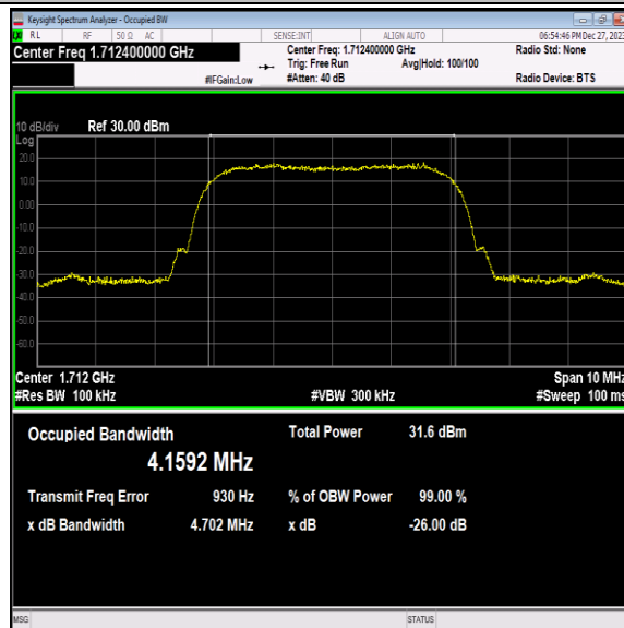
Band4-1312-5-PASS
