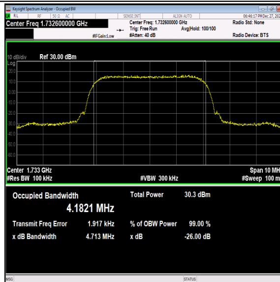
Band4-1413-2-PASS
