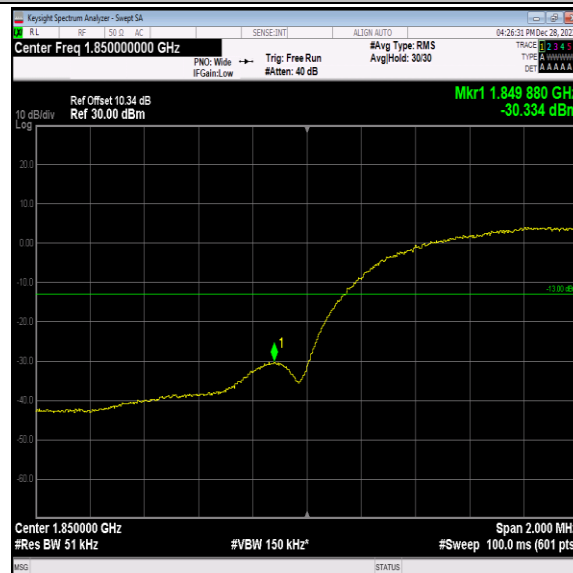
Band2-9262-2-PASS
