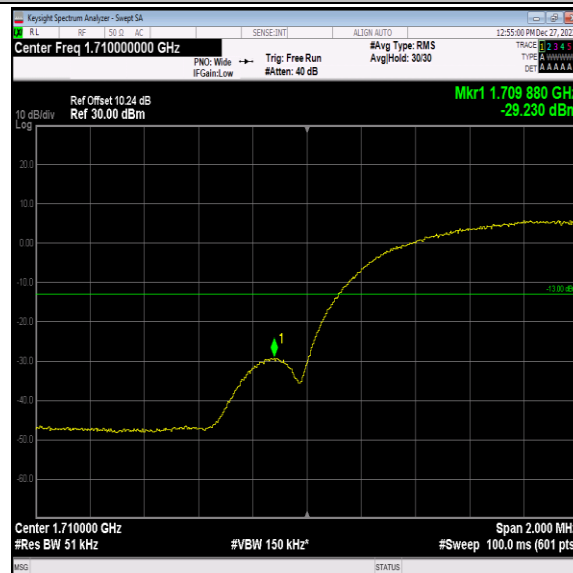
Band4-1312-2-PASS
