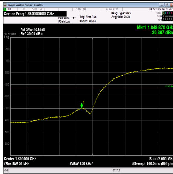
Band2-9262-3-PASS
