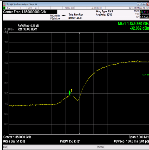
Band2-9262-4-PASS
