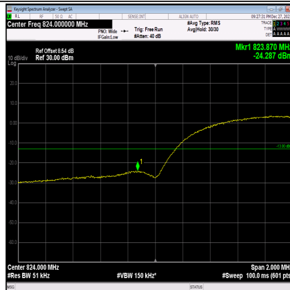
Band5-4132-2-PASS
