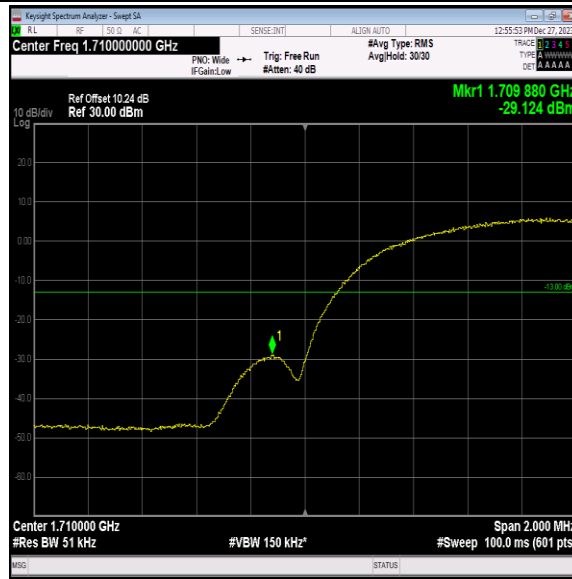
Band4-1312-3-PASS
