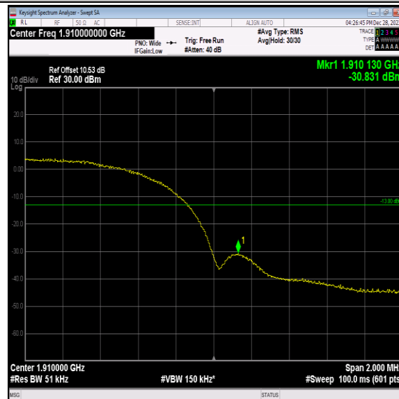
Band2-9538-2-PASS
