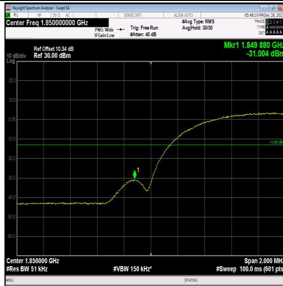
Band2-9262-5-PASS
