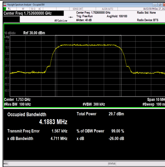
Band4-1513-4-PASS
