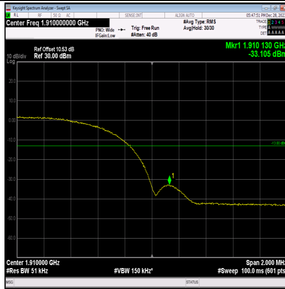
Band2-9538-4-PASS
