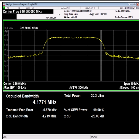
Band5-4233-2-PASS
