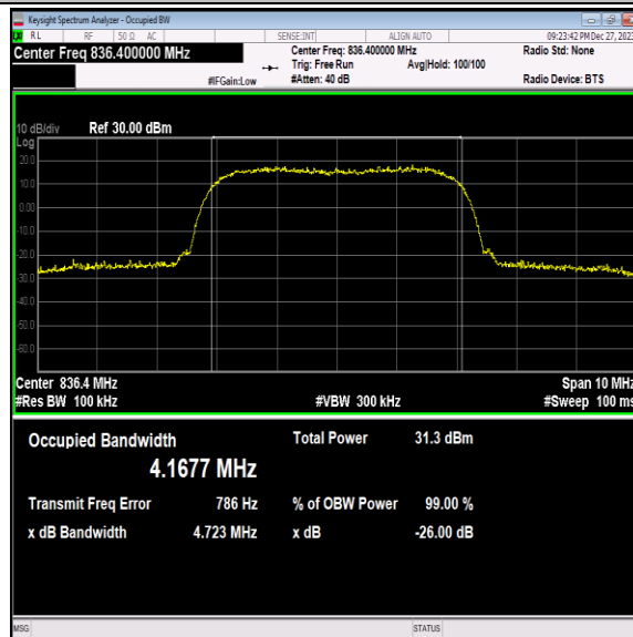
Band5-4182-5-PASS
