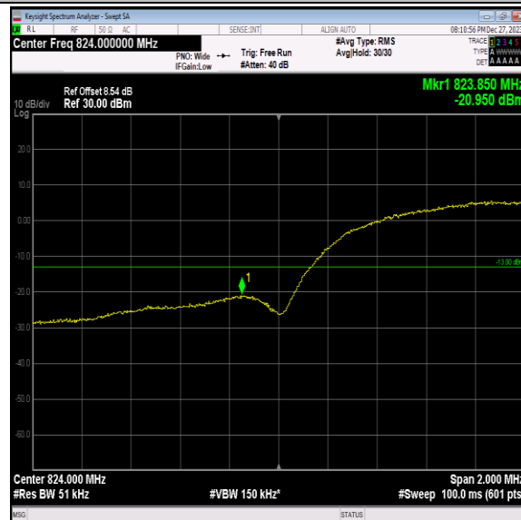
Band5-4132-4-PASS
