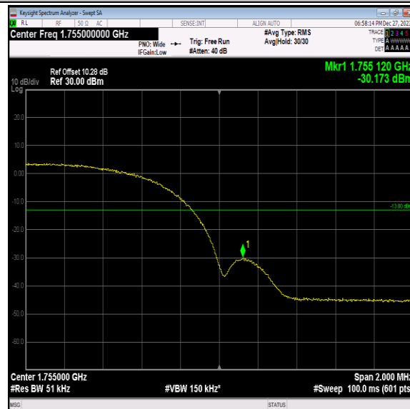
Band4-1513-1-PASS
