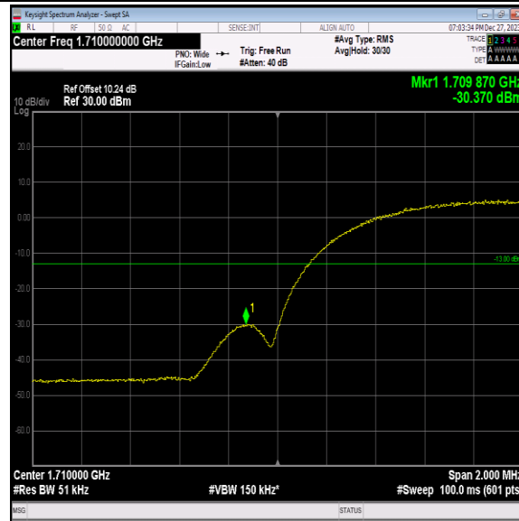
Band4-1312-5-PASS
