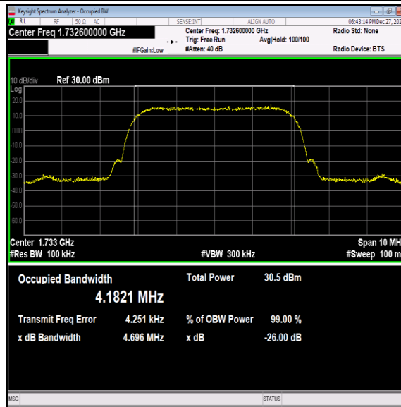
Band4-1413-1-PASS
