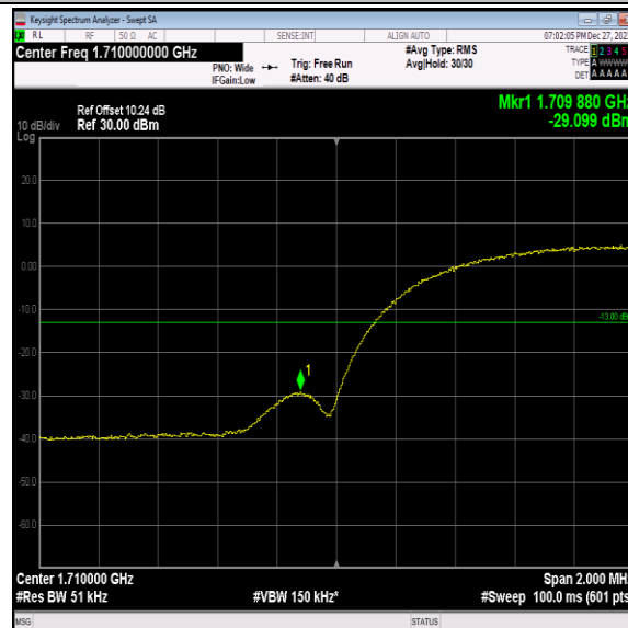
Band4-1312-4-PASS
