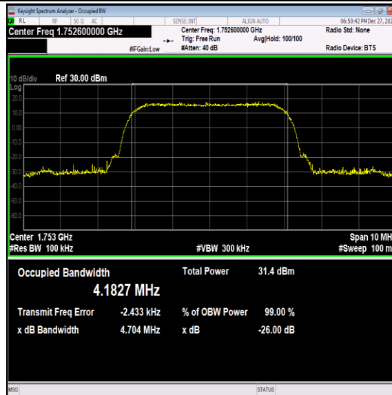
Band4-1513-3-PASS
