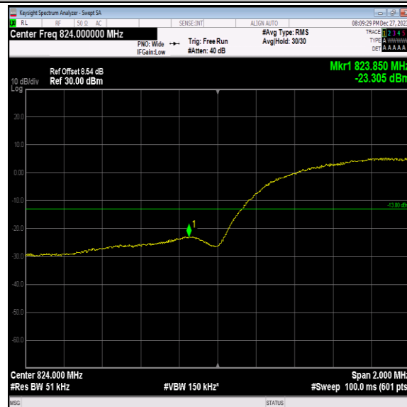
Band5-4132-2-PASS
