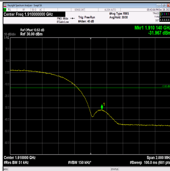
Band2-9538-1-PASS
