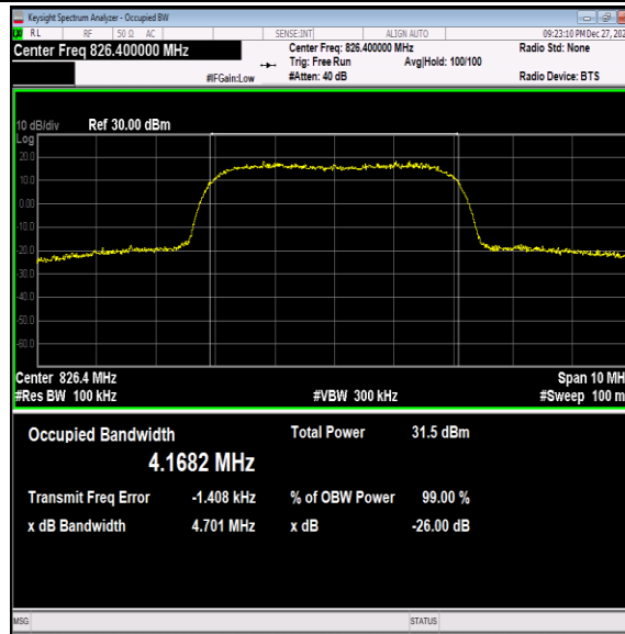
Band5-4132-5-PASS
