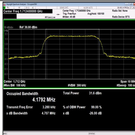
Band4-1312-3-PASS
