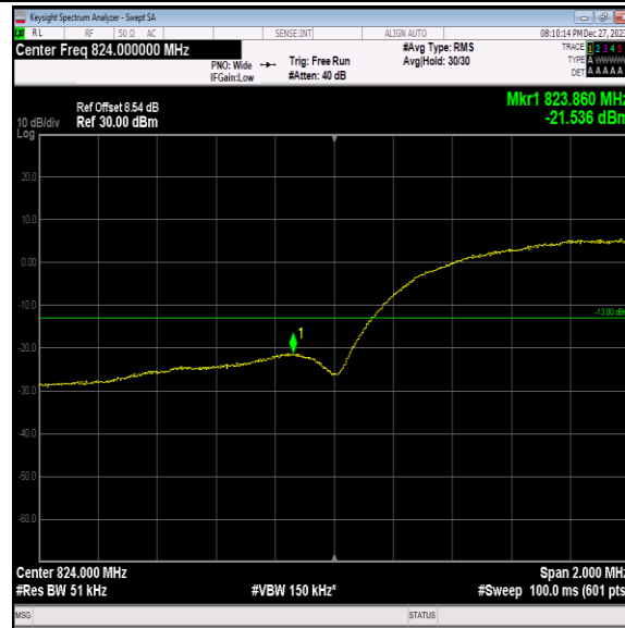
Band5-4132-3-PASS
