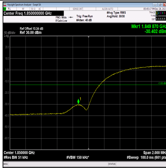
Band2-9262-3-PASS
