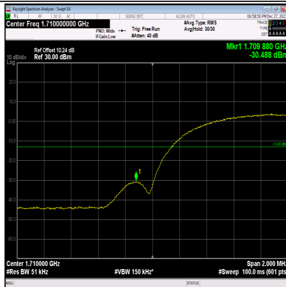
Band4-1312-2-PASS
