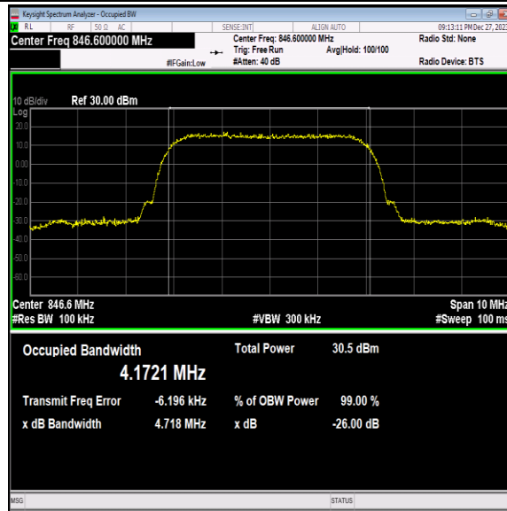
Band5-4233-1-PASS
