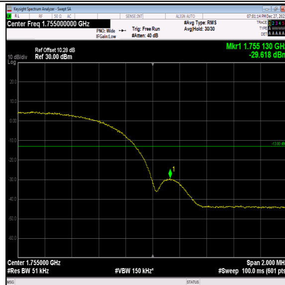
Band4-1513-3-PASS
