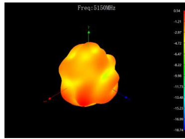
XYZ face @5150MHz
