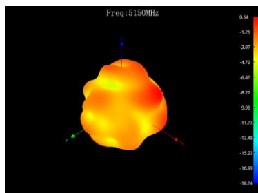
ZXY face @5150MHz
