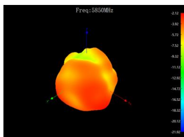
ZXY face @5850MHz
