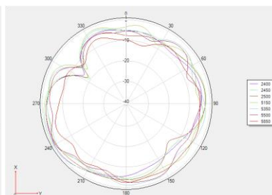
Theta =90
