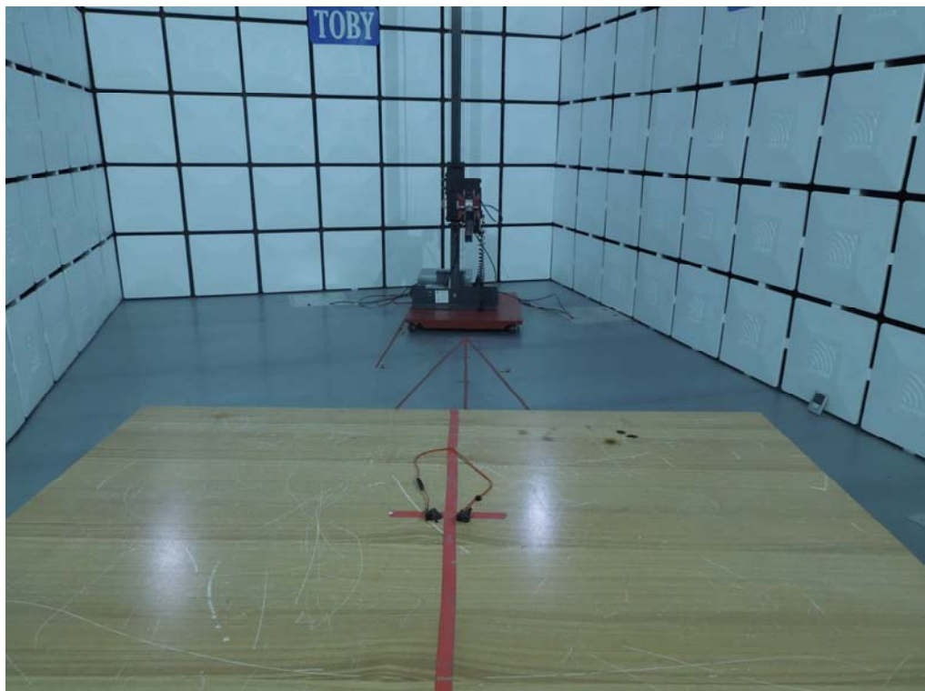
Radiation Test Setup (Above 1 GHz)
