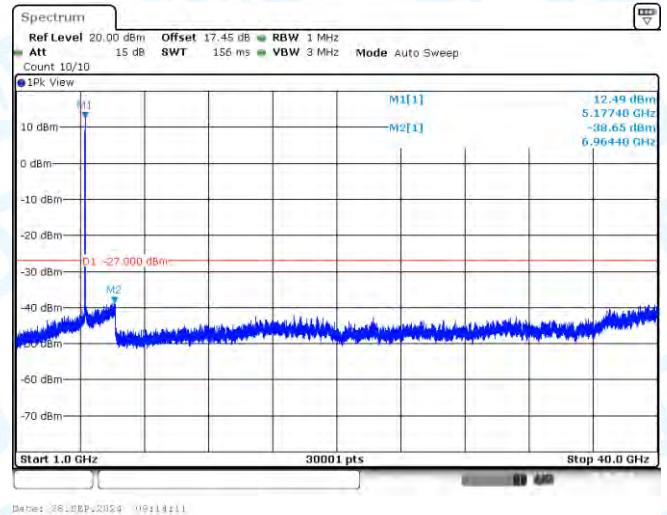
11N20-CDD-Ant1-5180-1000~40000-PASS
