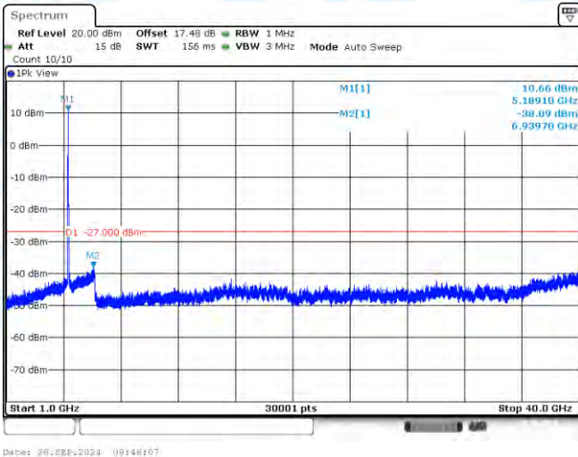
11N40-CDD-Ant2-5190-1000~40000-PASS
