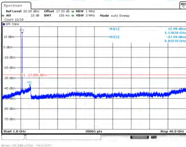
11N20-CDD-Ant2-5180-1000~40000-PASS
