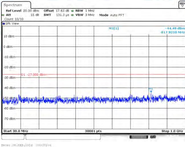
11N20-CDD-Ant3-5240-30~1000-PASS
