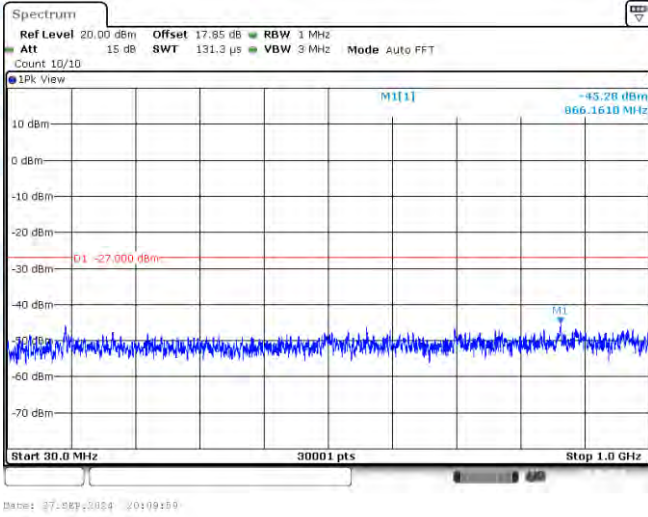
11A-CDD-Ant3-5745-30~1000-PASS
