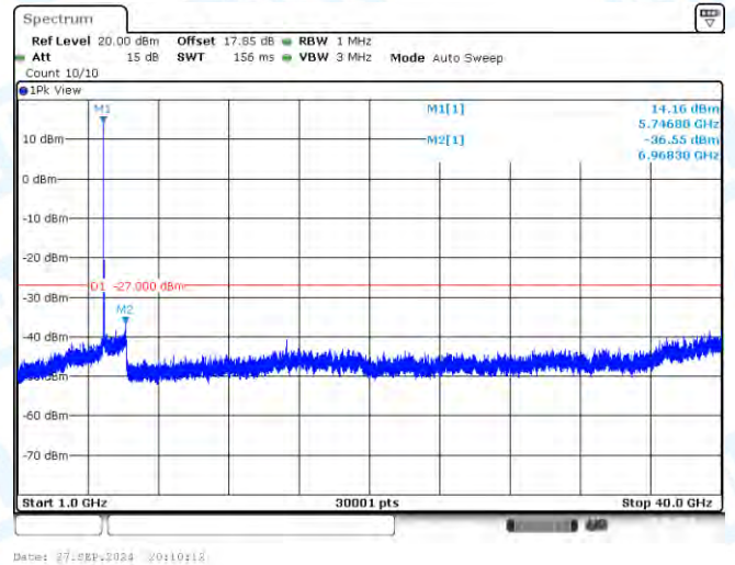
11A-CDD-Ant3-5745-1000~40000-PASS
