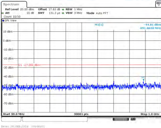
11A-CDD-Ant3-5240-30~1000-PASS
