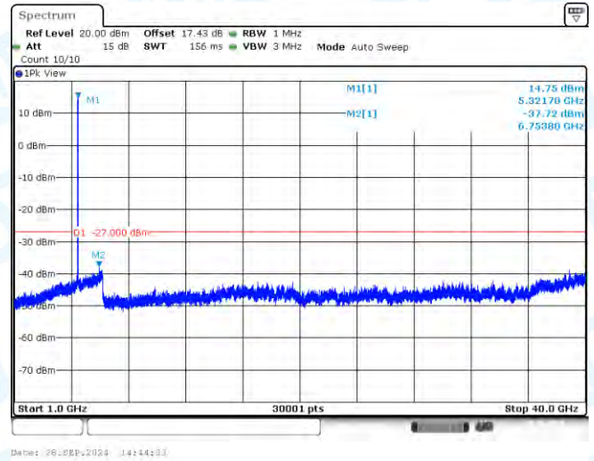
11A-Ant1-5320-1000~40000-PASS
