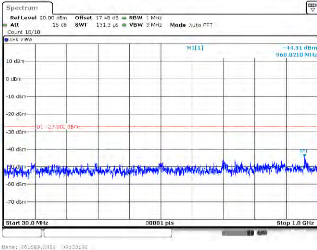
11N20-CDD-Ant1-5240-30~1000-PASS
