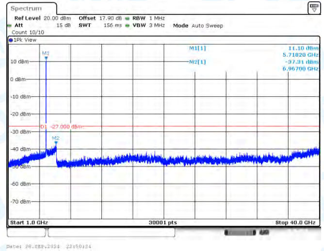
11A-CDD-Ant1-5720-1000~40000-PASS
