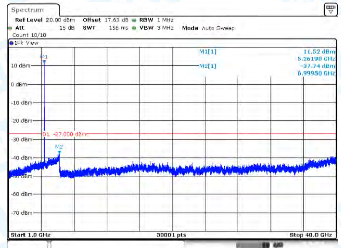
11A-CDD-Ant1-5260-1000~40000-PASS
