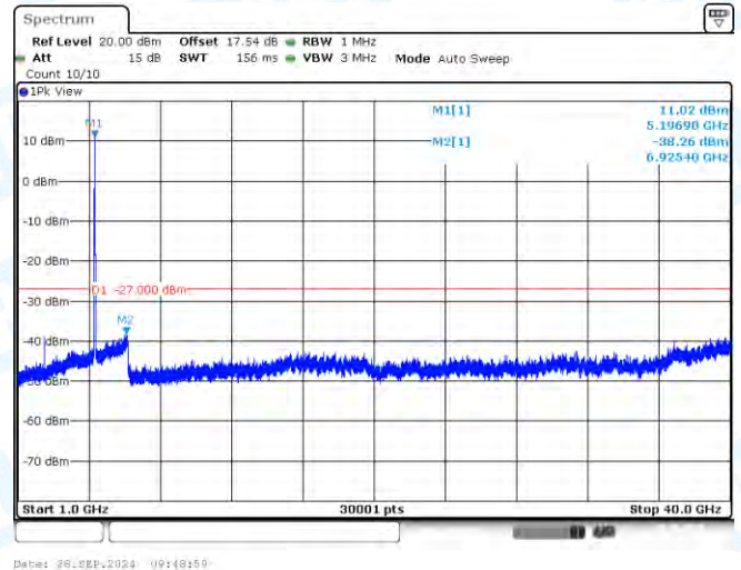
11N40-CDD-Ant3-5190-1000~40000-PASS
