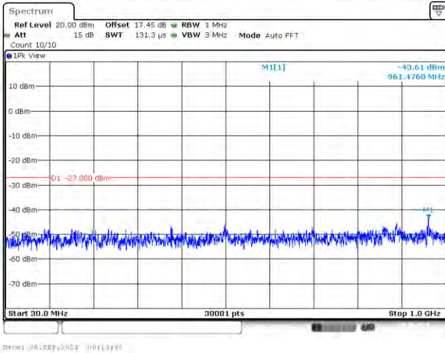
11N20-CDD-Ant1-5180-30~1000-PASS
