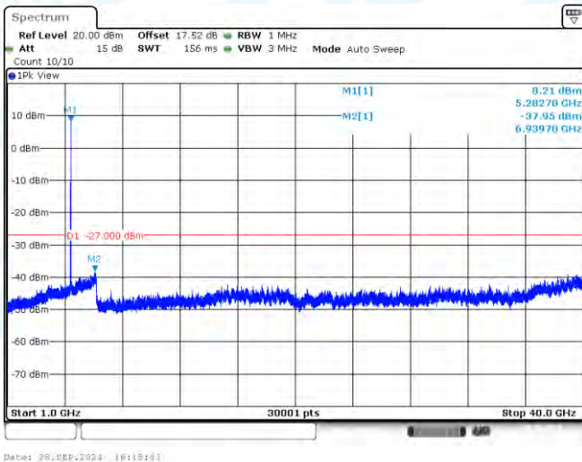
11A-CDD-Ant2-5280-1000~40000-PASS
