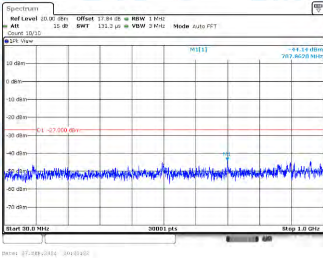
11A-CDD-Ant3-5785-30~1000-PASS
