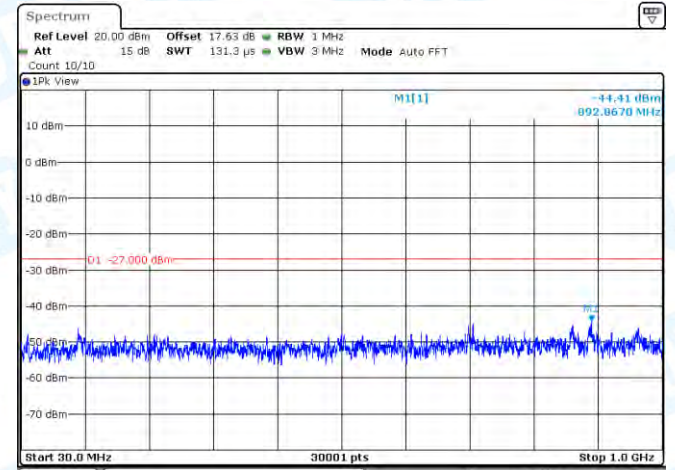
11A-CDD-Ant2-5580-30~1000-PASS
