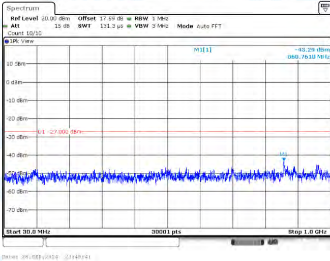
11N20-CDD-Ant1-5580-30~1000-PASS
