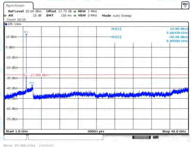
11N20-CDD-Ant3-5580-1000~40000-PASS
