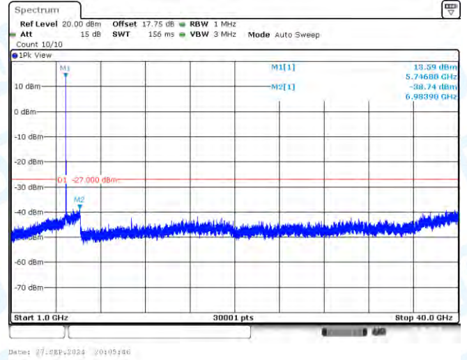
11A-CDD-Ant1-5745-1000~40000-PASS
