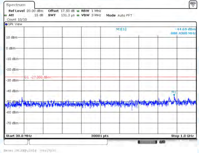
11N20-CDD-Ant2-5180-30~1000-PASS
