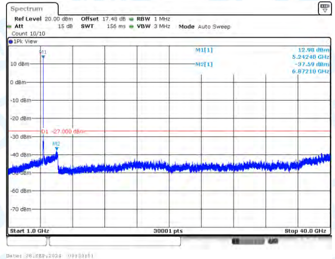
11N20-CDD-Ant1-5240-1000~40000-PASS
