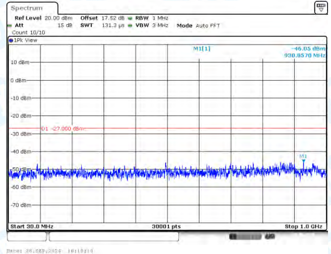
11A-CDD-Ant2-5280-30~1000-PASS
