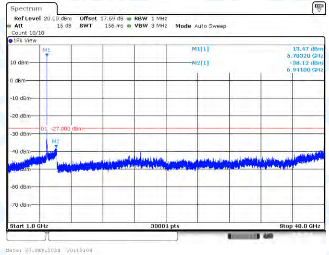
11A-CDD-Ant1-5785-1000~40000-PASS
