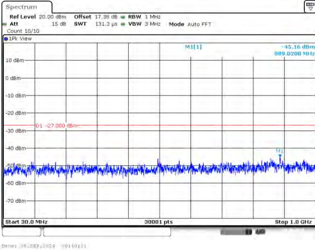
11N40-CDD-Ant1-5190-30~1000-PASS
