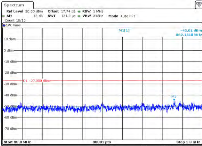
11A-Ant1-5825-30~1000-PASS
