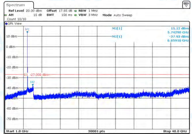
11N20-CDD-Ant1-5745-1000~40000-PASS
