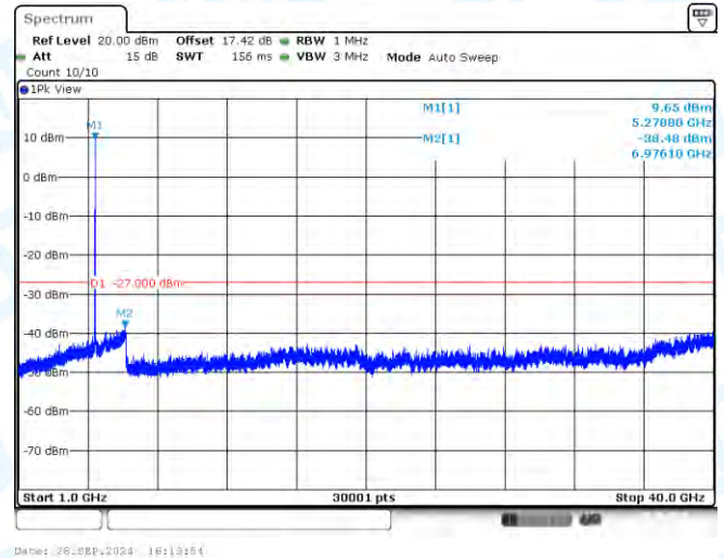
11A-CDD-Ant1-5280-1000~40000-PASS
