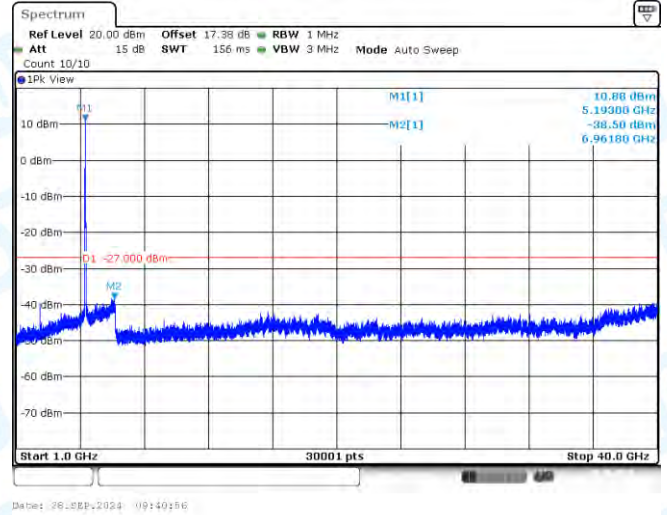
11N40-CDD-Ant1-5190-1000~40000-PASS
