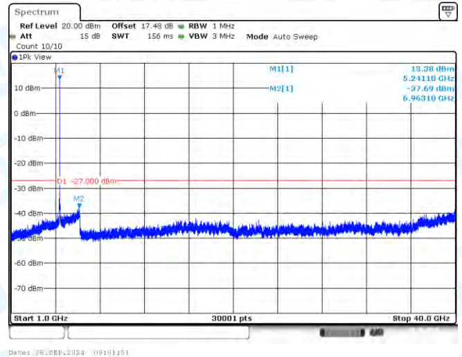
11A-CDD-Ant1-5240-1000~40000-PASS
