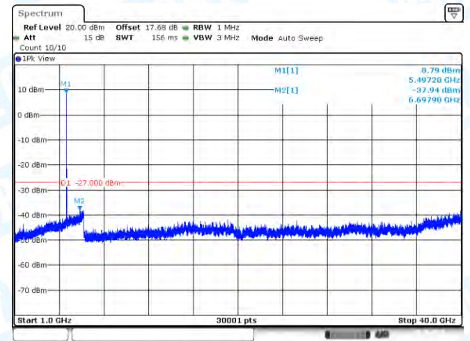
11N20-CDD-Ant1-5500-1000~40000-PASS
