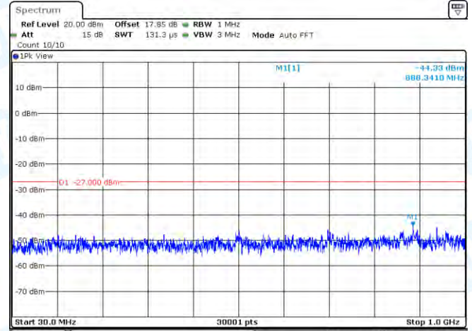
11N20-CDD-Ant2-5720-30~1000-PASS
