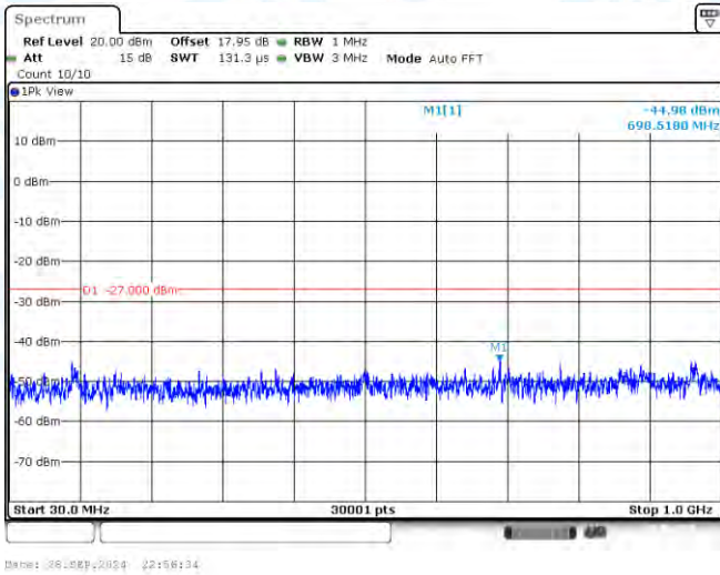
11A-CDD-Ant3-5720-30~1000-PASS
