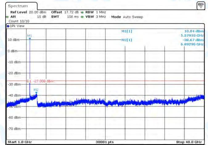
11A-CDD-Ant1-5580-1000~40000-PASS
