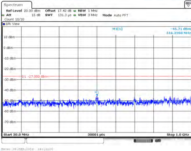
11A-CDD-Ant1-5280-30~1000-PASS
