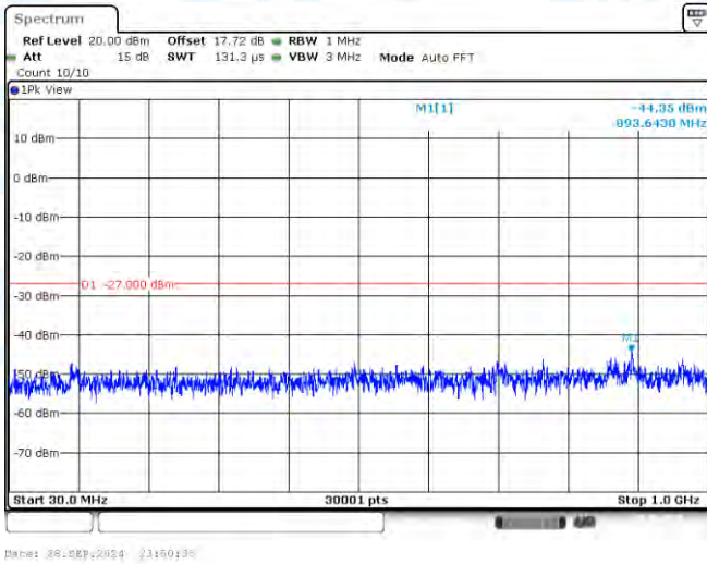
11N20-CDD-Ant3-5580-30~1000-PASS
