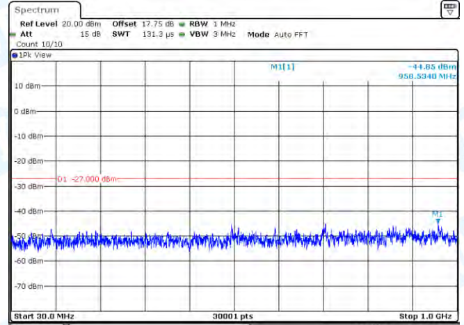
11A-Ant2-5745-30~1000-PASS
