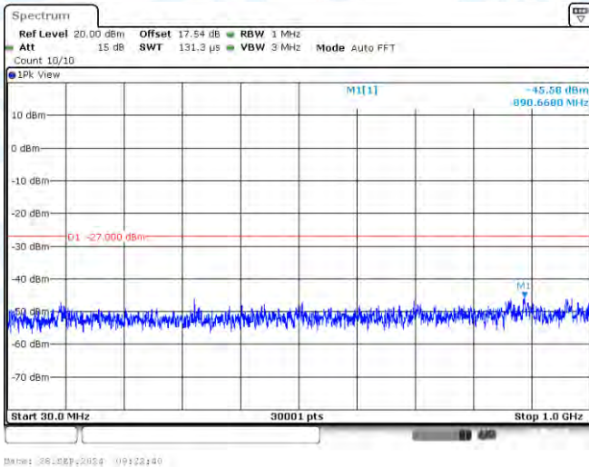
11N20-CDD-Ant3-5180-30~1000-PASS
