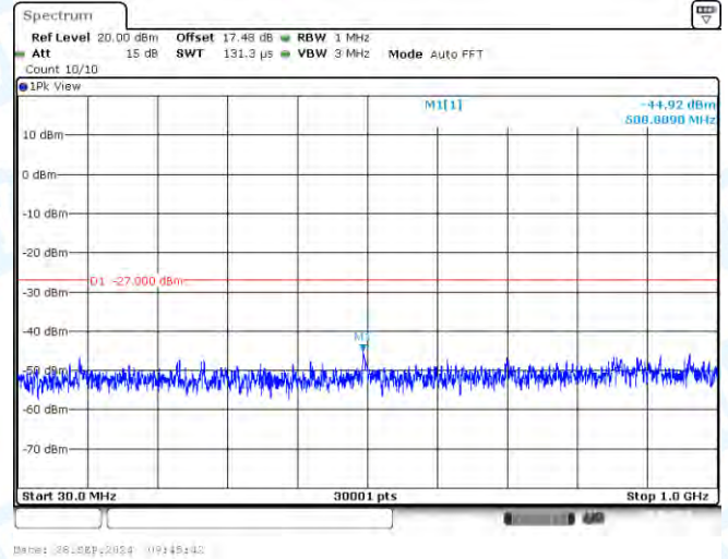
11N40-CDD-Ant2-5190-30~1000-PASS
