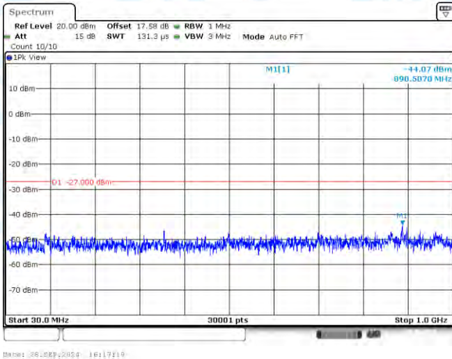
11A-CDD-Ant3-5280-30~1000-PASS
