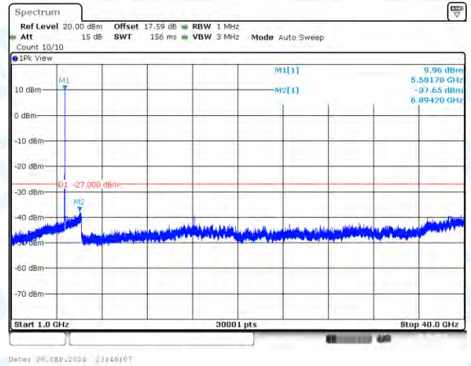
11N20-CDD-Ant1-5580-1000~40000-PASS
