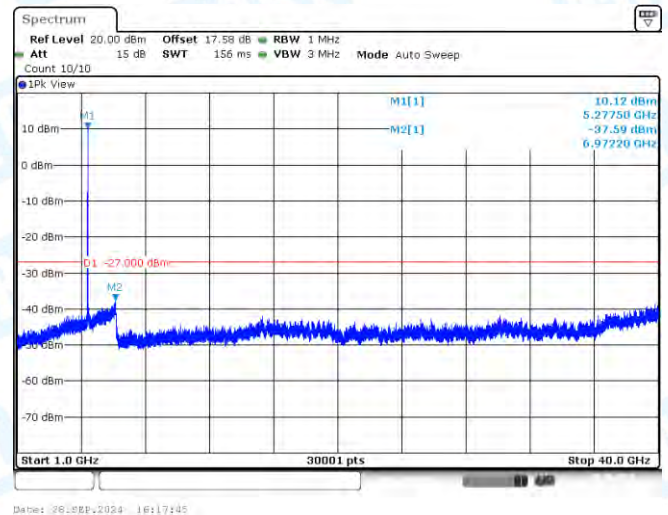
11A-CDD-Ant3-5280-1000~40000-PASS
