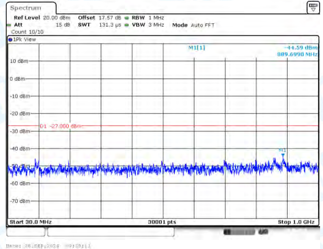
11N20-CDD-Ant2-5240-30~1000-PASS
