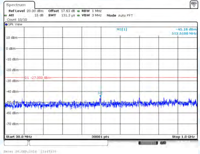
11N20-CDD-Ant2-5580-30~1000-PASS
