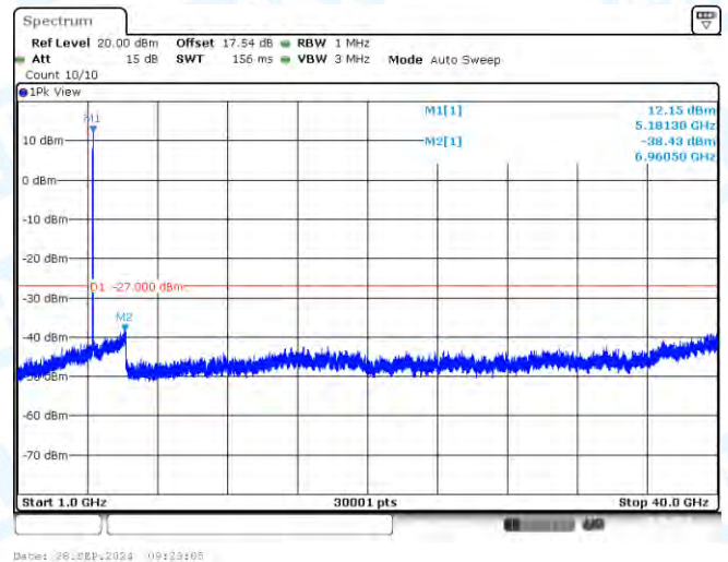
11N20-CDD-Ant3-5180-1000~40000-PASS
