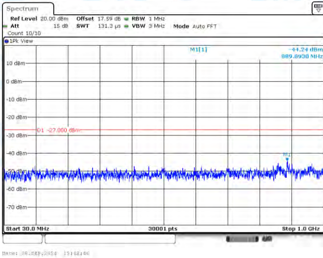
11A-Ant3-5320-30~1000-PASS
