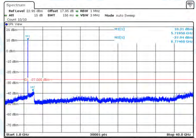
11N20-CDD-Ant1-5720-1000~40000-PASS
