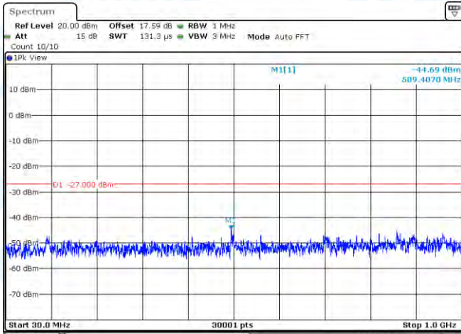
11A-CDD-Ant1-5580-30~1000-PASS
