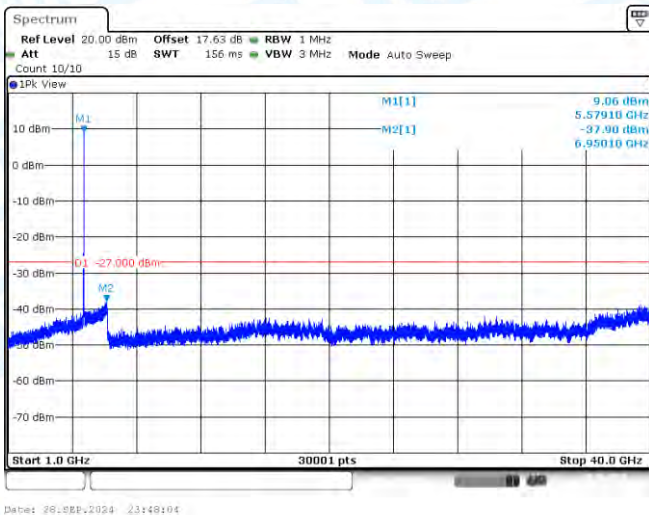
11N20-CDD-Ant2-5580-1000~40000-PASS
