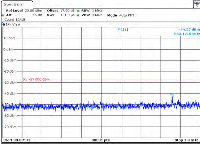
11N20-CDD-Ant1-5720-30~1000-PASS
