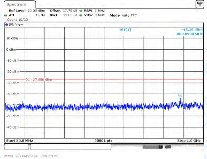
11A-CDD-Ant2-5745-30~1000-PASS
