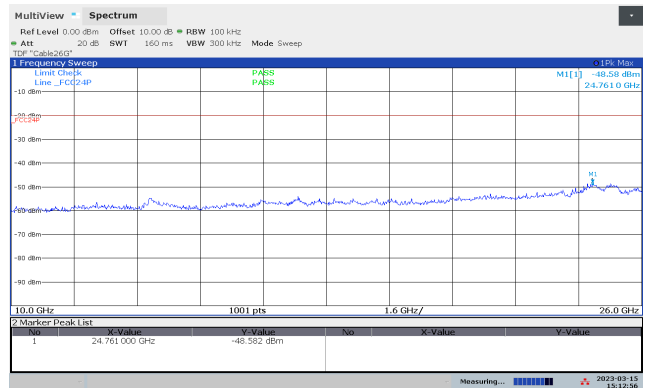
Conducted Emissions 10-26 GHz, 2480 MHz, 1Mb
