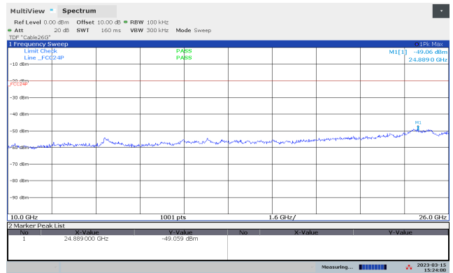
Conducted Emissions 10-26 GHz, 2402 MHz, 1Mb
