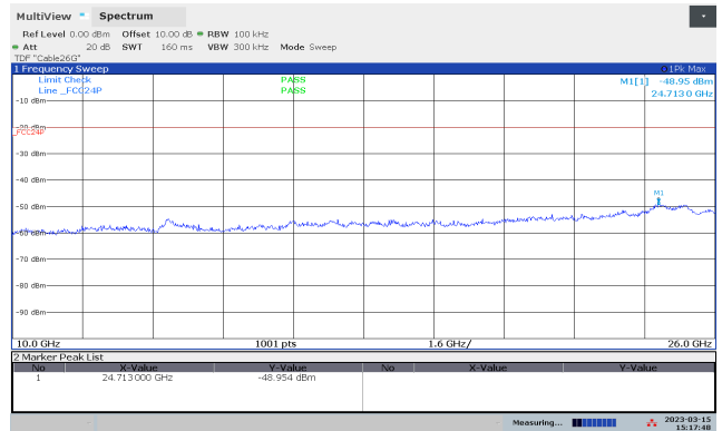
Conducted Emissions 10-26 GHz, 2440 MHz, 1Mb
