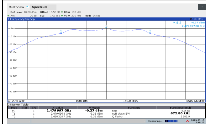
DTS BW, 2480 MHz, 1M
