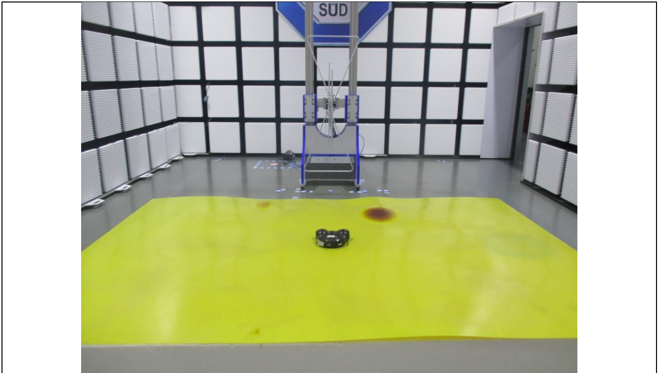
Radiated Emission test (30MHz to 1000MHz)
