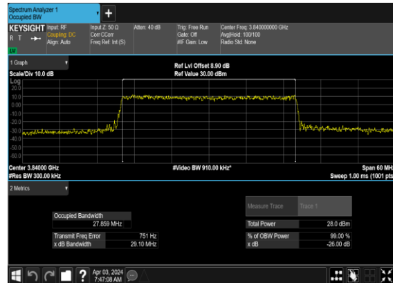
B2_N77(30M)_CP-OFDM_16 QAM_Outer_Full_Mid_CH
