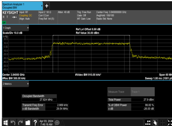
B2_N77(30M)_CP- OFDM_QPSK_Outer_Full_Mid_CH
