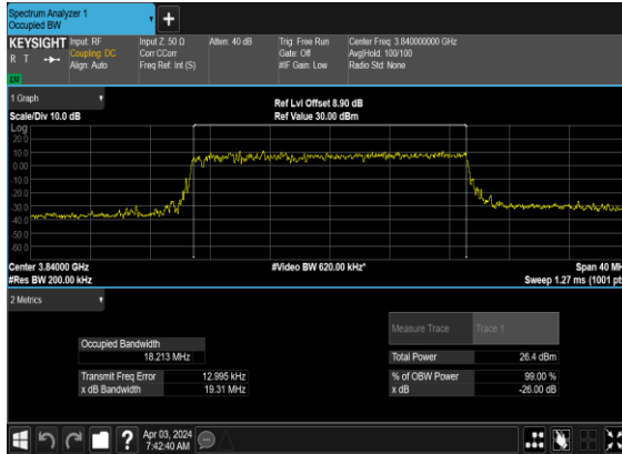
B2_N77(20M)_CP- OFDM_QPSK_Outer_Full_Mid_CH
