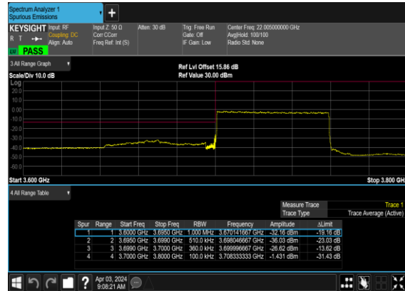
B2_N77(60M)_DFT-s- OFDM_BPSK_Outer_Full_Low_CH
