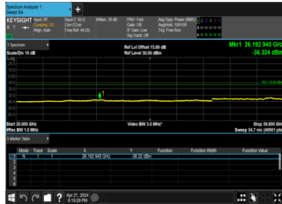
B2_N77(20M)_DFT-s- OFDM_BPSK_Edge_1RB_Left_Low_CH
