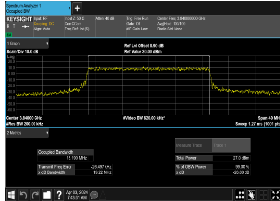
B2_N77(20M)_CP-OFDM_16 QAM_Outer_Full_Mid_CH
