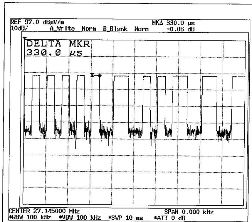
Duty Cycle 3
