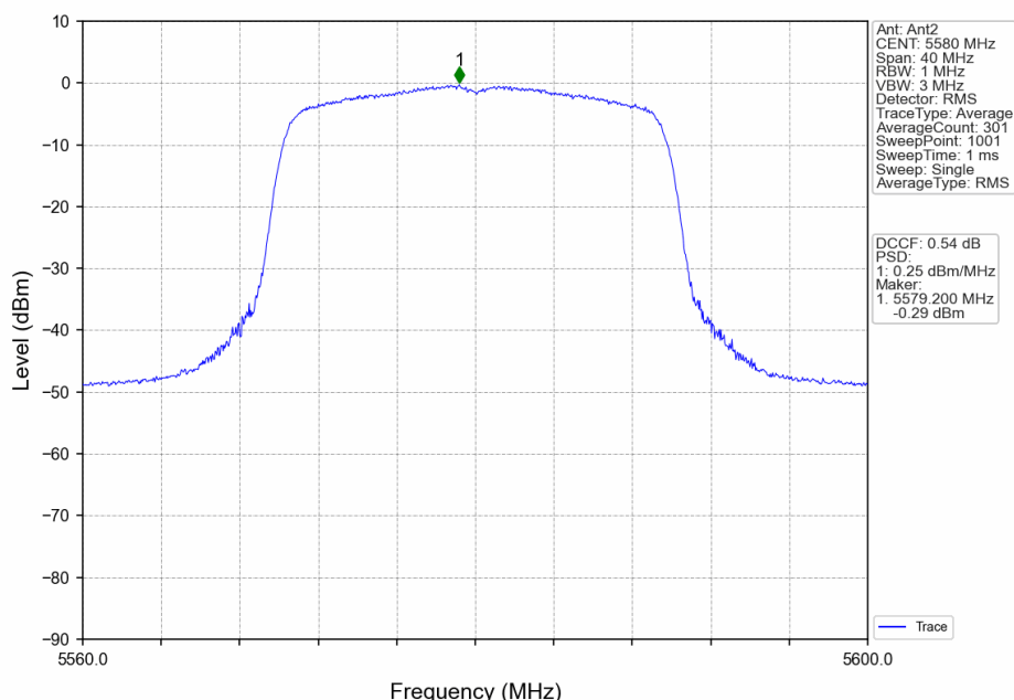
802.11ax(HEW20)_MCH_5580MHz_RU242_Left_Ant2_NTNV
