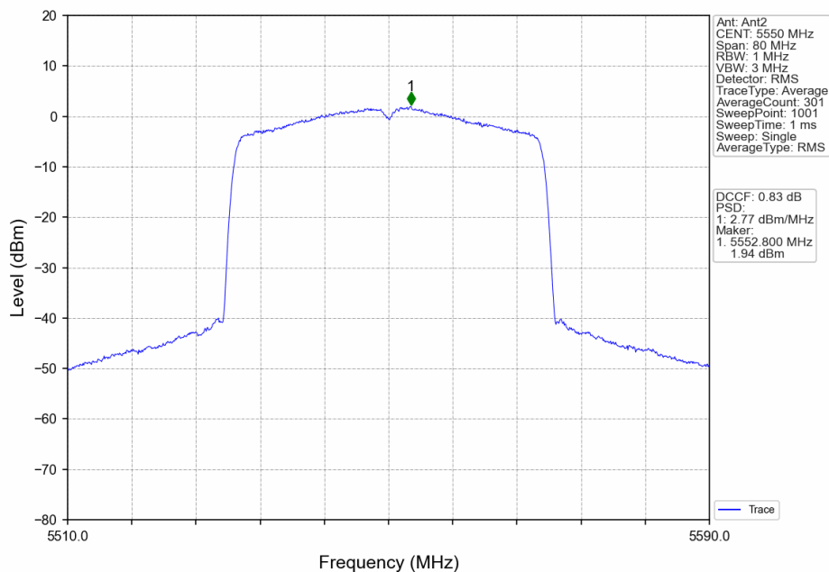
802.11ax(HEW40)_MCH_5550MHz_RU484_Left_Ant2_NTNV
