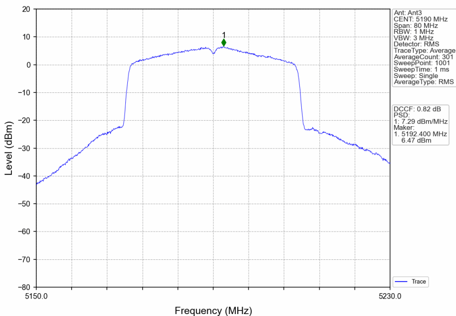
802.11ax(HEW40)_LCH_5190MHz_RU484_Left_MIMO_NTNV
