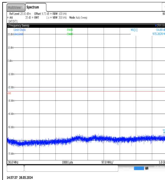
NTNV-N77-3700-3980-PC3-30-60-L-DFT-QPSK- Edge_1RB_Left-30-1000-Ant1-PASS
