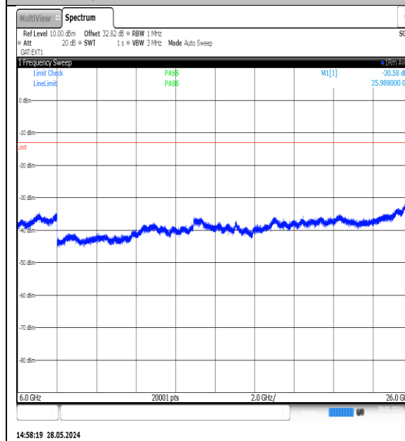
NTNV-N77-3700-3980-PC3-30-60-L-DFT-QPSK- Edge_1RB_Left-6000-26000-Ant1-PASS
