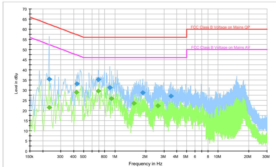
Fig.A.7.2 AC Powerline Conducted Emission-Idle
