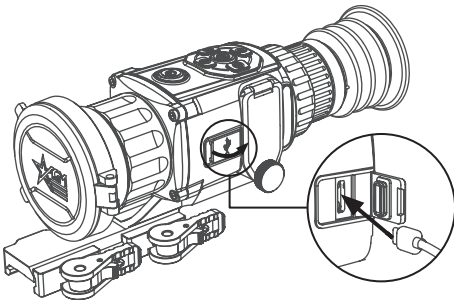
FIGURE 2-2. CABLE INTERFACE
