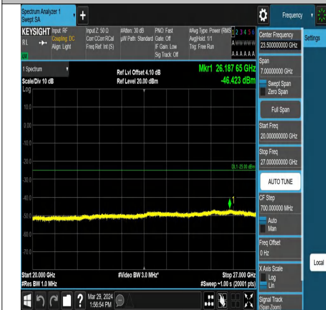
Band7_15MHz_QPSK_20825_1RB#0_20000~27000_20000~27000
