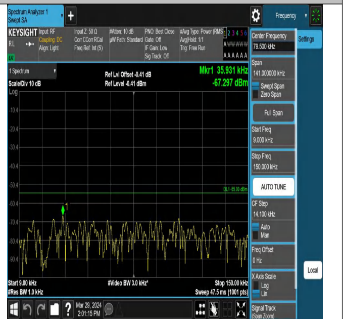
Band7_20MHz_QPSK_21350_1RB#0_0.009~0.15_0.009~0.15
