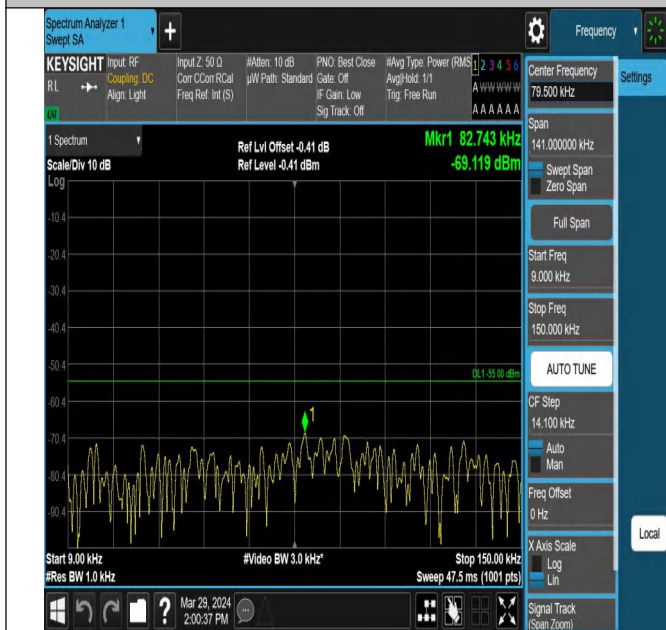
Band7_20MHz_QPSK_21100_1RB#0_0.009~0.15_0.009~0.15
