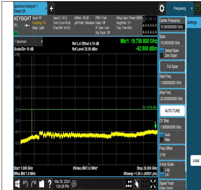
Band7_10MHz_QPSK_21400_1RB#0_1000~20000_1000~20000
