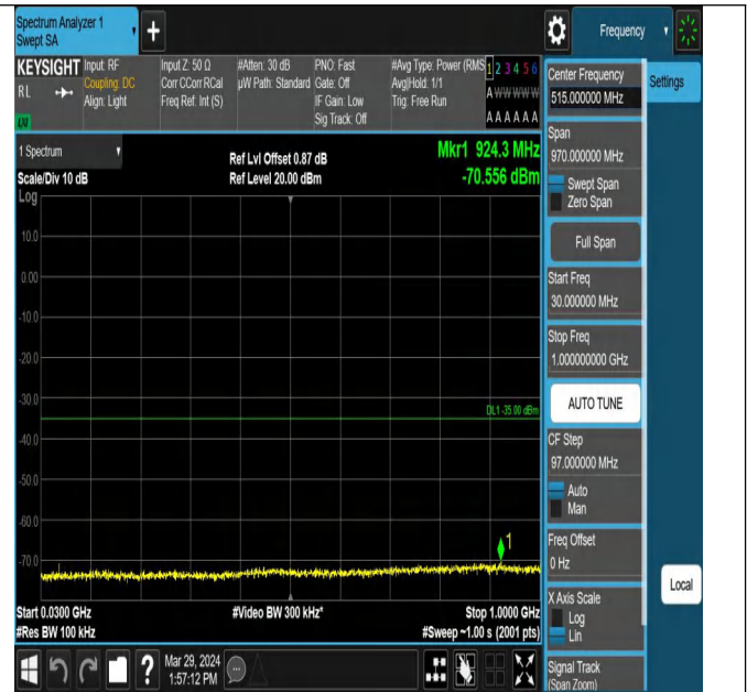
Band7_15MHz_QPSK_21100_1RB#0_30~1000_30~1000
