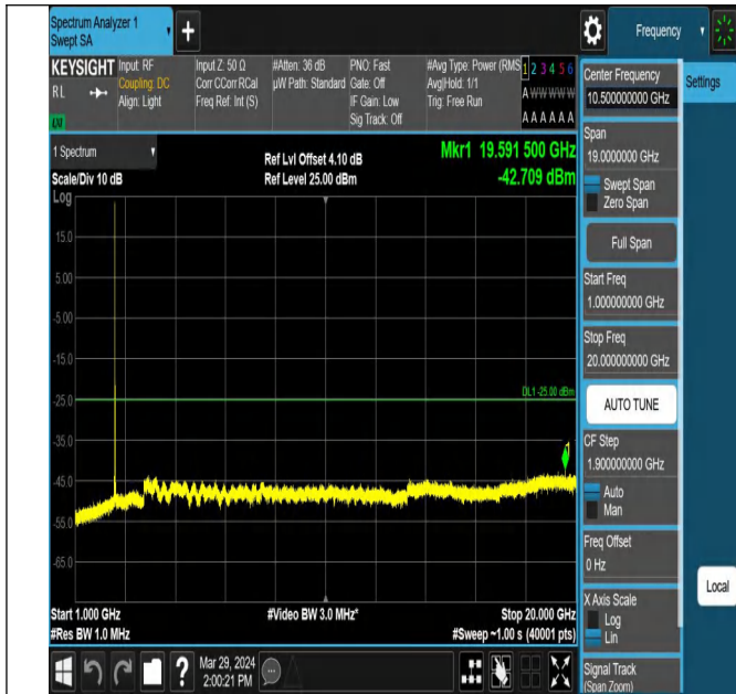
Band7_20MHz_QPSK_20850_1RB#0_1000~20000_1000~20000
