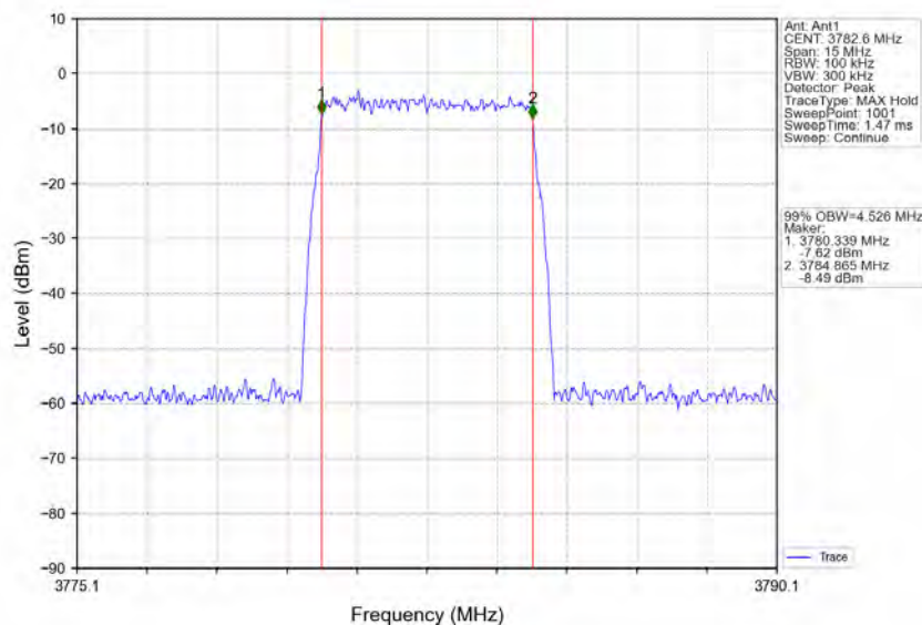
Bandn77a_3782.6MHz_AWGN_SISO_Ant1_NTNV_Input_AGC+3
