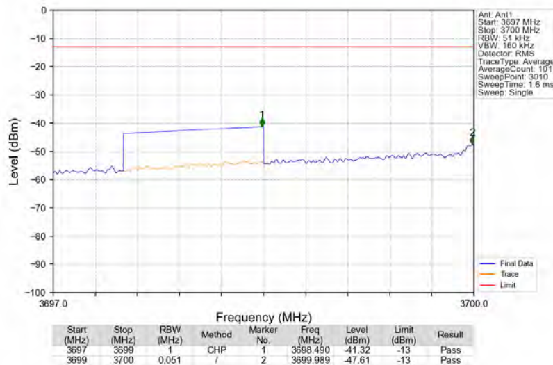
Bandn77a_3702.5MHz_AWGN_SISO_Ant1_NTNV_AGC
