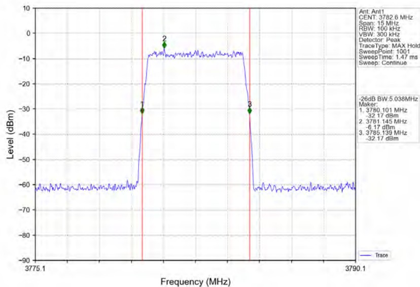
Bandn77a_3782.6MHz_AWGN_SISO_Ant1_NTNV_Input_AGC+3
