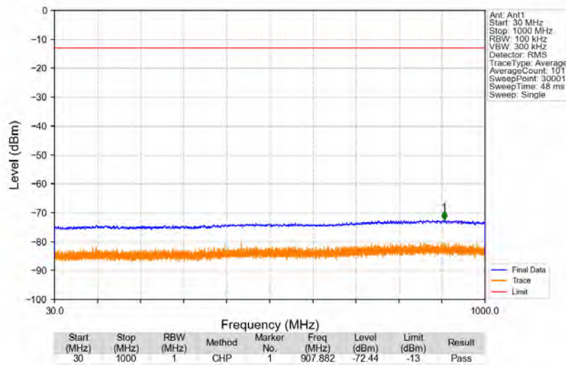
Bandn77a_3702.5MHz_AWGN_SISO_Ant1_NTNV
