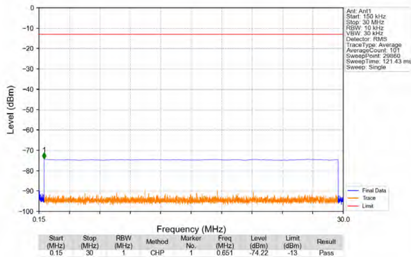
Bandn77a_3702.5MHz_AWGN_SISO_Ant1_NTNV
