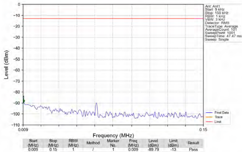
Bandn77a_3702.5MHz_AWGN_SISO_Ant1_NTNV
