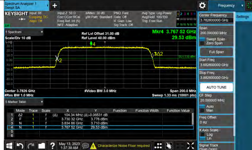
Bandn77a 3782.6MHz AWGN SISO Ant1 NTN Output AGC+3
