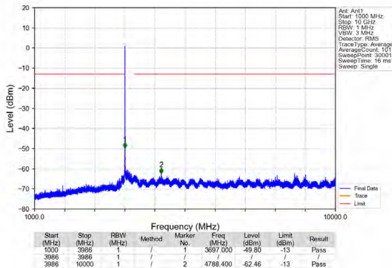
Bandn77a_3702.5MHz_AWGN_SISO_Ant1_NTNV
