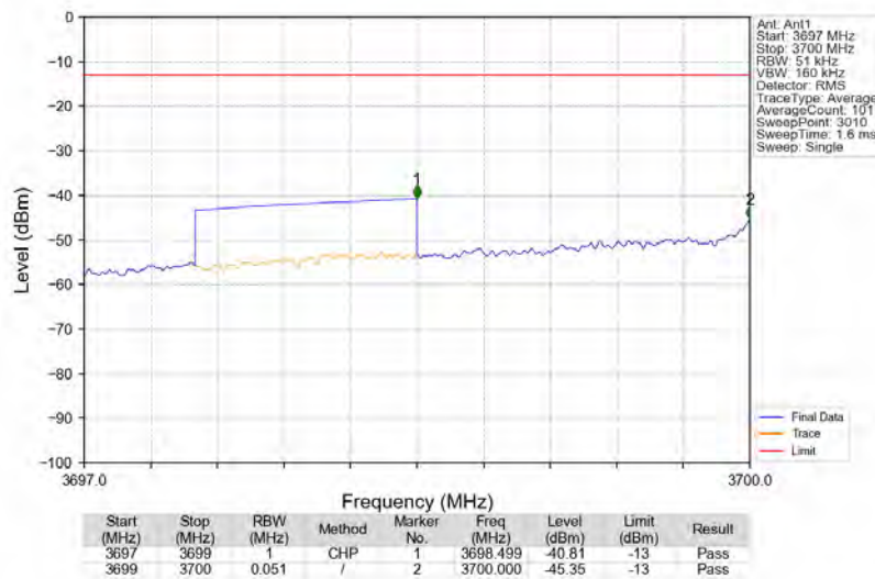
Bandn77a_3702.5MHz_AWGN_SISO_Ant1_NTNV_AGC+3
