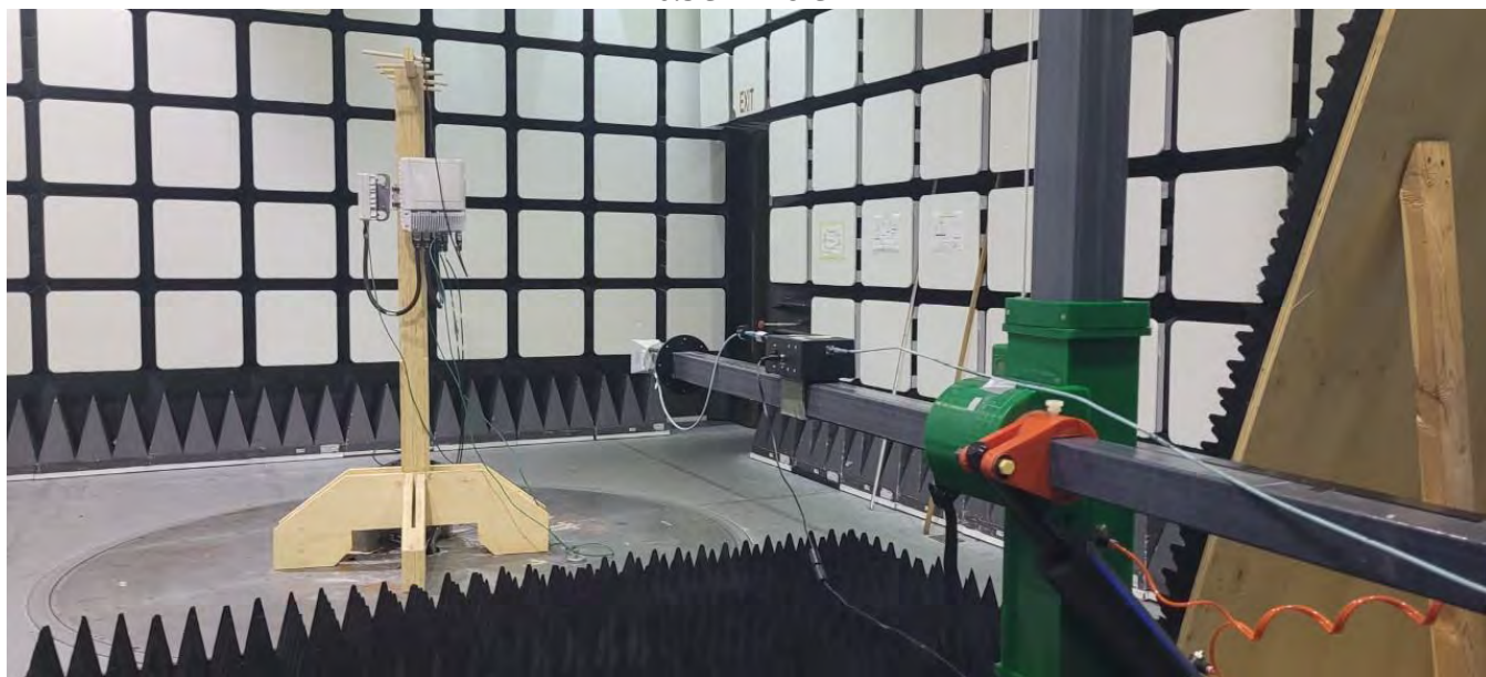
26.5GHz-40 GHz
