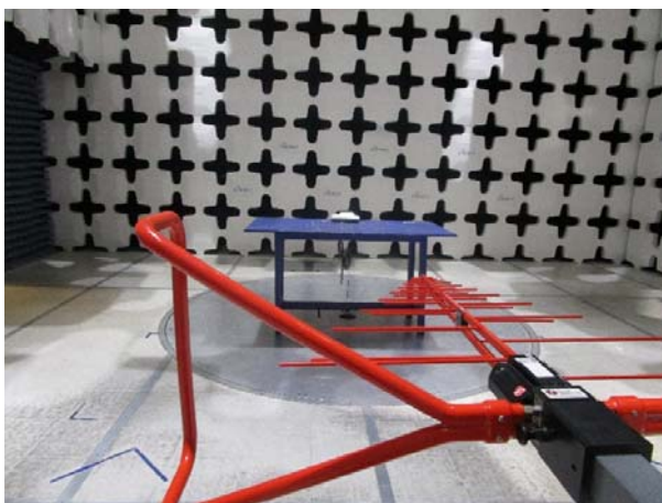
Radiated Emissions Below 1GHz– Front View
