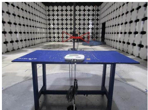
Radiated Emissions Below 1 GHz – Rear View
