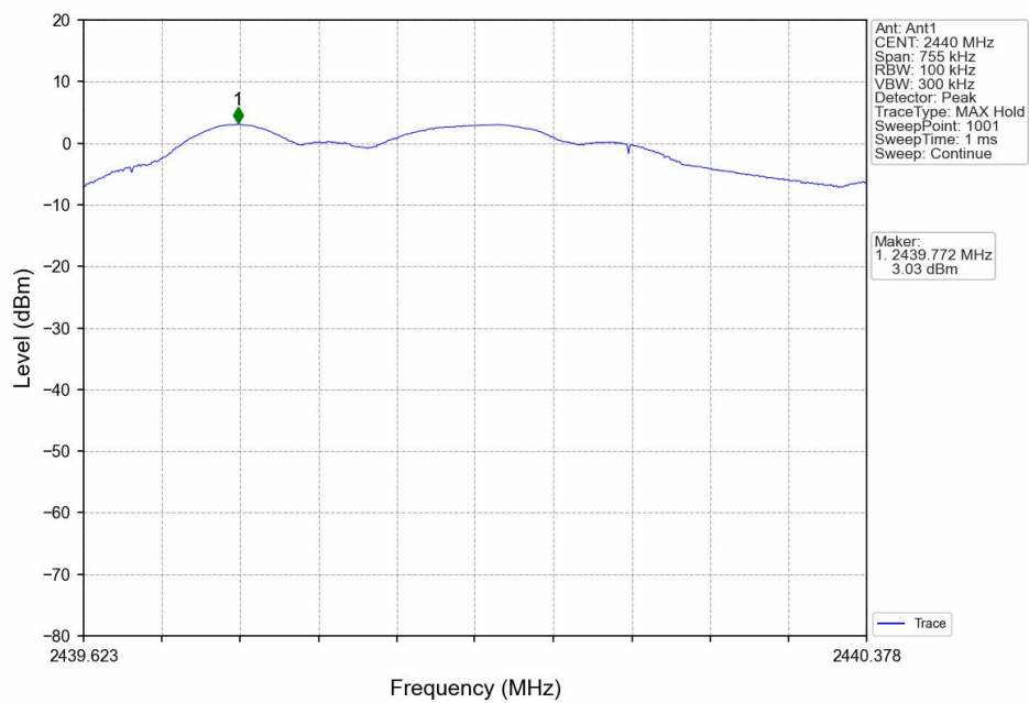
1M_LCH_2440MHz
