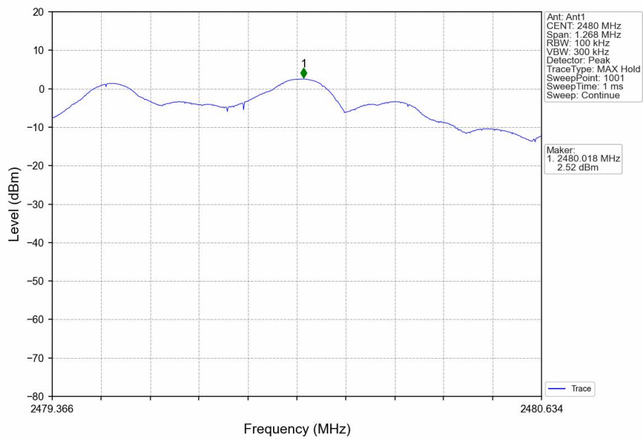
2M_LCH_2480MHz
