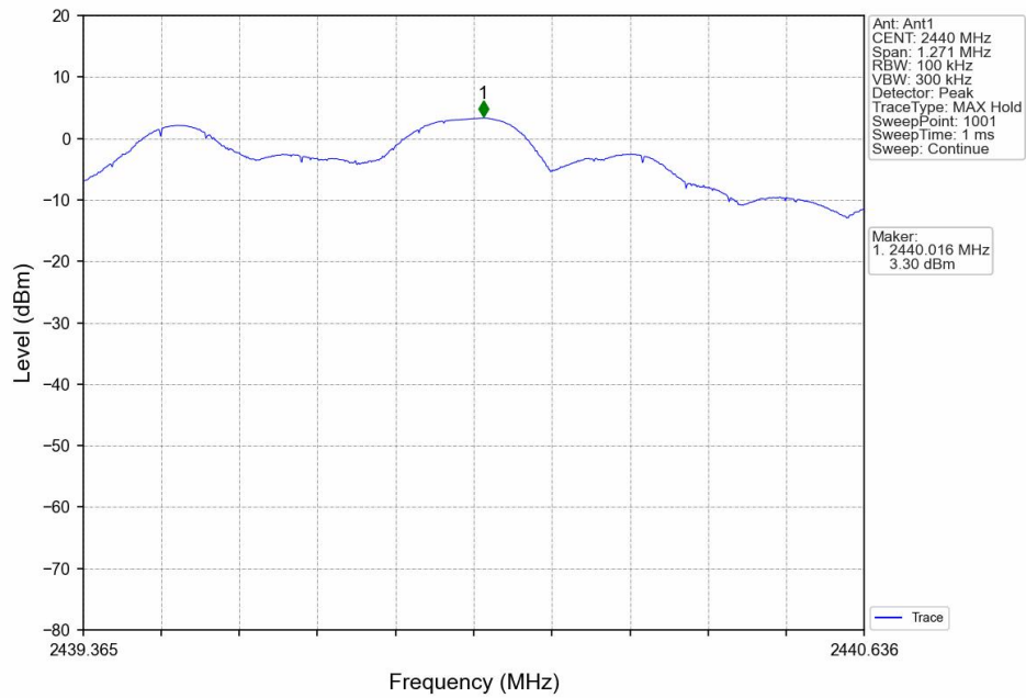
2M_LCH_2440MHz
