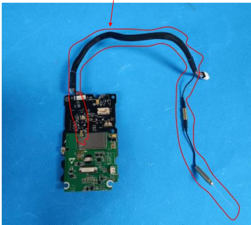
Wireless antenna
