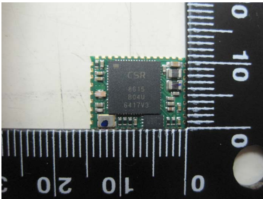
Front View of the BT module
