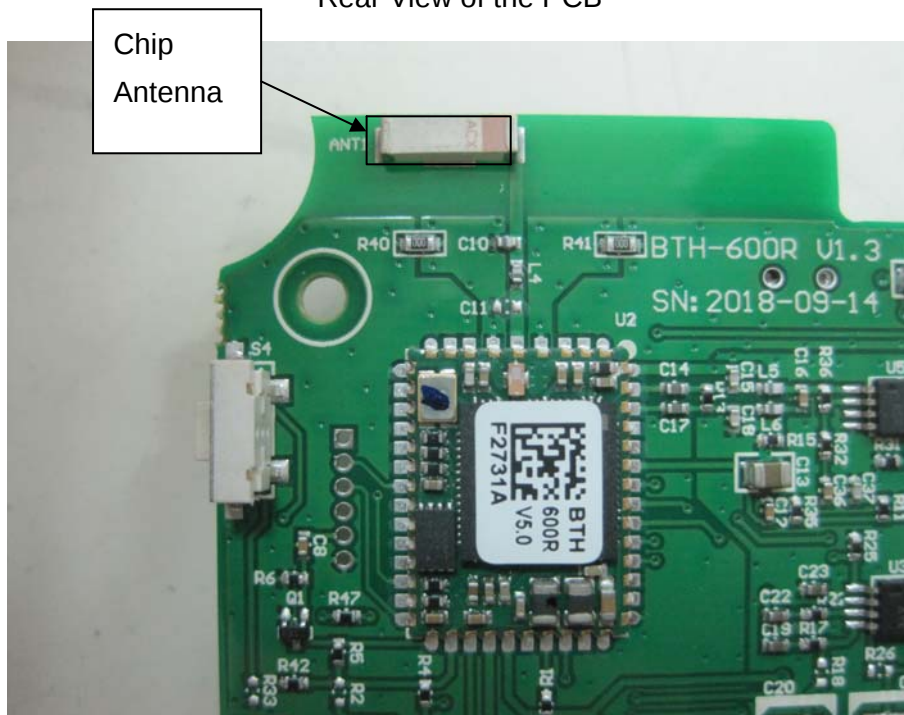
Close Up View of the BT module & Antenna
