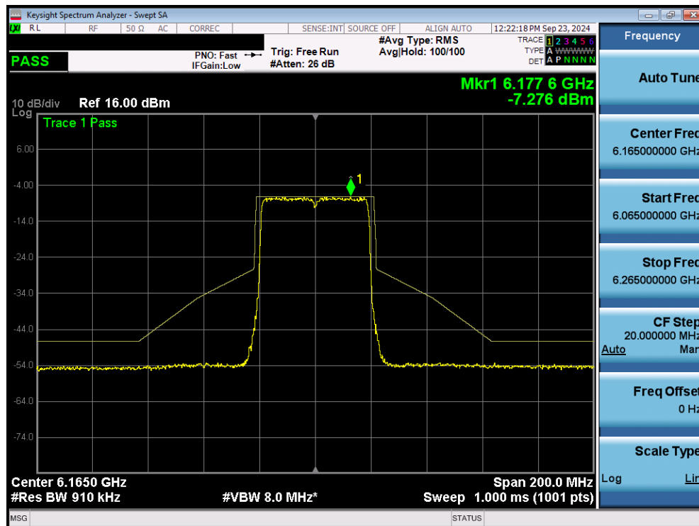
Plot 7-74. In Band Emissions Plot MIMO ANT1 (40MHz 802.11ax/be (Full Tones) (UNII Band 5) – Ch. 43) - VLP
