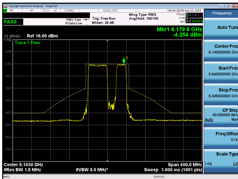
Plot 7-84. In Band Emissions Plot MIMO ANT2 (80MHz 802.11be (484+242 Tones) (UNII Band 5) – Ch. 39) VLP
