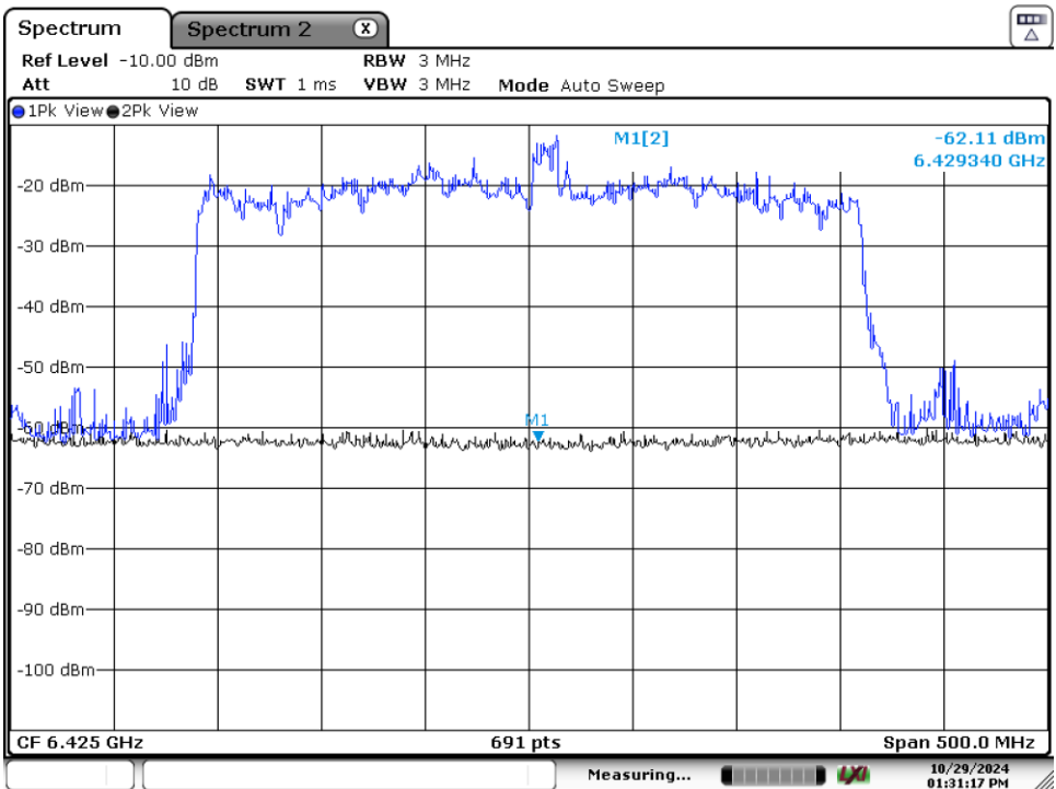
Plot 7-102. CBP 320MHz Channel - Injection Center – [6425 MHz]
