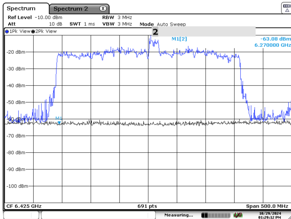
Plot 7-101. CBP 320MHz Channel - Injection Lower Edge – [6270 MHz]
