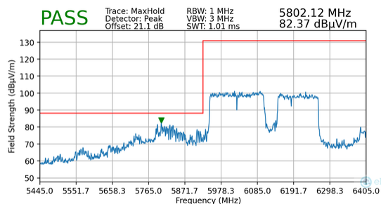
Plot 7-137. Radiated Lower Band Edge Plot MIMO (Peak – UNII Band 5 – 3*996+484T)
