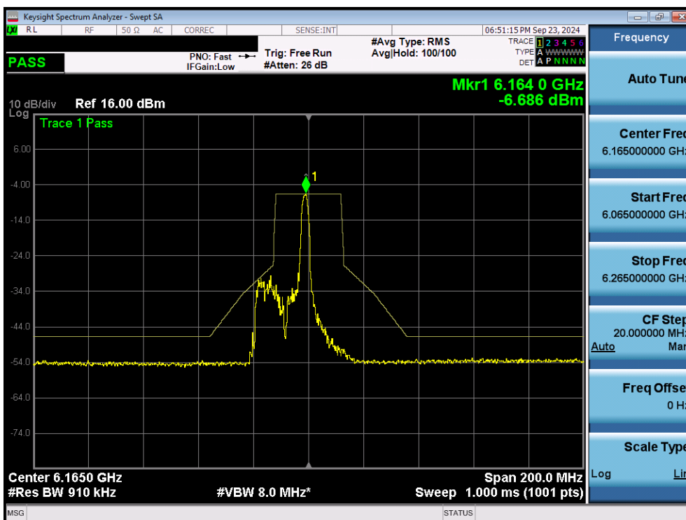
Plot 7-79. In Band Emissions Plot MIMO ANT2 (40MHz 802.11ax/be (26 Tones) (UNII Band 5) – Ch. 43) - VLP
