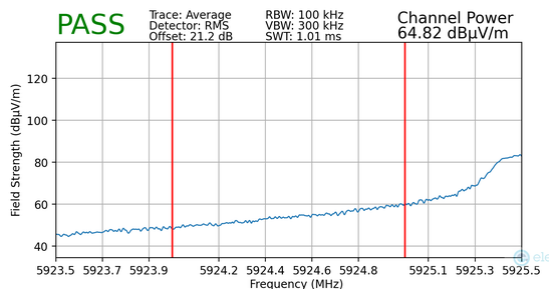
Plot 7-114. Radiated Lower Band Edge Plot MIMO (Average – UNII Band 5 – 106+26T)
