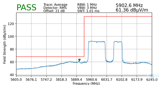
Plot 7-130. Radiated Lower Band Edge Plot MIMO (Average – UNII Band 5 – 996+484T)
