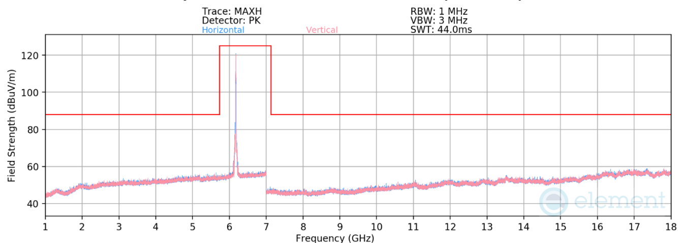
Plot 7-104. Radiated Spurious Plot 1GHz – 18GHz MIMO (802.11ax – UNII Band 5 Ch. 45)
