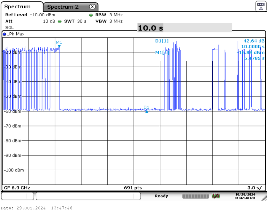
Plot 7-100. Contention Based Protocol Timing Plot (320MHz (UNII Band 7) – Ch. 175 High)
