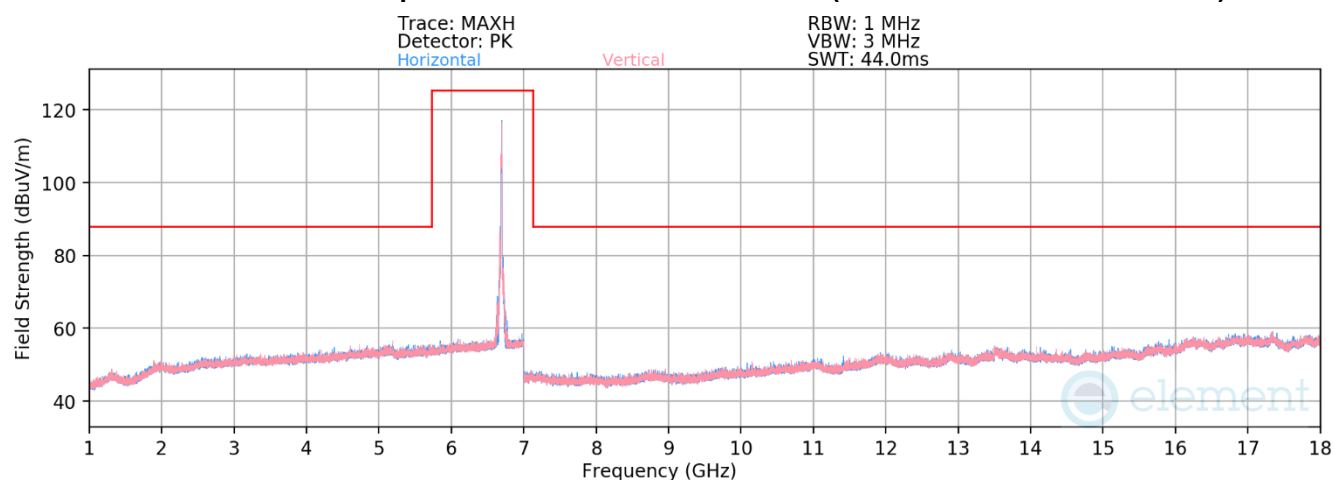
Plot 7-105. Radiated Spurious Plot 1GHz – 18GHz MIMO (802.11ax – UNII Band 7 Ch. 149)
