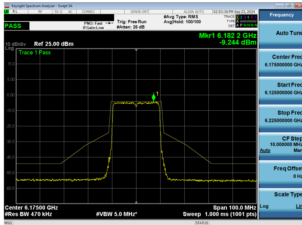
Plot 7-87. In Band Emissions Plot MIMO ANT2 (20MHz 802.11ax/be (Full Tones) (UNII Band 5) – Ch. 45) - VLP
