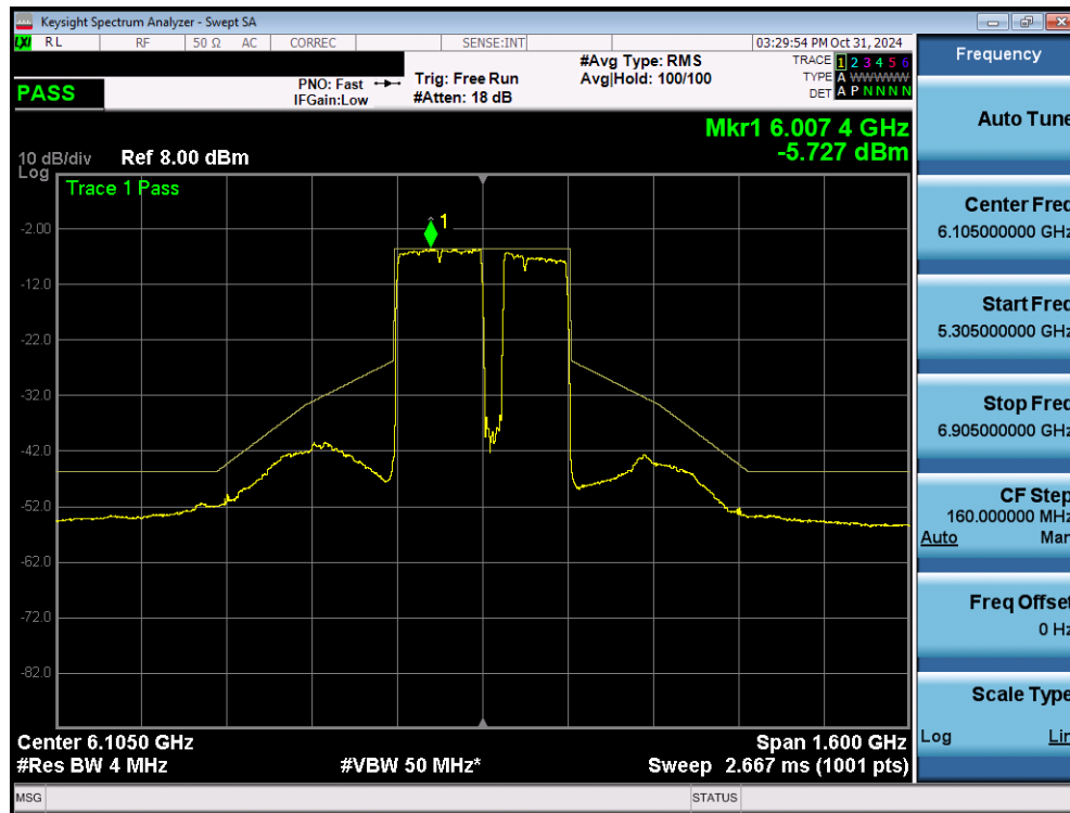
Plot 7-86. In Band Emissions Plot MIMO ANT2 (320MHz 802.11be (3*996+484 Tones) (UNII Band 5) – Ch. 31) VLP
