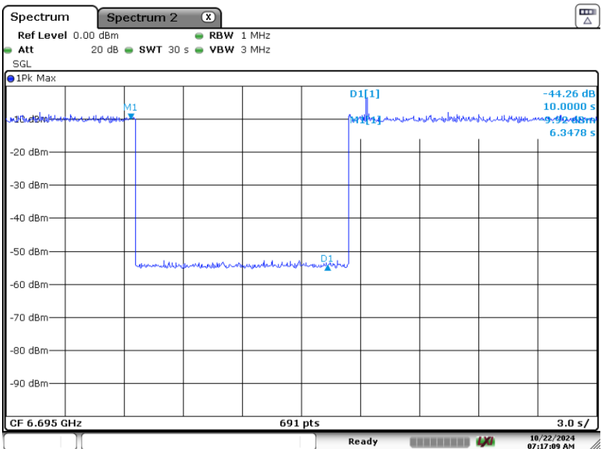
Plot 7-97. Contention Based Protocol Timing Plot (20MHz (UNII Band 7) – Ch. 149)
