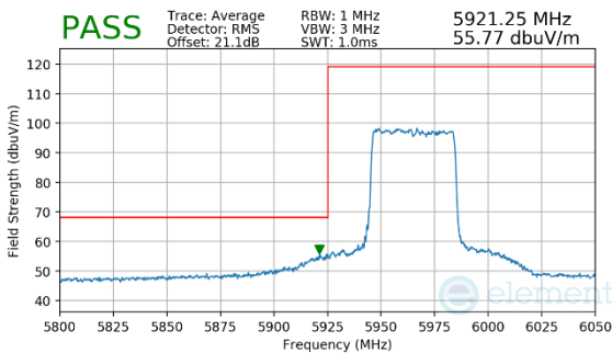
Plot 7-122. Radiated Lower Band Edge Plot MIMO (Average – UNII Band 5 – 484T)
