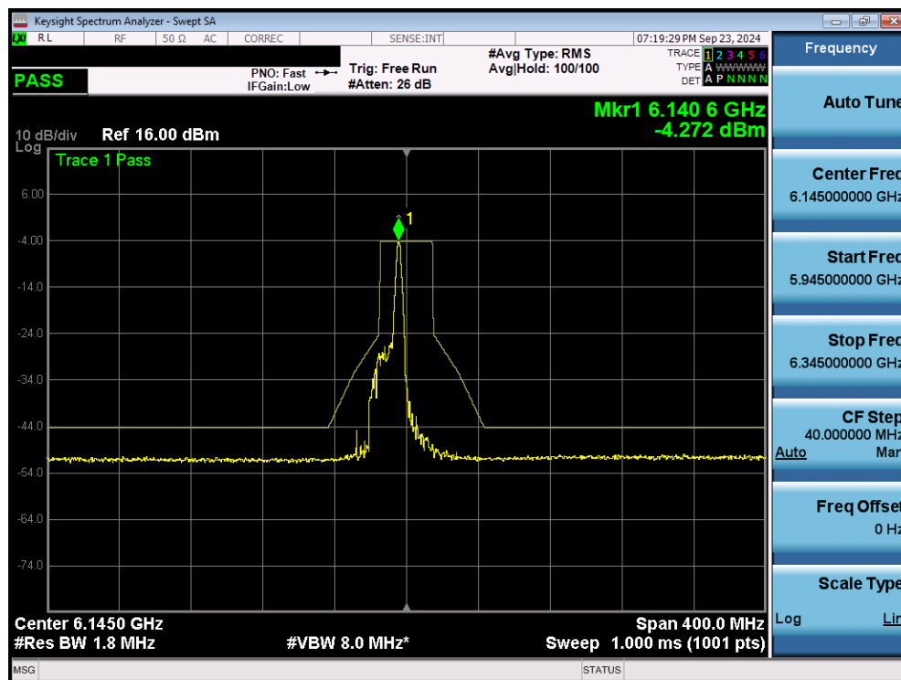
Plot 7-80. In Band Emissions Plot MIMO ANT2 (80MHz 802.11ax/be (26 Tones) (UNII Band 5) – Ch. 39) - VLP
