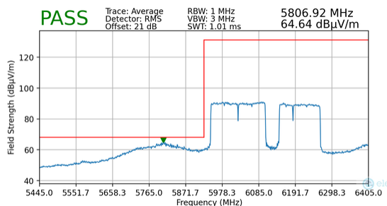
Plot 7-136. Radiated Lower Band Edge Plot MIMO (Average – UNII Band 5 – 3*996+484T)
