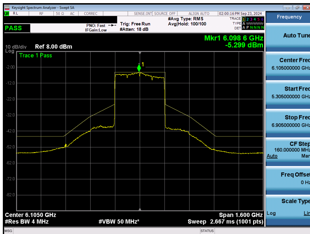
Plot 7-77. In Band Emissions Plot MIMO ANT1 (320MHz 802.11be (Full Tones) (UNII Band 5) – Ch. 31) - VLP
