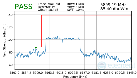
Plot 7-129. Radiated Lower Band Edge Plot MIMO (Peak – UNII Band 5 – 2x996T)
