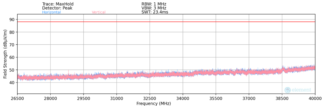
Plot 7-107. Radiated Spurious Plot 26.5GHz - 40GHz (802.11ax)
