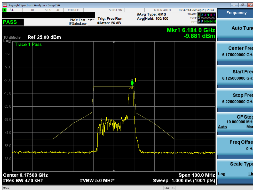
Plot 7-78. In Band Emissions Plot MIMO ANT2 (20MHz 802.11ax/be (26 Tones) (UNII Band 5) – Ch. 45) - VLP
