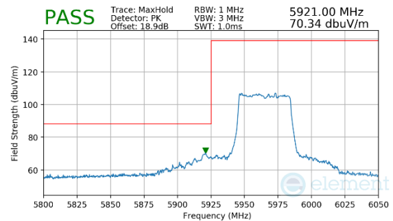
Plot 7-123. Radiated Lower Band Edge Plot MIMO (Peak – UNII Band 5 – 484T)
