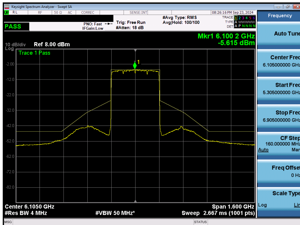
Plot 7-91. In Band Emissions Plot MIMO ANT2 (320MHz 802.11be (Full Tones) (UNII Band 5) – Ch. 31) - VLP
