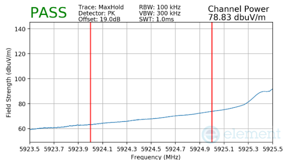
Plot 7-113. Radiated Lower Band Edge Plot MIMO (Peak – UNII Band 5 – 106T)
