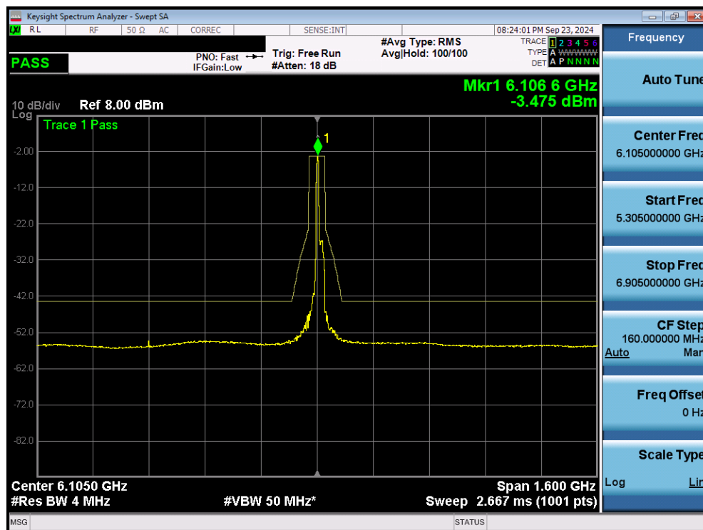
Plot 7-82. In Band Emissions Plot MIMO ANT2 (320MHz 802.11be (26 Tones) (UNII Band 5) – Ch. 31) - VLP
