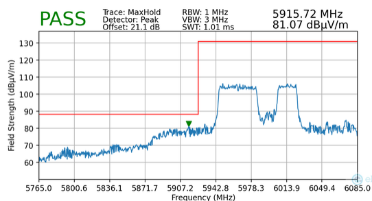
Plot 7-127. Radiated Lower Band Edge Plot MIMO (Peak – UNII Band 5 – 484+242T)
