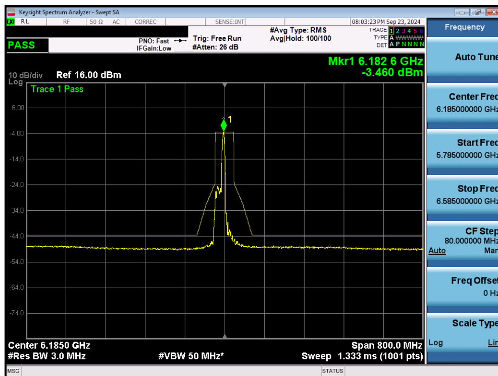
Plot 7-81. In Band Emissions Plot MIMO ANT2 (160MHz 802.11ax/be (26 Tones) (UNII Band 5) – Ch. 47) - VLP
