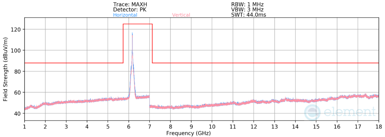
Plot 7-108. Radiated Spurious Plot 1GHz – 18GHz MIMO (802.11ax – UNII Band 5 Ch. 45)
