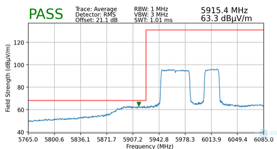
Plot 7-126. Radiated Lower Band Edge Plot MIMO (Average – UNII Band 5 – 484+242T)
