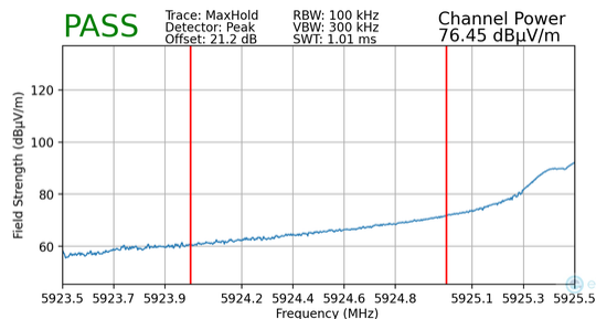
Plot 7-115. Radiated Lower Band Edge Plot MIMO (Peak – UNII Band 5 – 106+26T)
