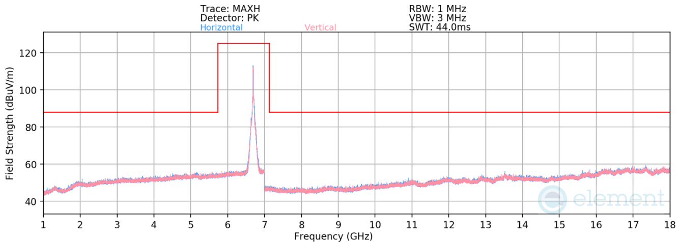
Plot 7-109. Radiated Spurious Plot 1GHz – 18GHz MIMO (802.11ax – UNII Band 7 Ch. 149)
