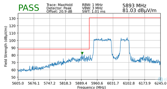
Plot 7-131. Radiated Lower Band Edge Plot MIMO (Peak – UNII Band 5 – 996+484T)
