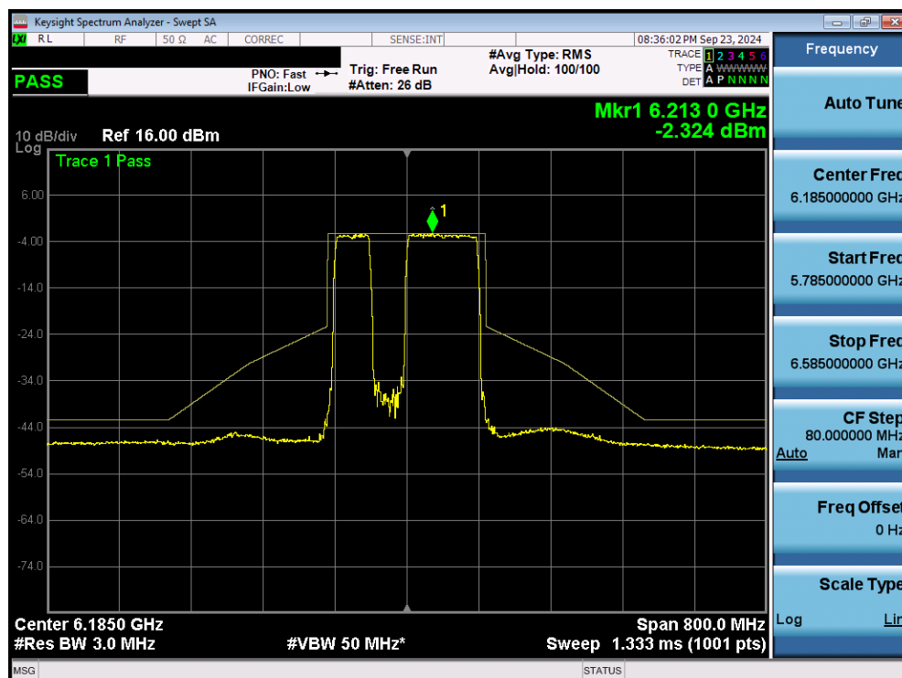
Plot 7-85. In Band Emissions Plot MIMO ANT2 (160MHz 802.11be (996+484 Tones) (UNII Band 5) – Ch. 47) VLP
