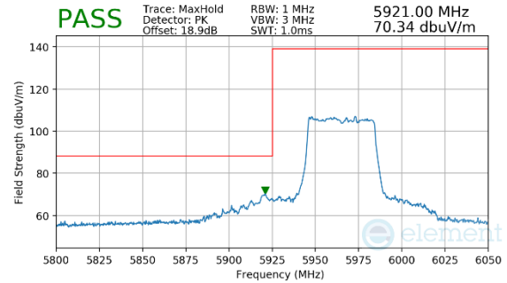
Plot 7-121. Radiated Lower Band Edge Plot MIMO (Peak – UNII Band 5 – 484T)
