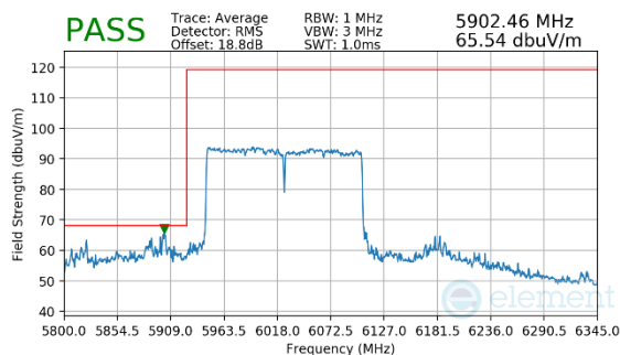
Plot 7-128. Radiated Lower Band Edge Plot MIMO (Average – UNII Band 5 – 2x996T)
