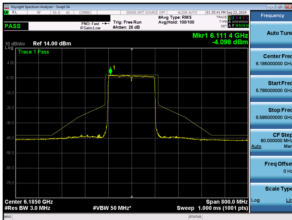
Plot 7-76. In Band Emissions Plot MIMO ANT1 (160MHz 802.11ax/be (Full Tones) (UNII Band 5) – Ch. 47) - VLP
