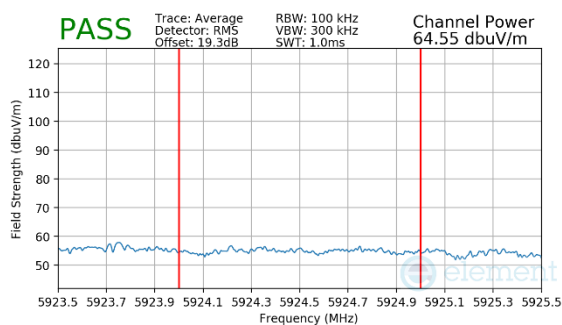
Plot 7-124. Radiated Lower Band Edge Plot MIMO (Average – UNII Band 5 – 996T)
