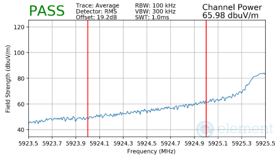
Plot 7-116. Radiated Lower Band Edge Plot MIMO (Average – UNII Band 5 – 242T)
