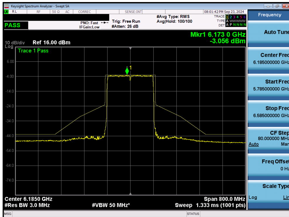
Plot 7-90. In Band Emissions Plot MIMO ANT2 (160MHz 802.11ax/be (Full Tones) (UNII Band 5) – Ch. 47) - VLP
