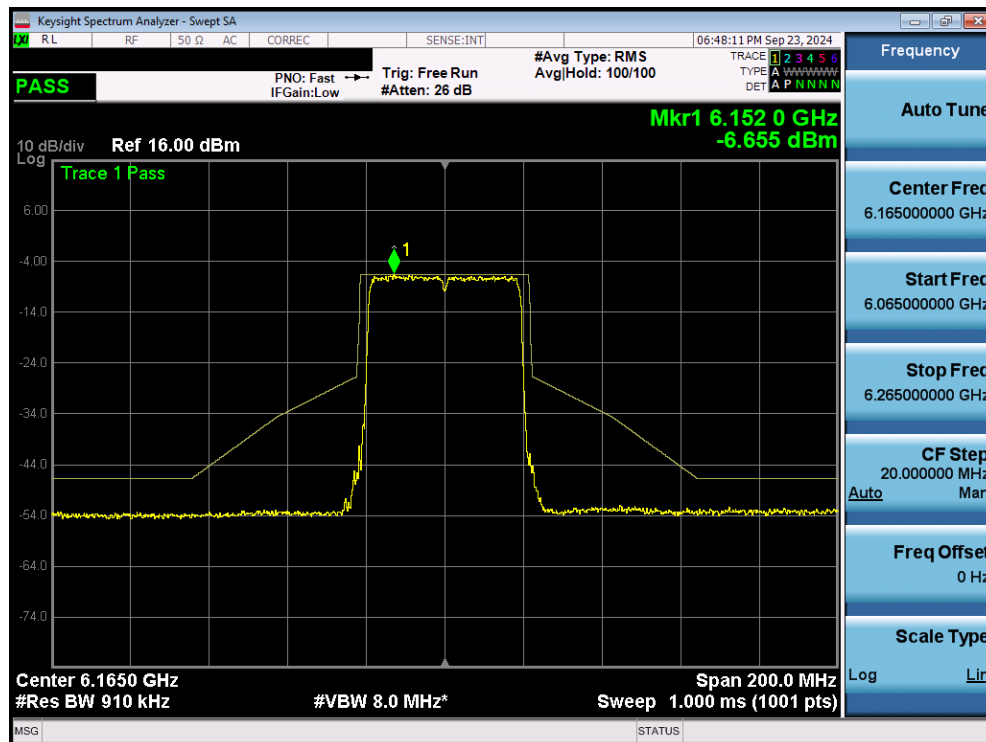
Plot 7-88. In Band Emissions Plot MIMO ANT2 (40MHz 802.11ax/be (Full Tones) (UNII Band 5) – Ch. 43) - VLP
