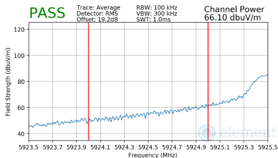
Plot 7-112. Radiated Lower Band Edge Plot MIMO (Average – UNII Band 5 – 106T)
