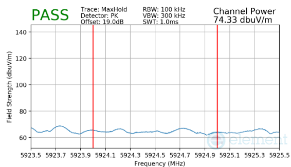
Plot 7-125. Radiated Lower Band Edge Plot MIMO (Peak – UNII Band 5 – 996T)
