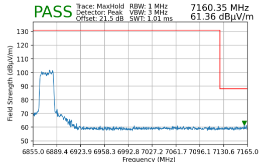
Plot 7-119. Radiated Upper Band Edge Plot MIMO (Peak – UNII Band 7 – 242T)
