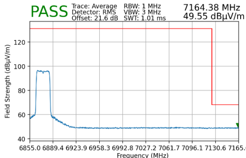
Plot 7-118. Radiated Upper Band Edge Plot MIMO (Average – UNII Band 7 – 242T)
