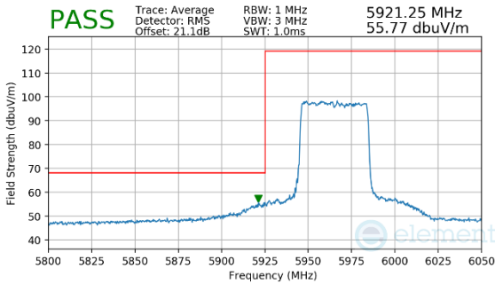
Plot 7-120. Radiated Lower Band Edge Plot MIMO (Average – UNII Band 5 – 484T)
