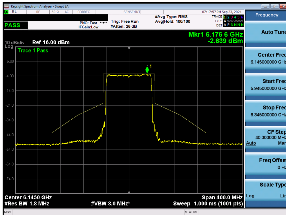
Plot 7-89. In Band Emissions Plot MIMO ANT2 (80MHz 802.11ax/be (Full Tones) (UNII Band 5) – Ch. 39) - VLP
