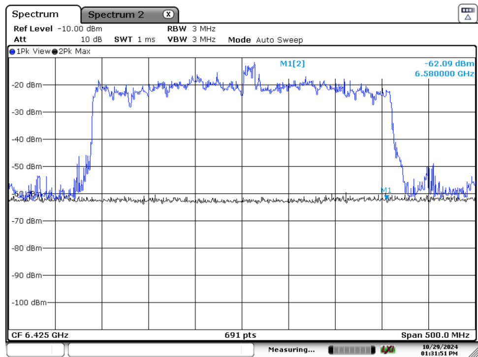
Plot 7-103. CBP 320MHz Channel - Injection Upper Edge – [6580 MHz]
