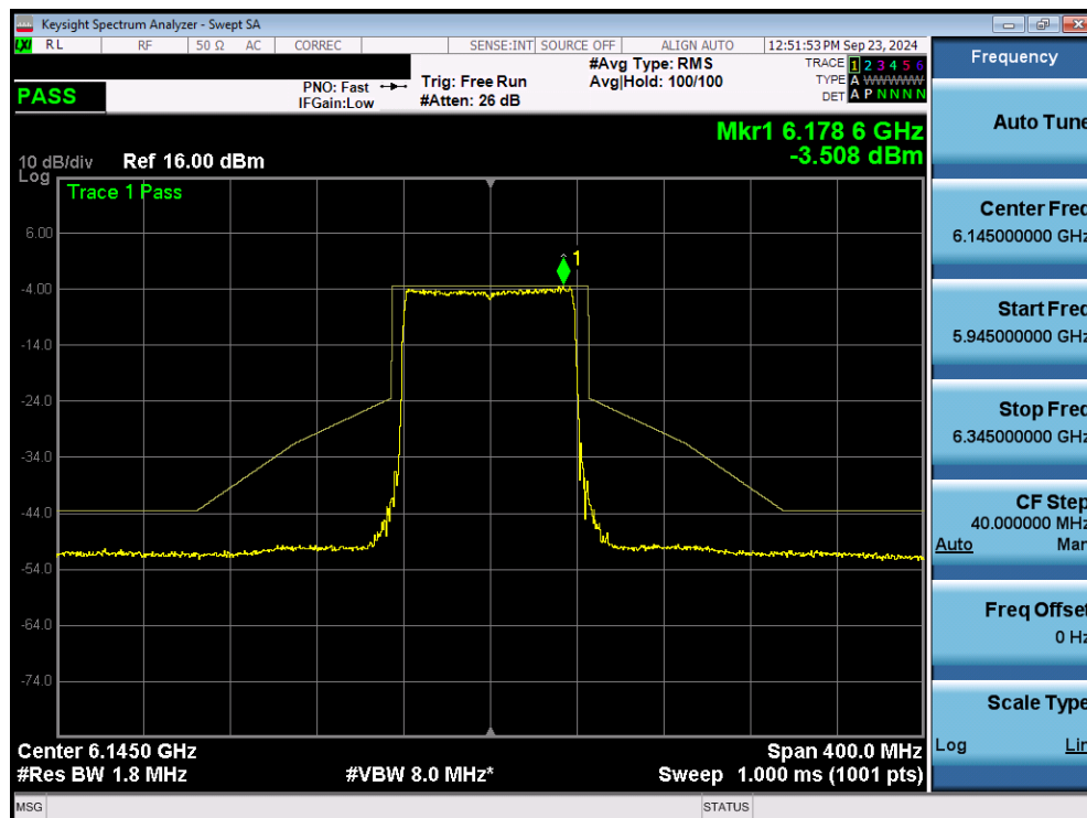
Plot 7-75. In Band Emissions Plot MIMO ANT1 (80MHz 802.11ax/be (Full Tones) (UNII Band 5) – Ch. 39) - VLP
