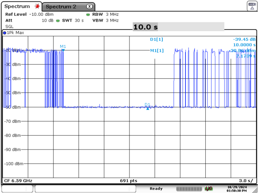
Plot 7-98. Contention Based Protocol Timing Plot (320MHz (UNII Band 7) – Ch. 175 Low)
