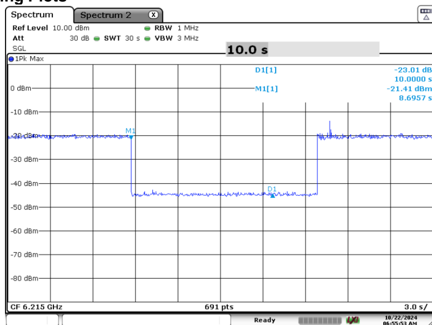
Plot 7-93. Contention Based Protocol Timing Plot (20MHz (UNII Band 5) – Ch. 53)
