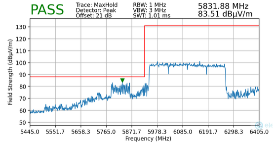
Plot 7-133. Radiated Lower Band Edge Plot MIMO (Peak – UNII Band 5 – 4*996T)
