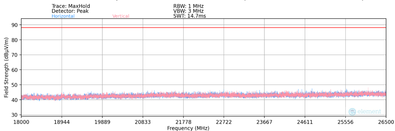
Plot 7-106. Radiated Spurious Plot 18GHz - 26.5GHz (802.11ax)
