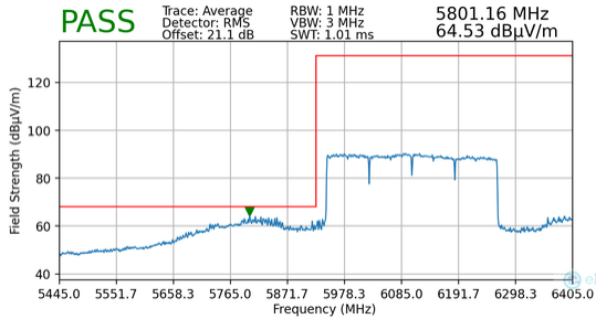
Plot 7-132. Radiated Lower Band Edge Plot MIMO (Average – UNII Band 5 – 4*996T)
