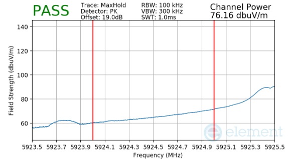
Plot 7-117. Radiated Lower Band Edge Plot MIMO (Peak – UNII Band 5 – 242T)
