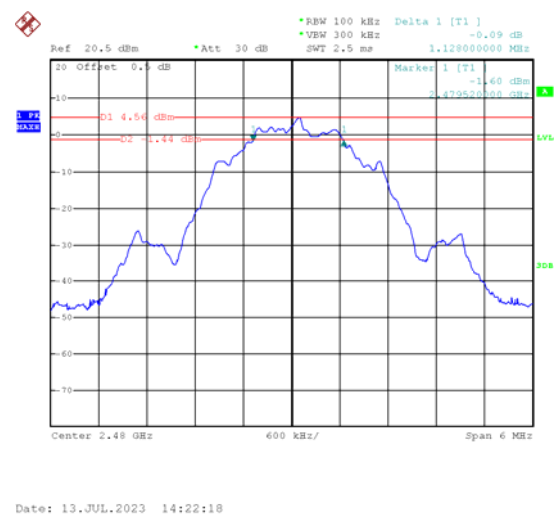
Mode: TX GFSK channel 39
