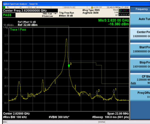
Band38_5MHz_16QAM_38225_1RB#24
