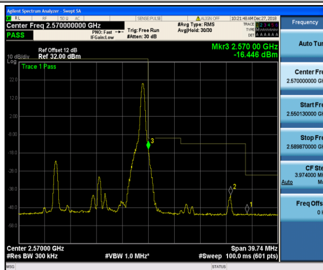
Band7_15MHz_QPSK_21375_1RB#74
