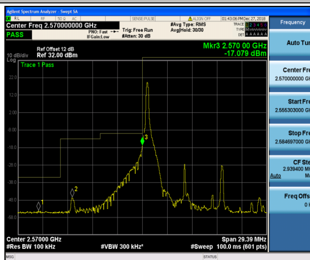
Band38_10MHz_QPSK_37800_1RB#0
