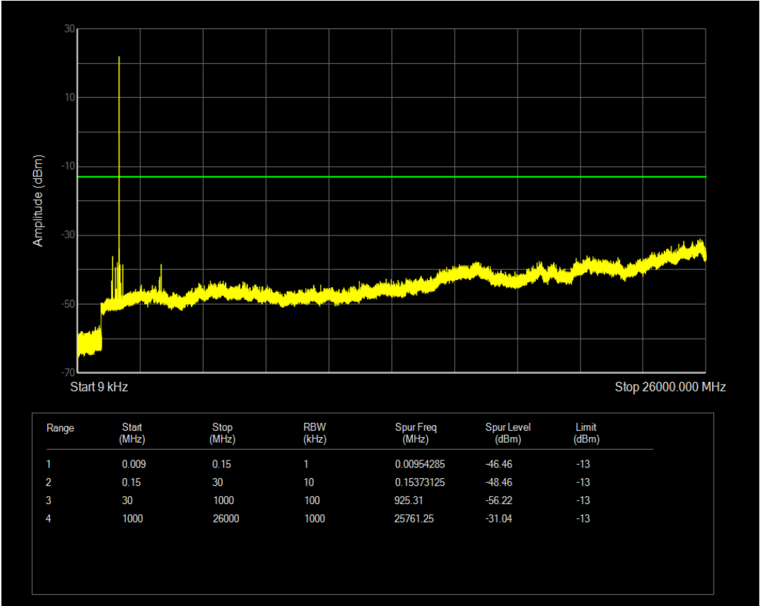
Band4 QAM16 BW=15MHz Channel=20325 RB Size=6 Position=#0 NB Index=0
