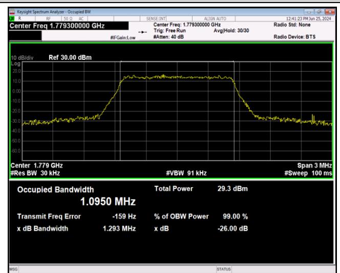
Band66-1.4MHz-64QAM-132322-6RB#0
