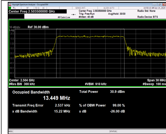
Band41-15MHz-QPSK-41515-75RB#0
