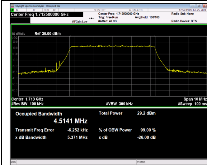
Band66-5MHz-64QAM-132647-25RB#0
