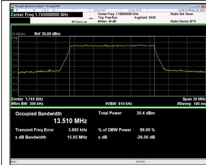
Band66-15MHz-64QAM-132047-75RB#0
