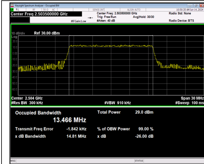
Band41-15MHz-64QAM-41515-75RB#0
