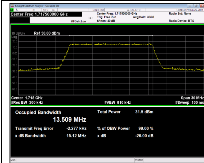
Band66-15MHz-QPSK-132597-75RB#0
