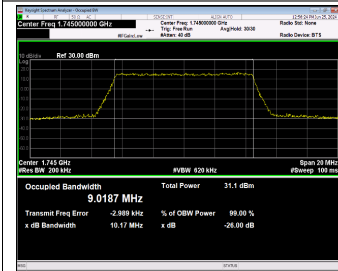
Band66-10MHz-16QAM-132022-50RB#0
