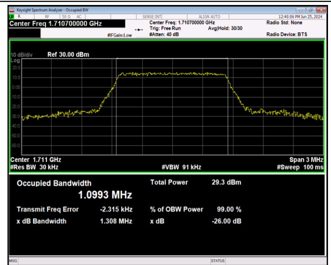
Band66-1.4MHz-16QAM-132665-6RB#0
