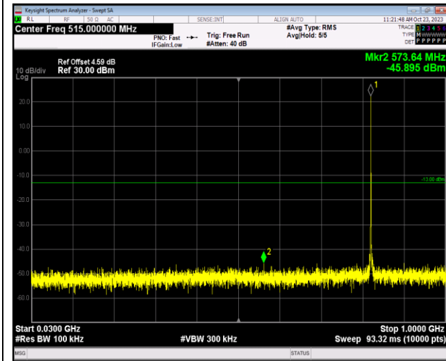
Band26-1.4MHz-QPSK-26915-1RB#0-Range1:30~1000MHz
