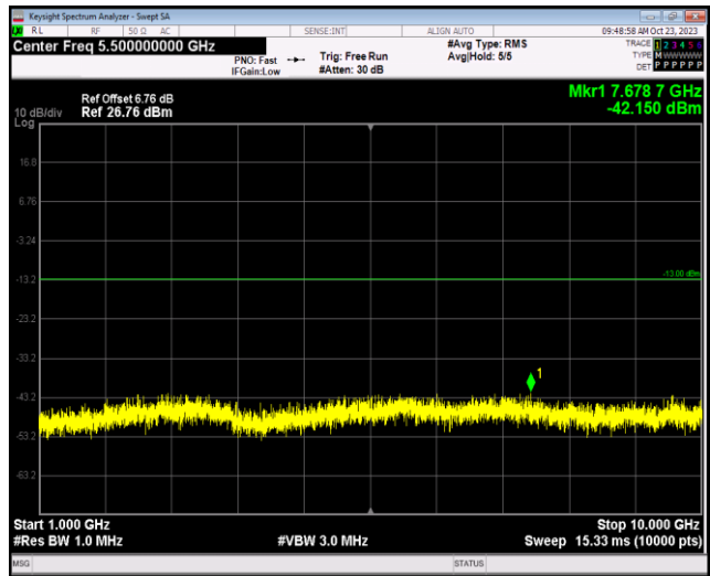
Band13-5MHz-64QAM-23230-1RB#0-Range1:30~1000MHz
