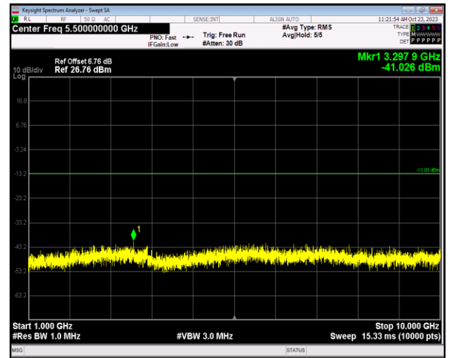
Band26-1.4MHz-QPSK-26915-1RB#0-Range2:1000~10000MHz
