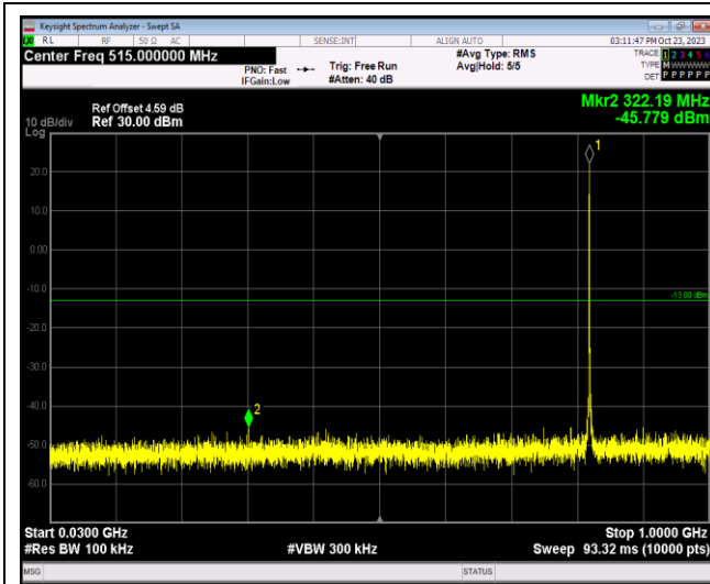
Band26-1.4MHz-QPSK-26797-1RB#0-Range1:30~1000MHz
