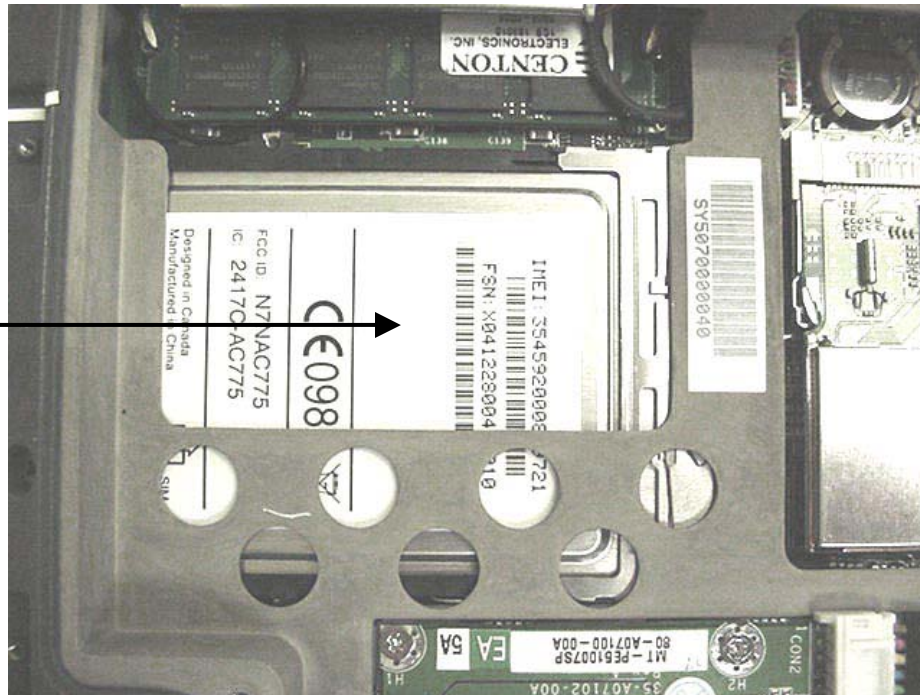
AirCard 775 Installed
