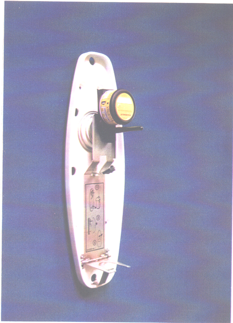
Float Free Enclosure with EPIRB removed (Hammar HRU installed) Figure A3
