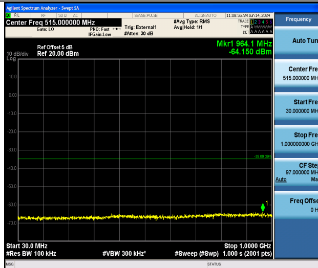
Band41_15MHz_16QAM_39725_1RB#0_30~1000_30~1000
