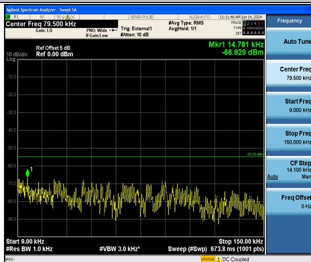
Band41_15MHz_16QAM_40620_1RB#0_0.009~0.15_0.009~0.15
