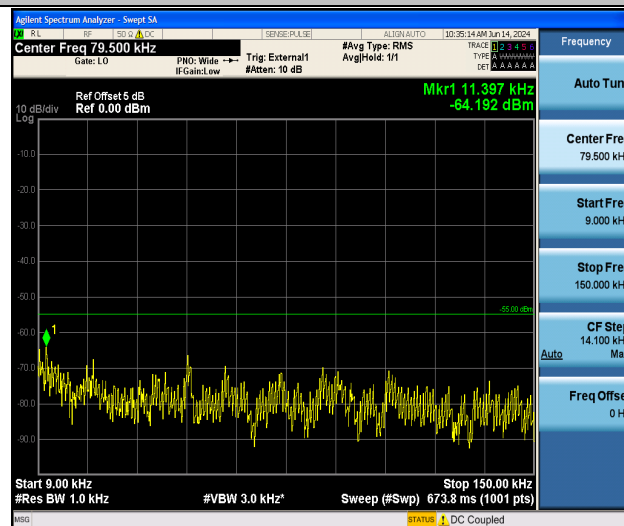
Band41_10MHz_16QAM_39700_1RB#0_0.009~0.15_0.009~0.15
