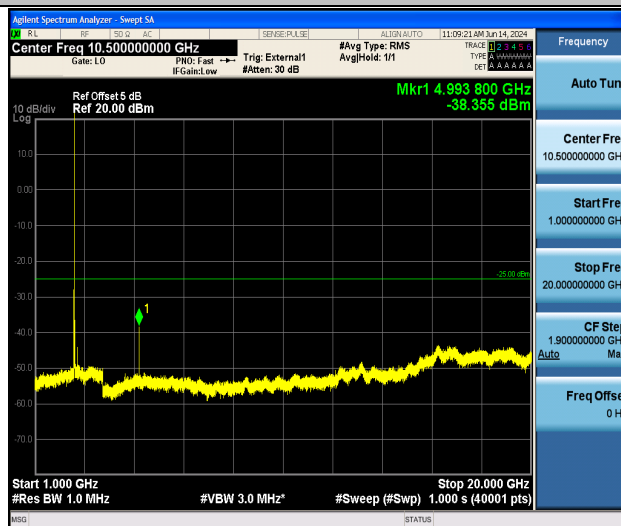
Band41_15MHz_16QAM_39725_1RB#0_1000~20000_1000~20000
