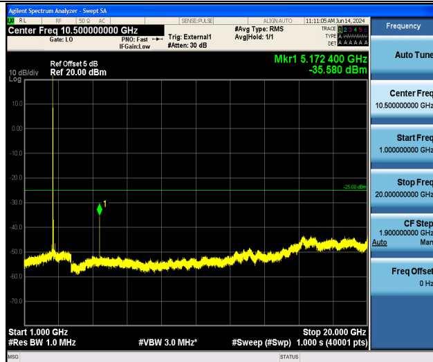
Band41_15MHz_QPSK_40620_1RB#0_1000~20000_1000~20000
