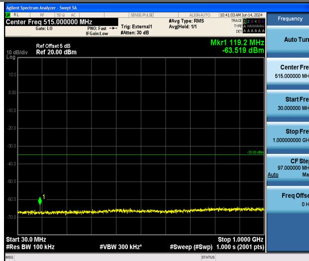
Band41_10MHz_QPSK_41540_1RB#0_30~1000_30~1000
