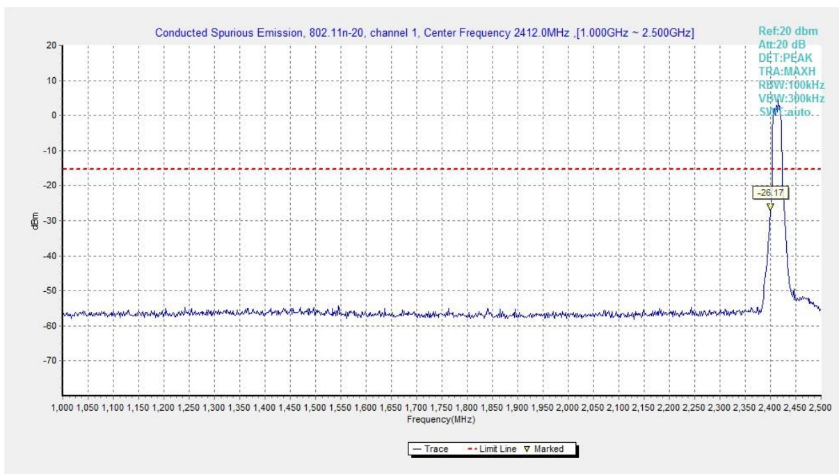
Fig.B.6.1.51 Transmitter Spurious Emission - Conducted (802.11n-HT20, Ch1, 1 GHz-2.5 GHz)
