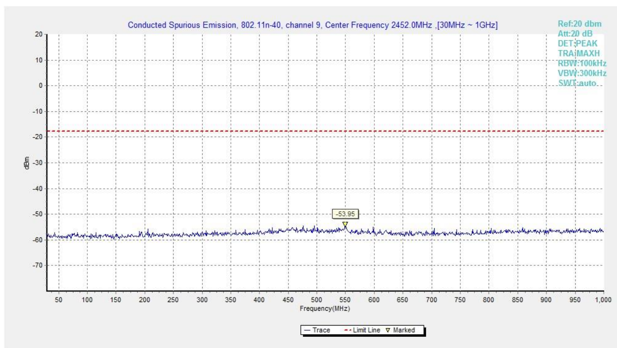
Fig.B.6.1.90 Transmitter Spurious Emission - Conducted (802.11n-HT40, Ch9, 30 MHz-1 GHz)
