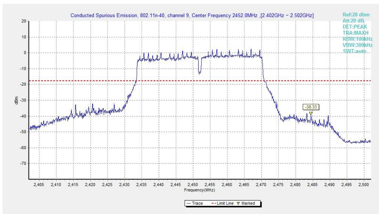
Fig.B.6.1.89 Transmitter Spurious Emission - Conducted (802.11n-HT40, Ch9, Center Frequency)
