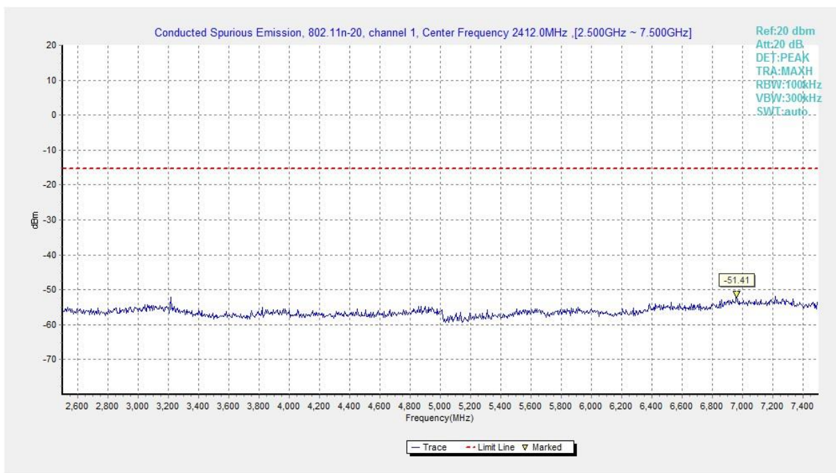
Fig.B.6.1.52 Transmitter Spurious Emission - Conducted (802.11n-HT20, Ch1, 2.5 GHz-7.5 GHz)
