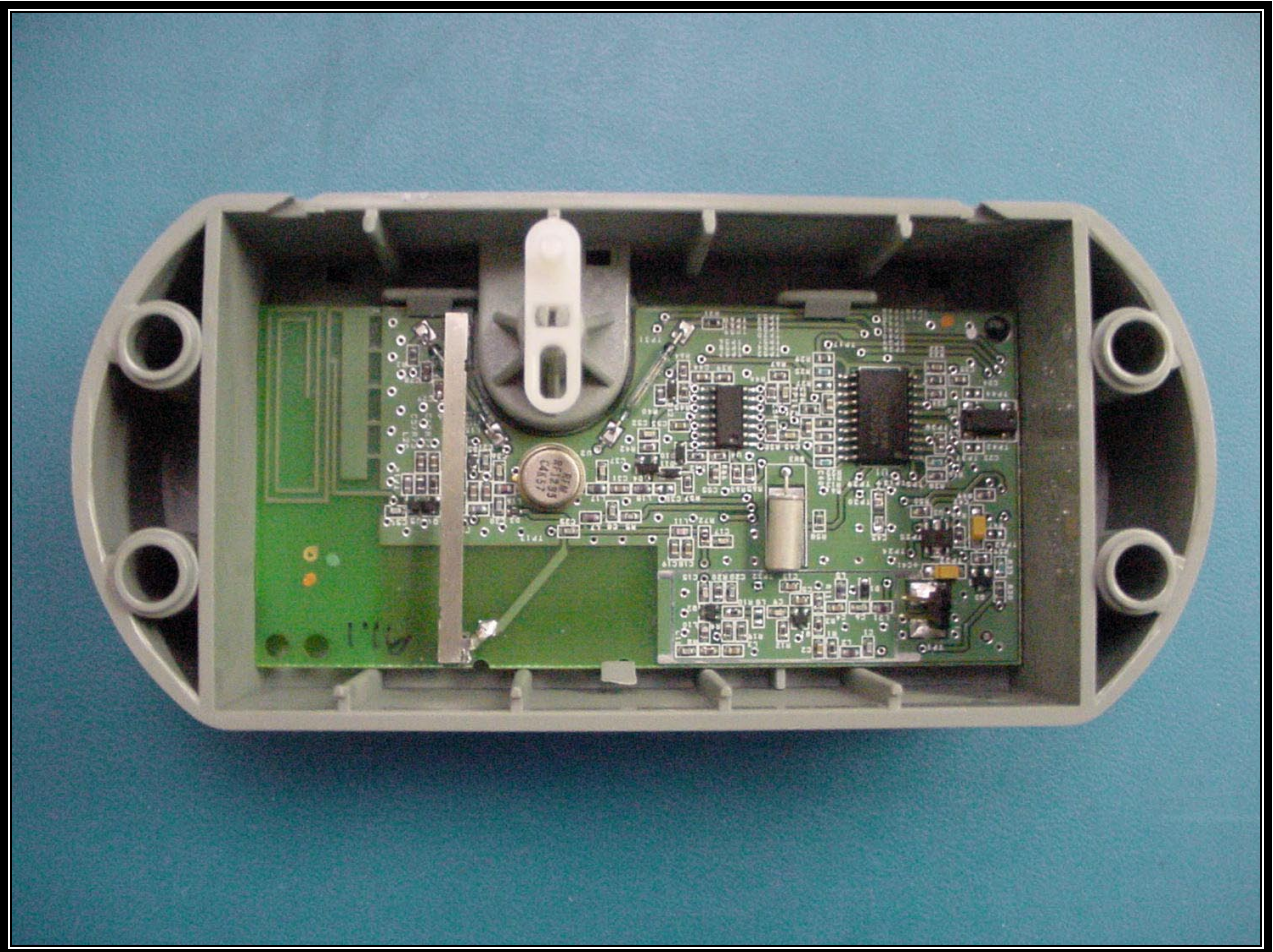
PHOTOGRAPH 5: BACK VIEW OF TRANSPONDER
