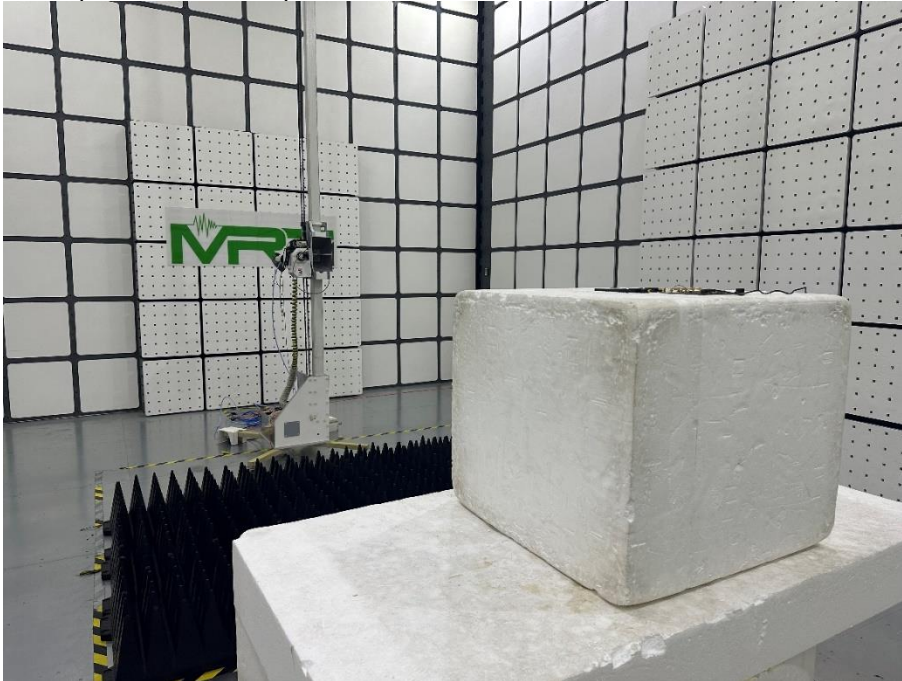
Description: Radiated Spurious Emission Test Setup for 18GHz to 40GHz
