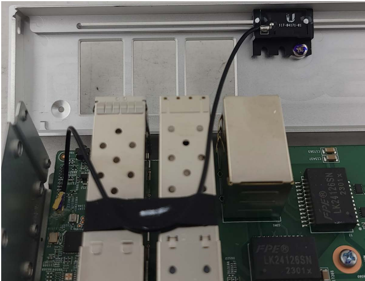
Photograph 1: Internal View of BLE Antenna on Front Panel
