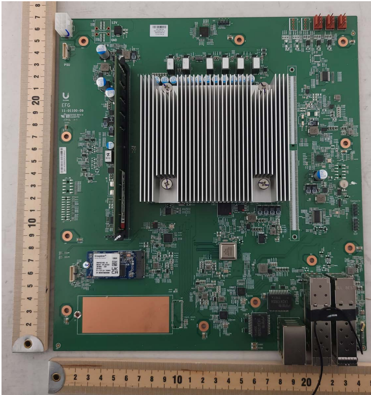
Photograph 2: Top Main PCB
