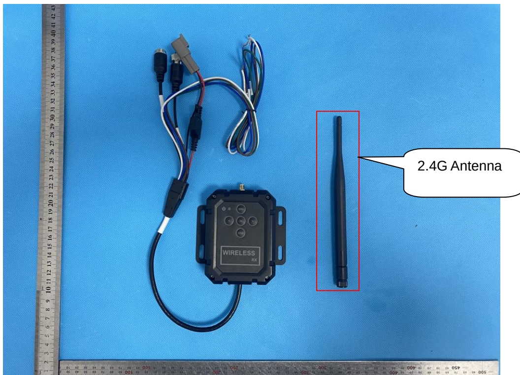
ALL VIEW OF EUT (FIGURE 2)
