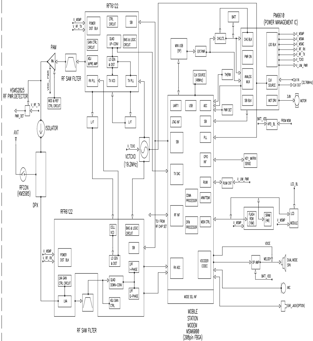
BLOCK DIAGRAM OF VS-500
