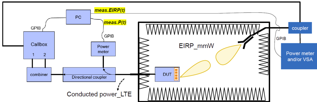
Figure 7-1 mmW NR radiated power measurement setup – Test Setup Photos 12
