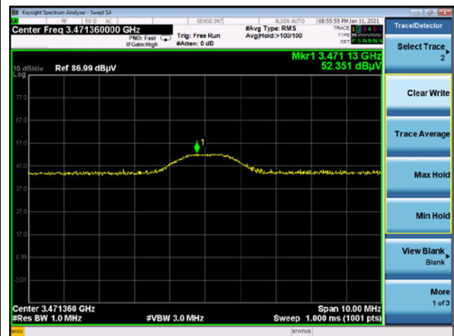
8 th harmonic
