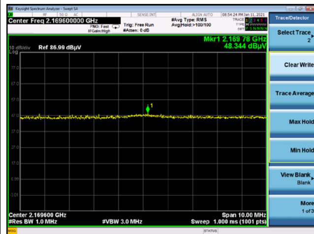
5 th harmonic
