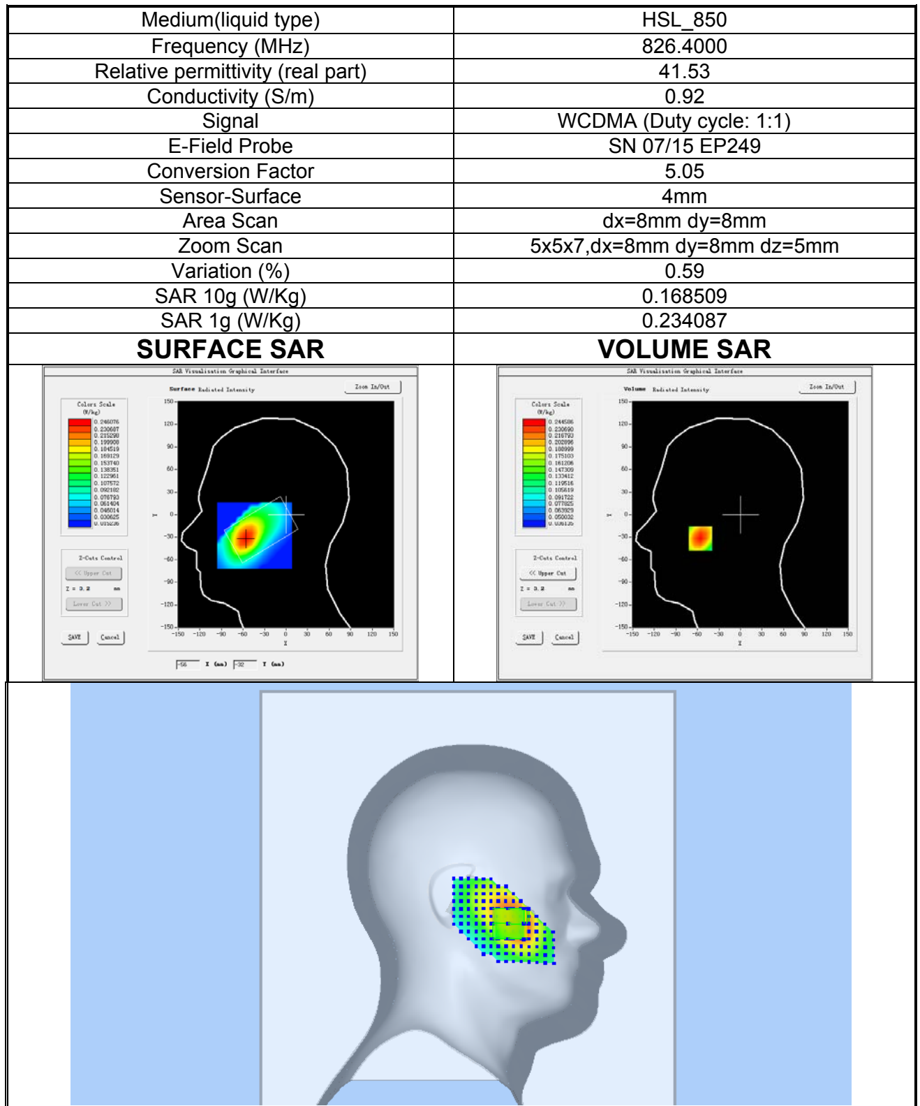
Plot 7: WCDMA BAND V, Low channel (Left Head Cheek) Product Description: Smart Phone Test Date: 2017-08-17
