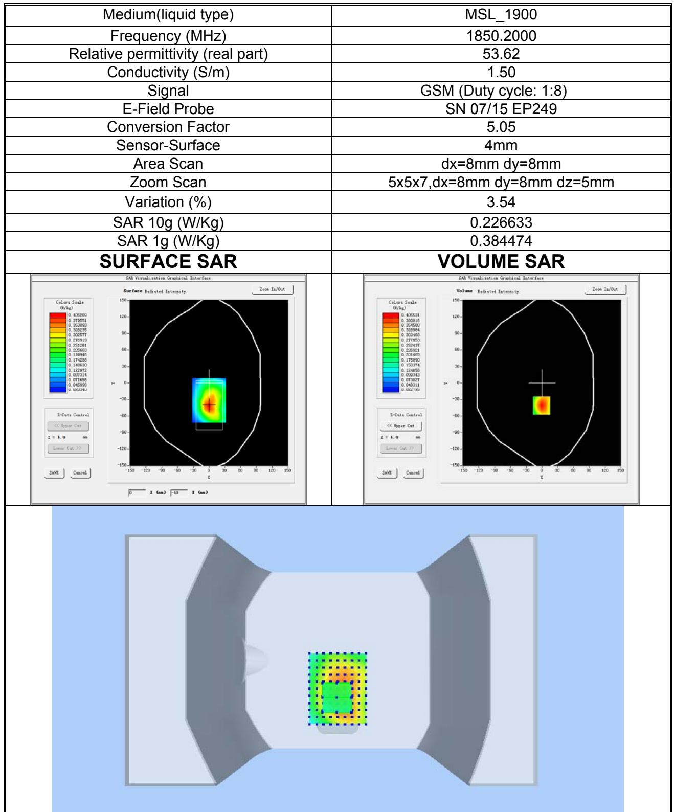
Plot 5: GSM1900, Low channel (Body-worn, Back Surface) Product Description: Smart Phone Test Date: 2017-08-26
