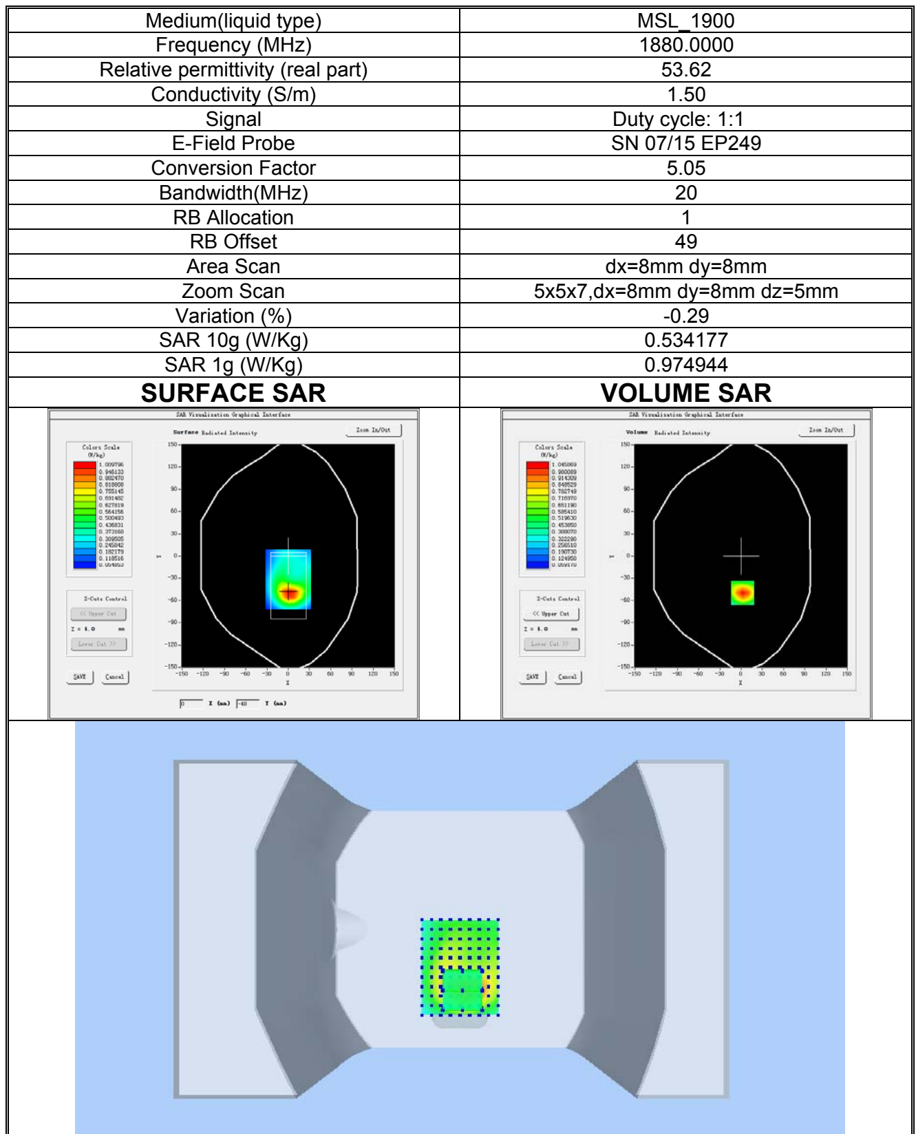
Plot 14:LTE BAND2, Middle channel (Body-worn/Data mode, Back Surface) Product Description:Smart phone Test Date: 2017-08-26
