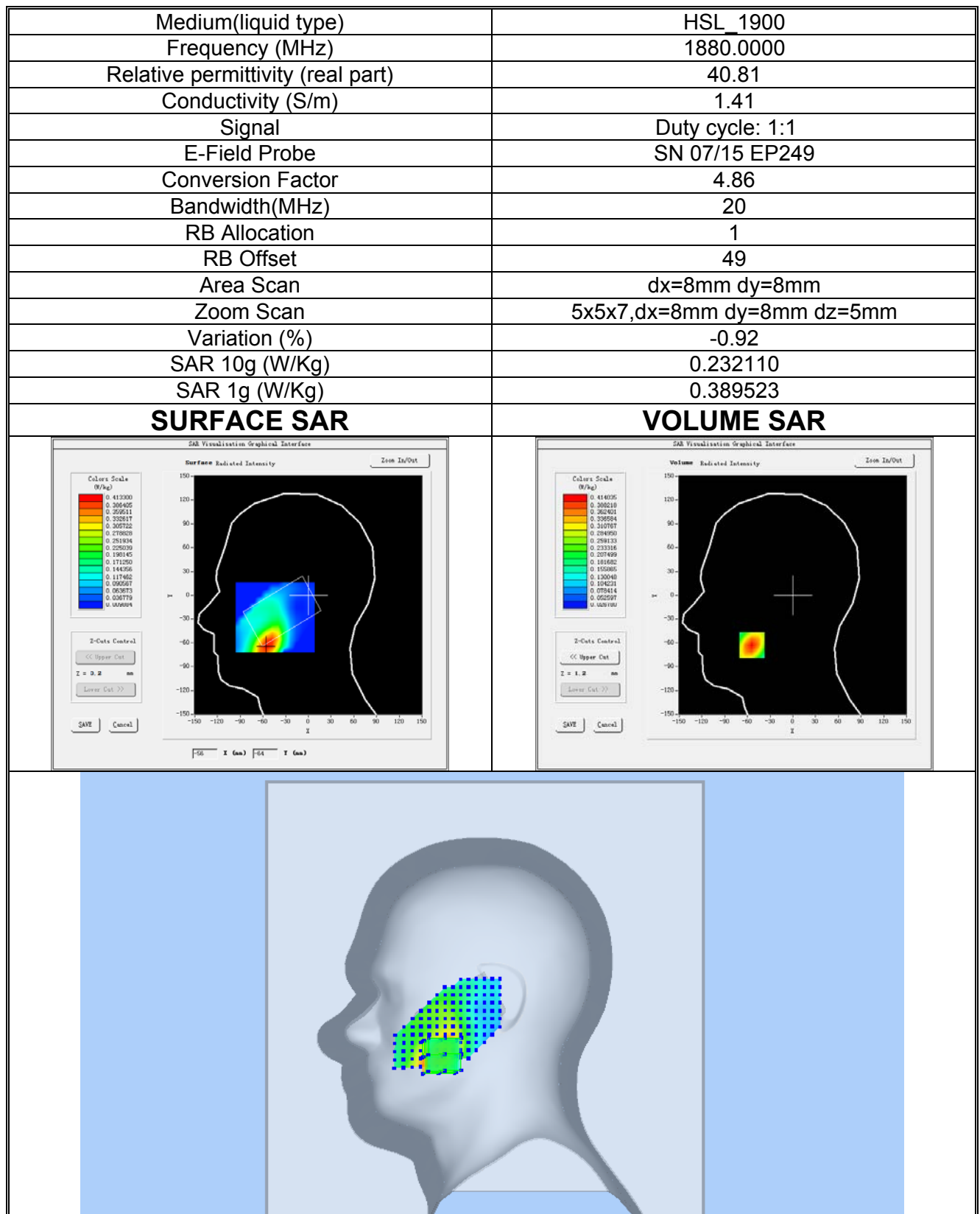
Plot 13:LTE BAND2, Middle channel (Right Head Cheek) Product Description:Smart phone Test Date: 2017-08-26
