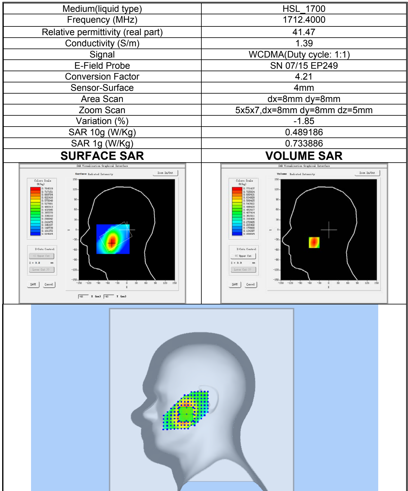
Plot 11: WCDMA BAND IV, Low channel (Right Head Cheek) Product Description: Smart Phone Test Date: 2017-08-26
