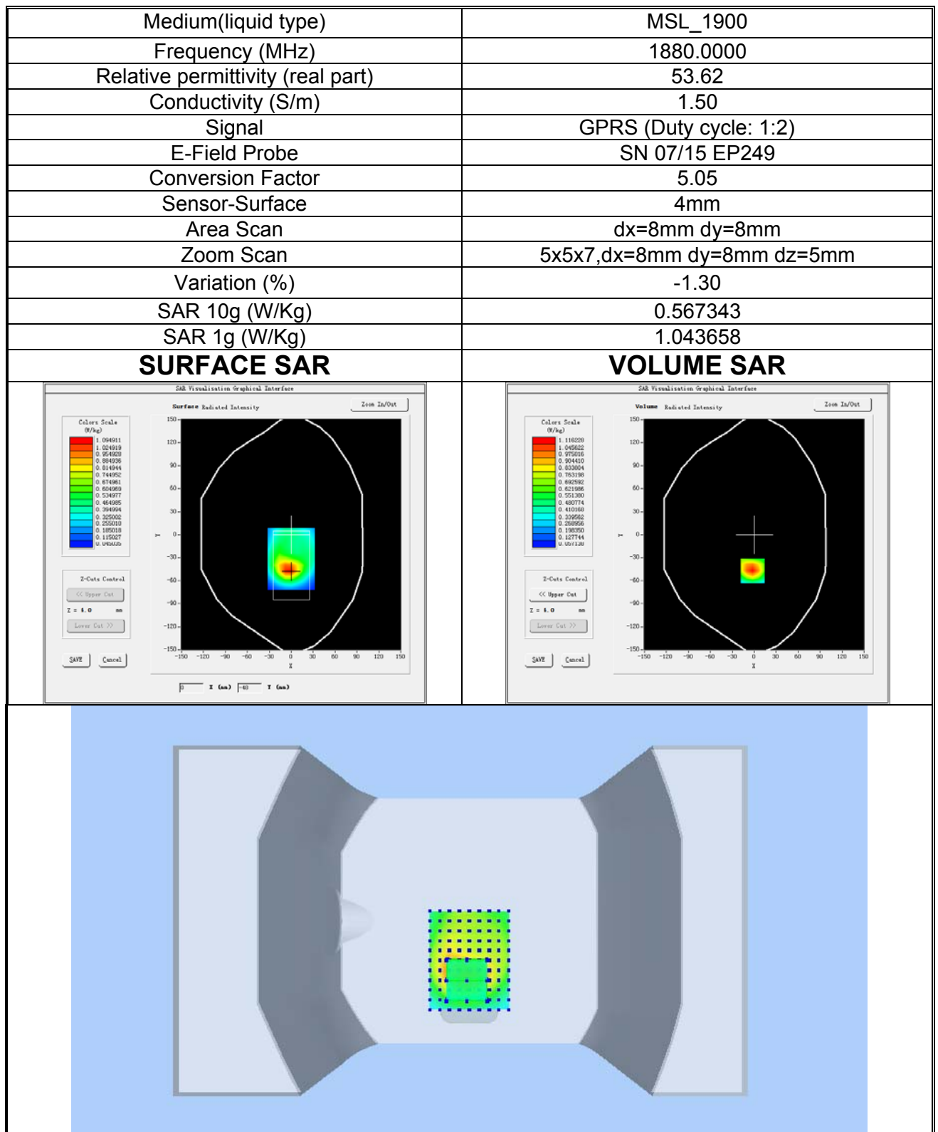
Plot 6: GPRS1900, Middle channel (Data mode, Back Surface) Product Description: Smart Phone Test Date: 2017-08-26
