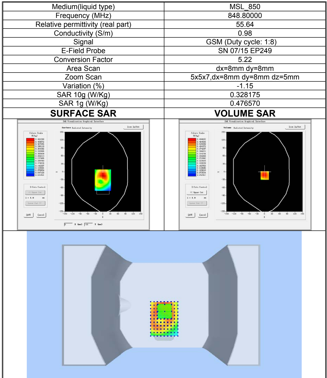
Plot 2: GSM850MHz, High channel (Body-worn, Back Surface) Product Description: Smart Phone Test Date: 2017-08-17
