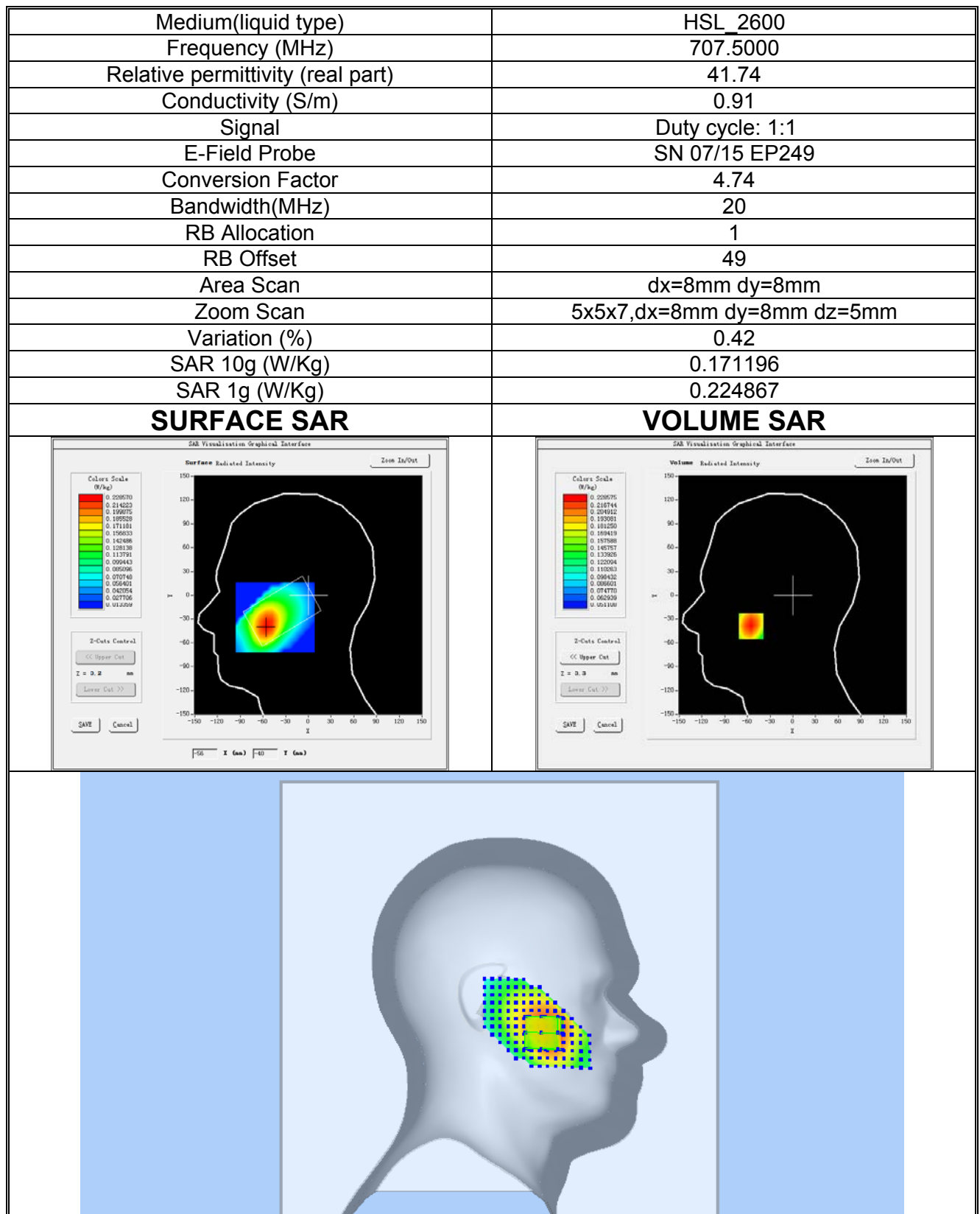
Plot 19:LTE BAND12, Middle channel (Left Head Cheek) Product Description:Smart phone Test Date: 2017-08-22
