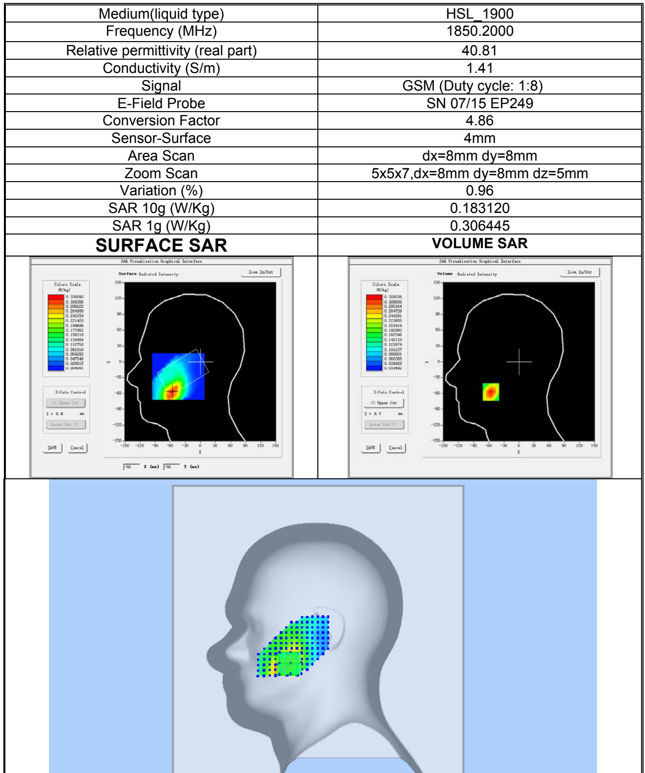
Plot 4: GSM1900, Low channel (Right Head Cheek) Product Description: Smart Phone Test Date: 2017-08-26
