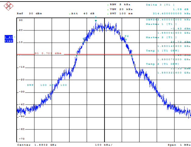
GPRS 1900
