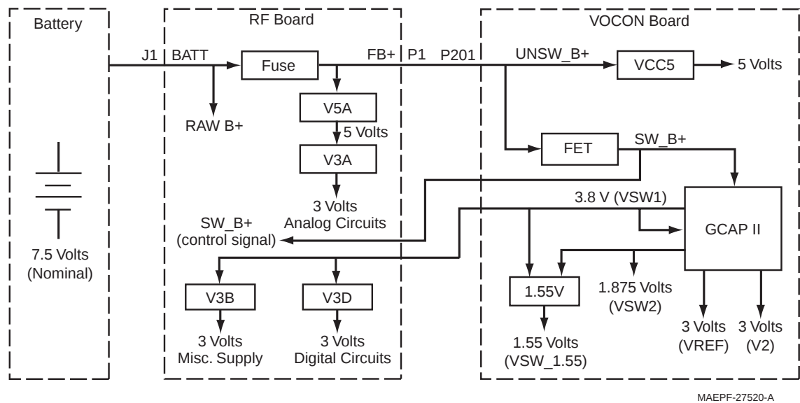
Figure 2-2. DC Power Distribution—VHF Radios
