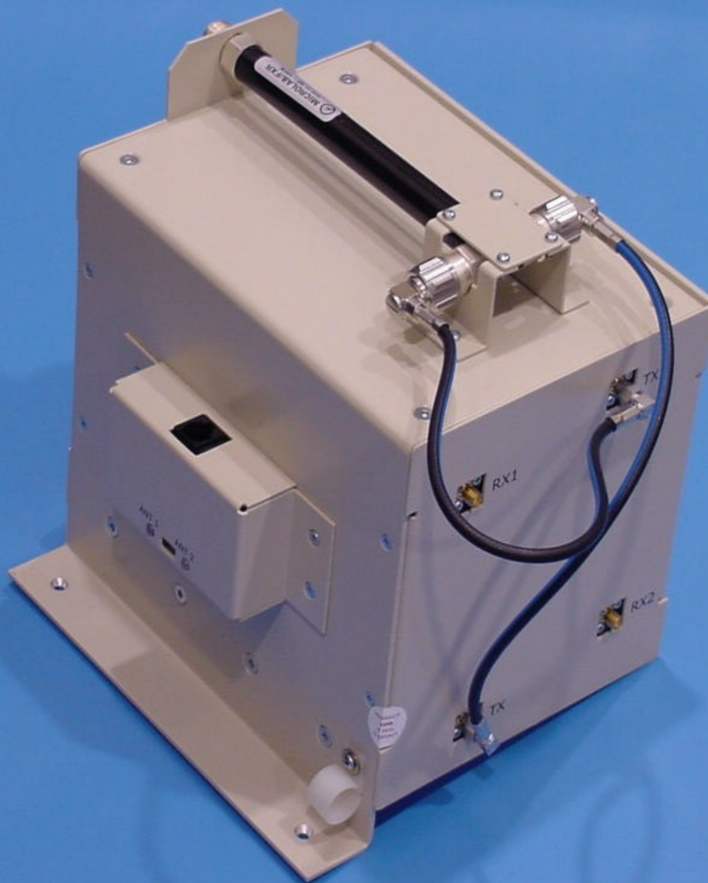
Digivance LRCS SMR Dual Transmit Duplexer Detail 2
