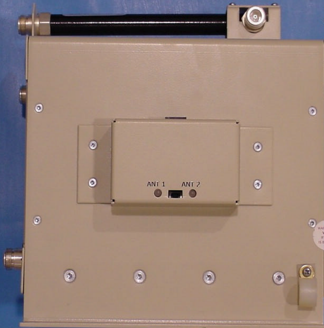
Digivance LRCS SMR Dual Transmit Duplexer Right View
