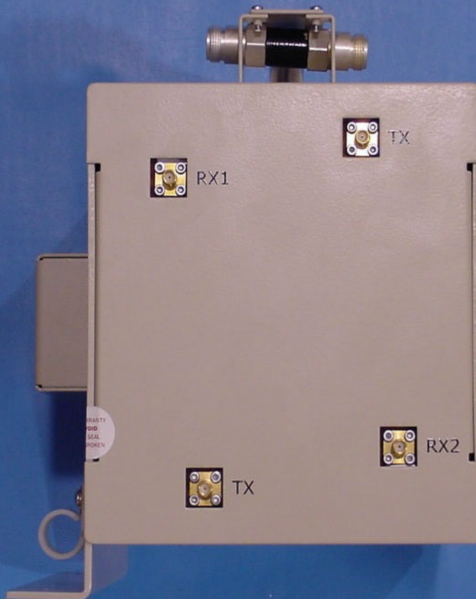
Digivance LRCS SMR Dual Transmit Duplexer Rear View
