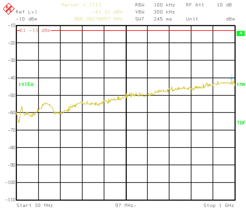
30MHz-1GHz – V Pol
