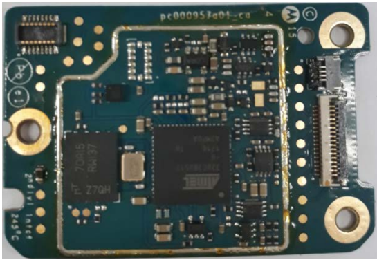
GOB board without shields (Top)
