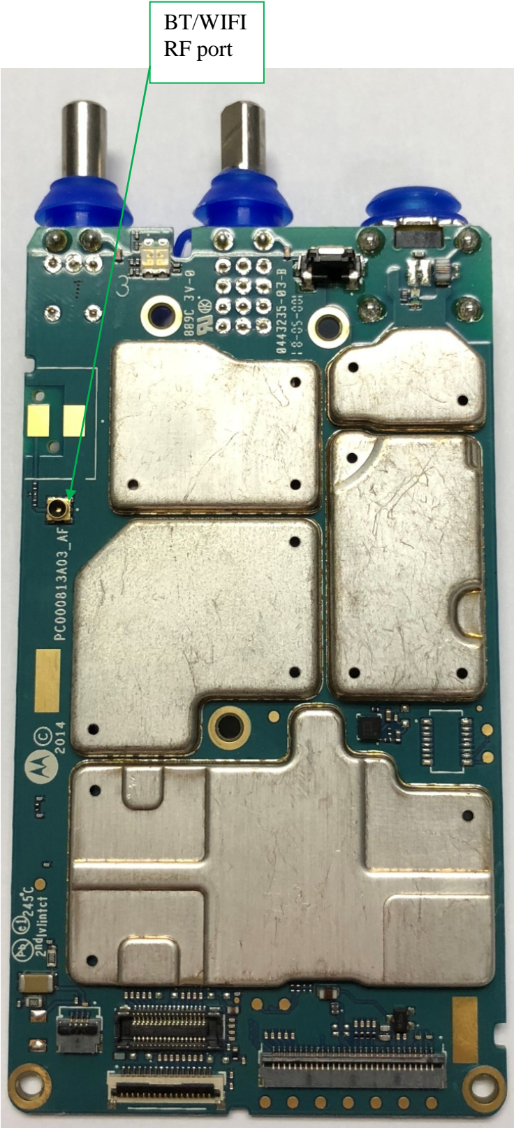
RF board with Shields (Top)
